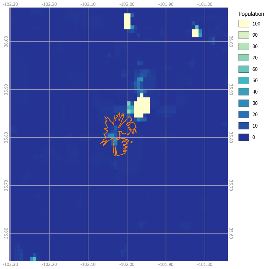
Figure 3. PFD Contour Projected Onto GPWv4 Population Grid
