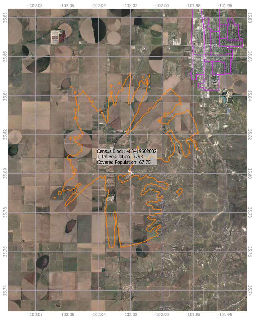
Figure 1. PFD Contours for Dumas Gateway
