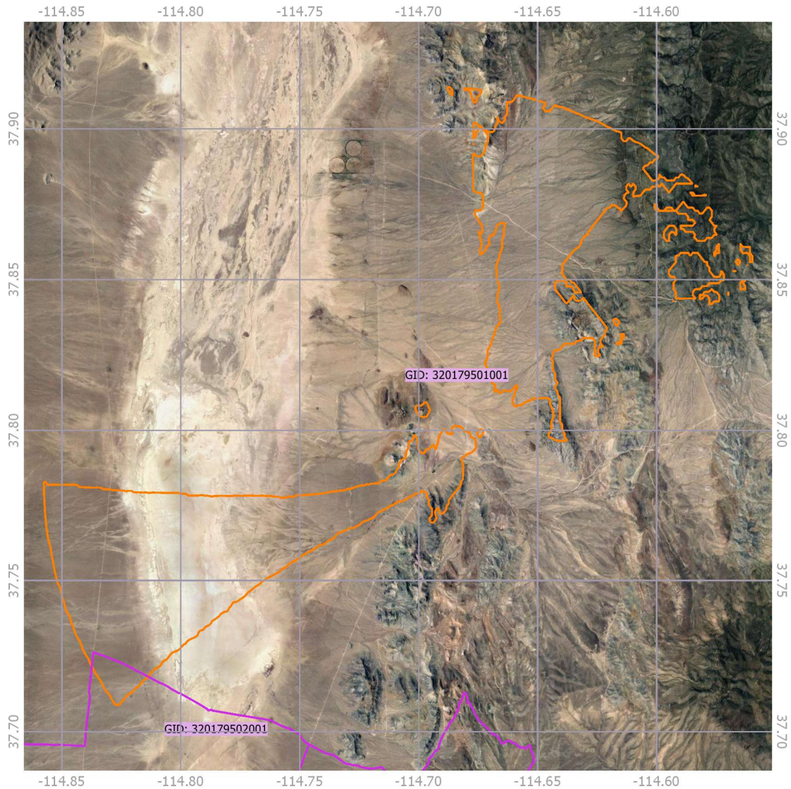
Figure 1. PFD Contours for Panaca Gateway
