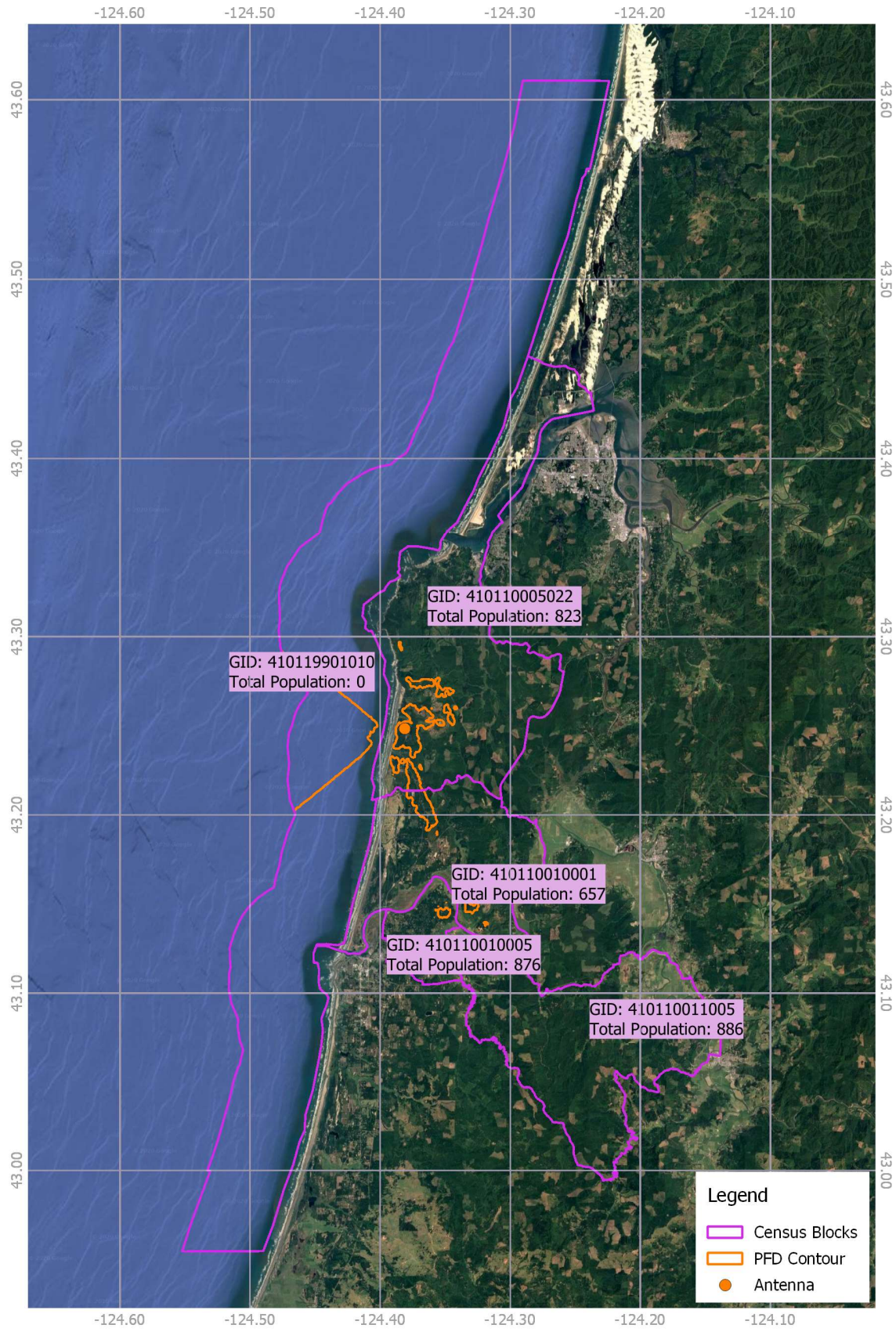
Figure 1. PFD Contours for Charleston Gateway
