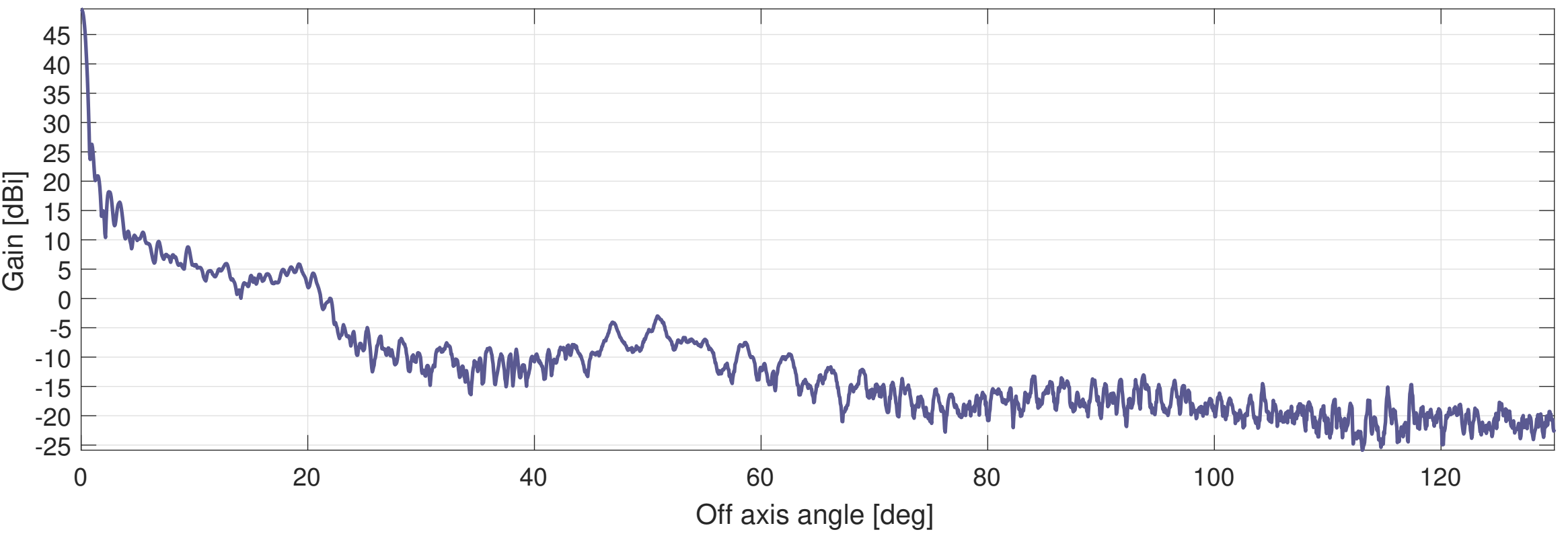
SpaceX (Co-pol) 1.47 Meter Gain
