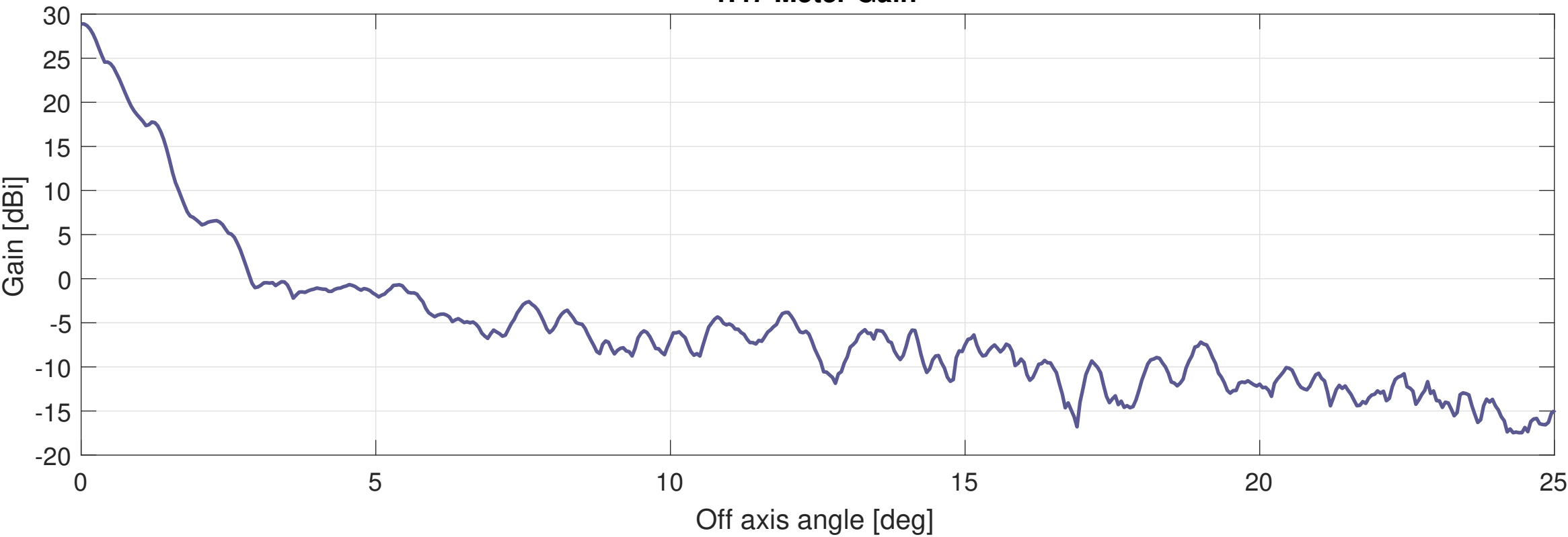
SpaceX (Cross-pol) 1.47 Meter Gain
