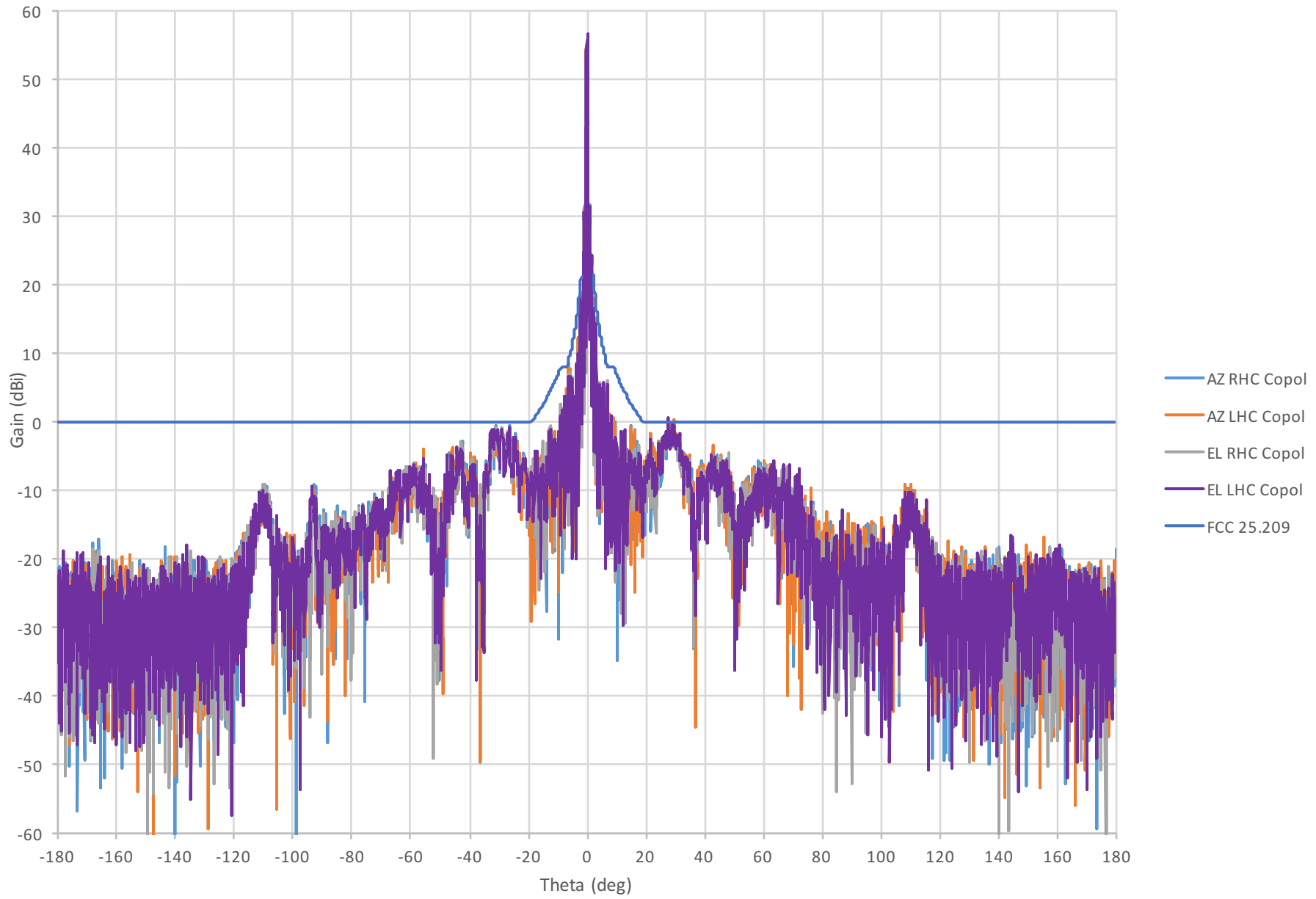
19.2 GHz Gain
