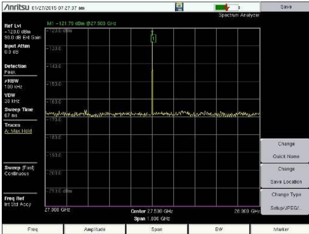
Figure 2.1-2 (E) Calibration Spectrum Photo 27.5 GHz
