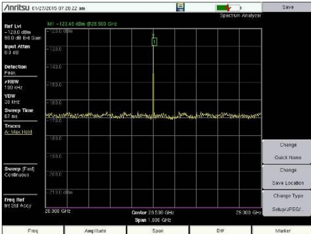
Figure 2.1-2 (F) Calibration Spectrum Photo 28.5 GHz
