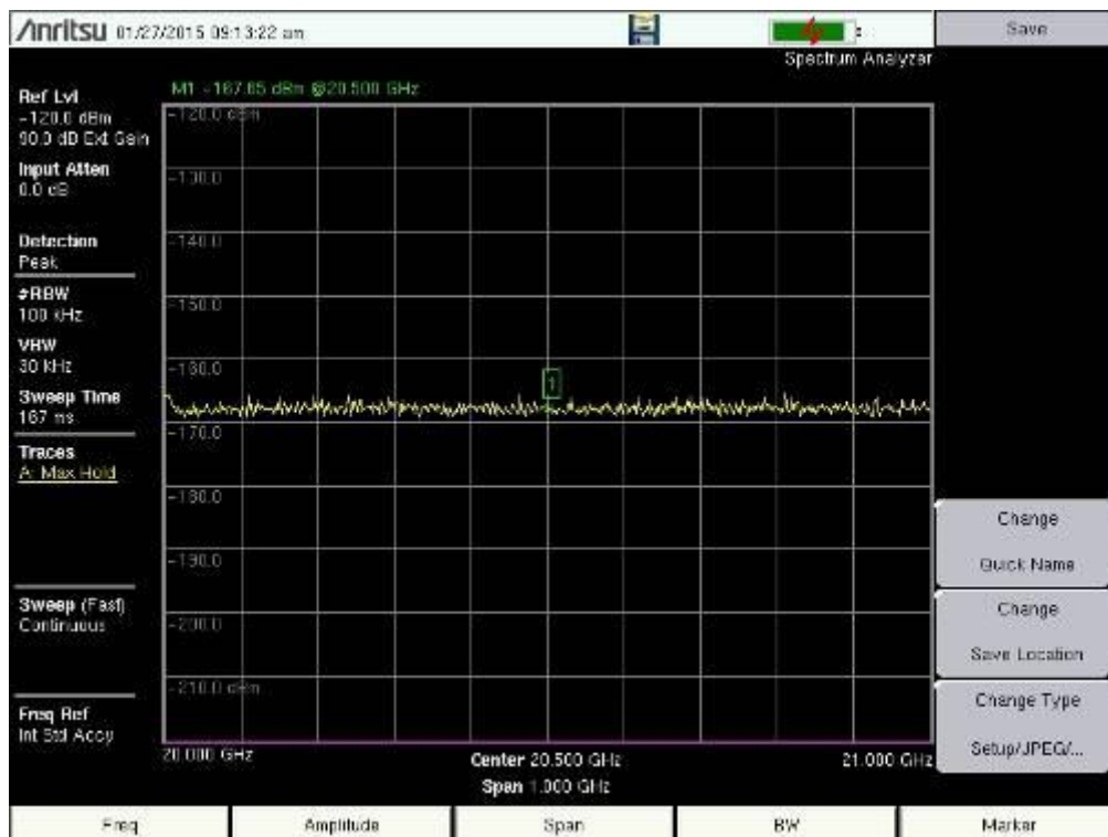
Figure 3.1-6 (B) Spectrum Photos 20-21 GHz 100 KHz Res BW Horizontal Pol 360 0
