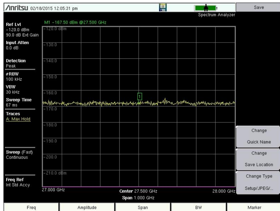
Figure 3.1-7 (B) Spectrum Photos 27-28 GHz 100 kHz Res BW Horizontal Pol 360°
