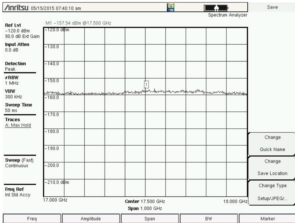
Figure 3.1-3 (C) Spectrum Photos 17-18 GHz 1 MHz Res BW Horizontal Pol Worst
