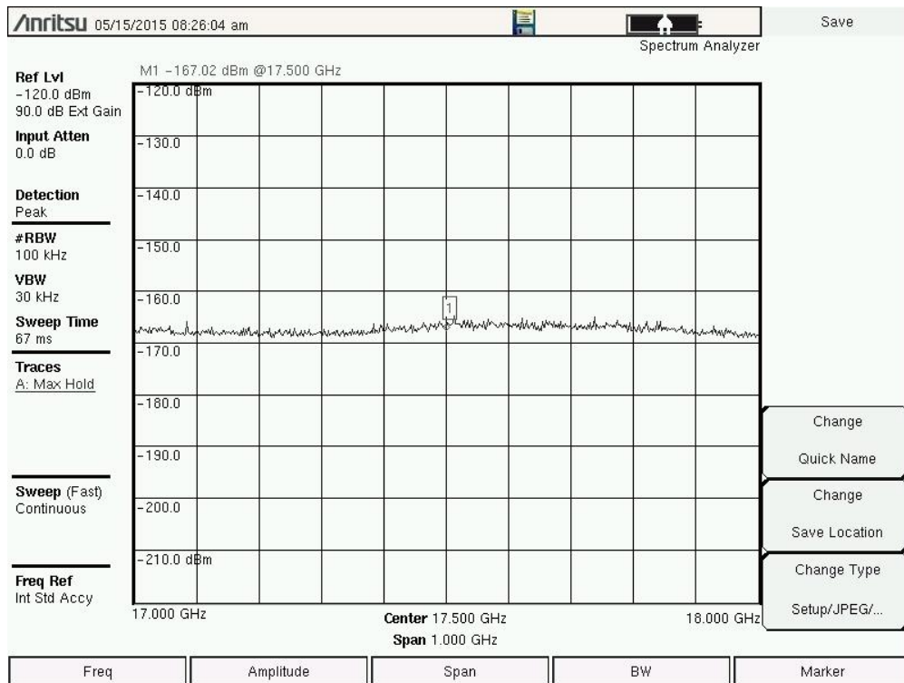
Figure 3.1-3 (H) Spectrum Photos 17-18 GHz 100 kHz Res BW Vertical Pol Worst
