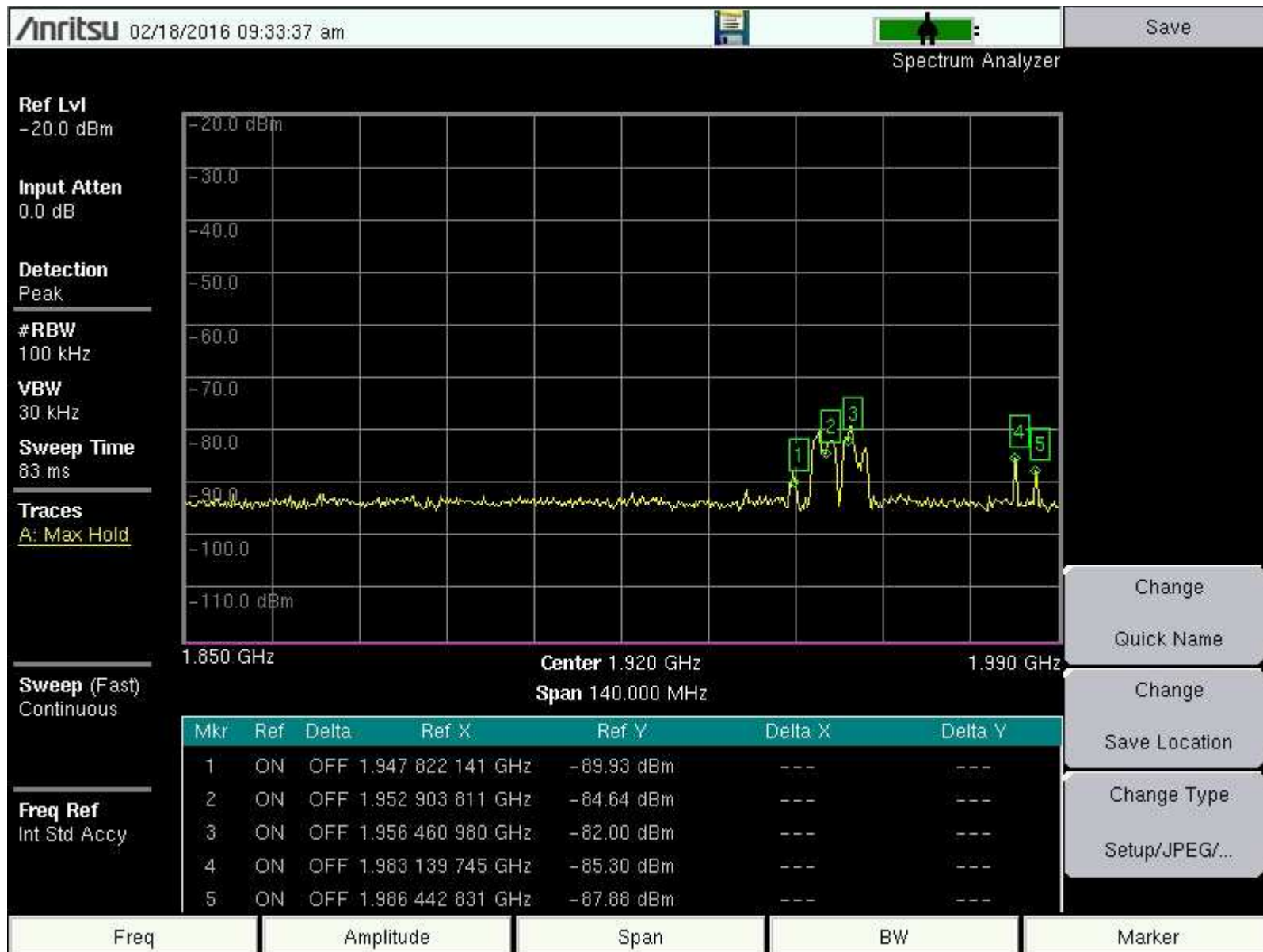
Figure Four – 1850-1990 MHz
