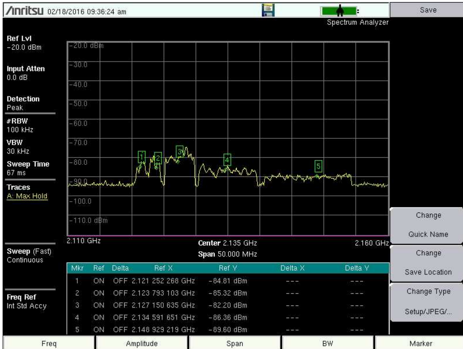
Figure Four – 2110-2160 MHz
