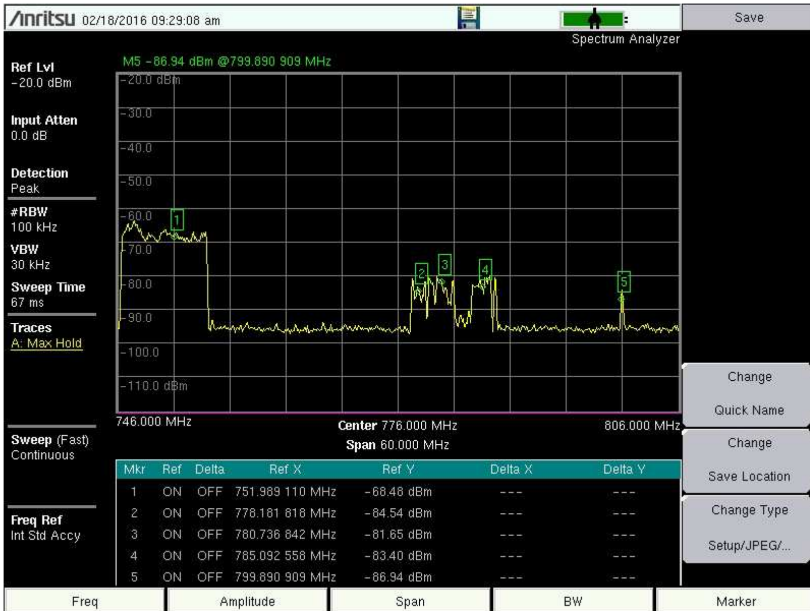
Figure Two – 746 -806 MHz
