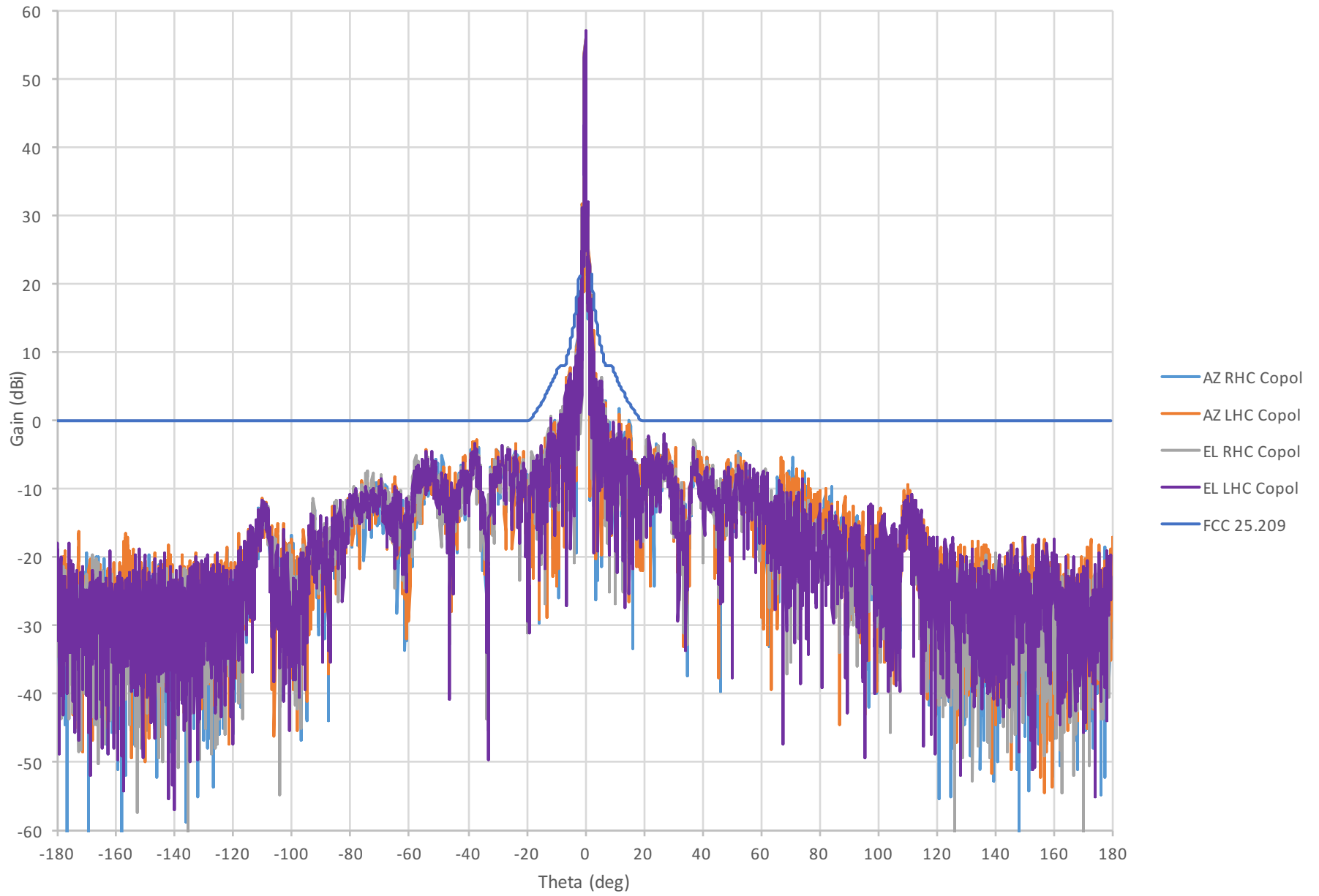
20.2 GHz Gain
