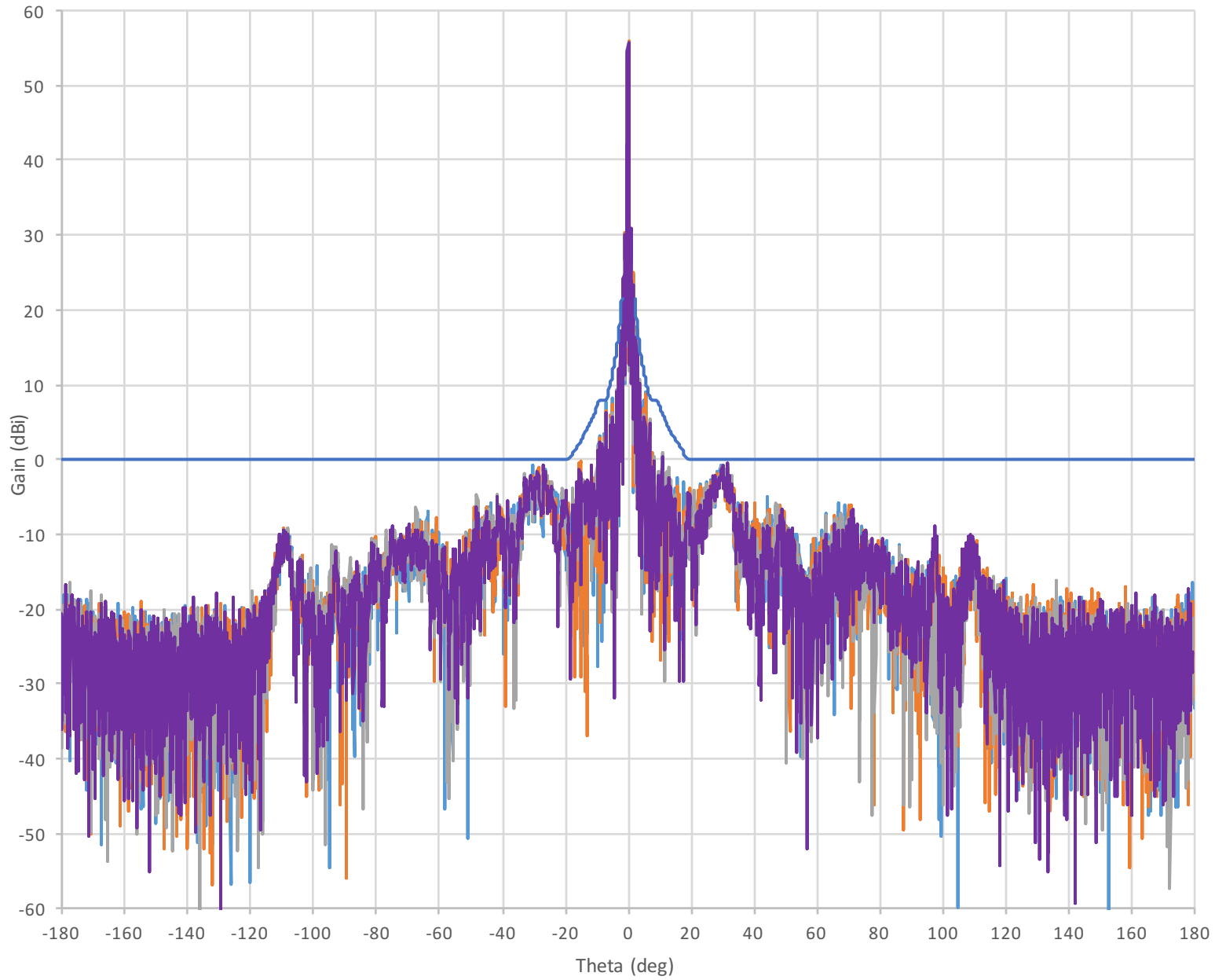
17.7 GHz Gain
