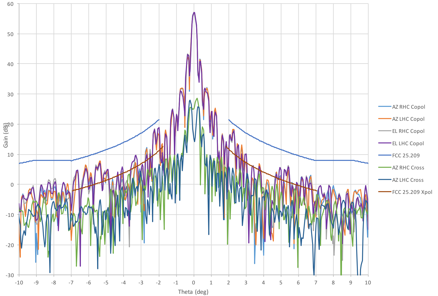
20.2 GHz Gain
