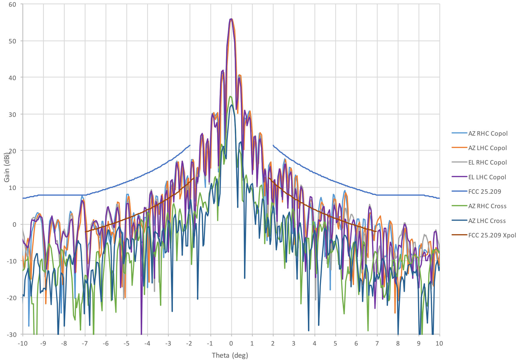
17.7 GHz Gain
