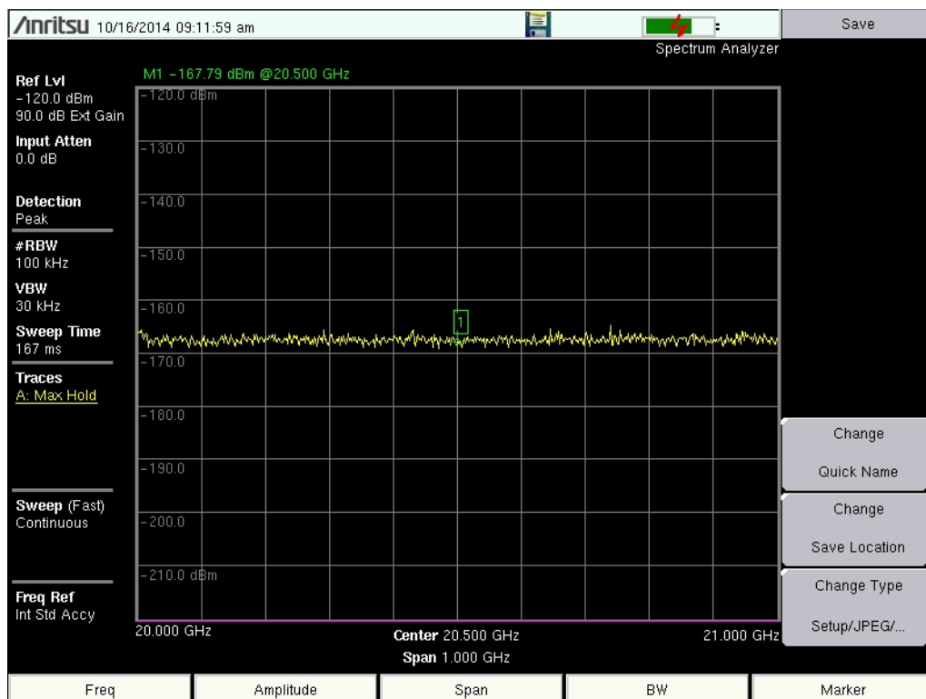
Figure 3.1-6 (F) Spectrum Photos 20-21 GHz 100 KHz Res BW Vertical Pol 360 0
