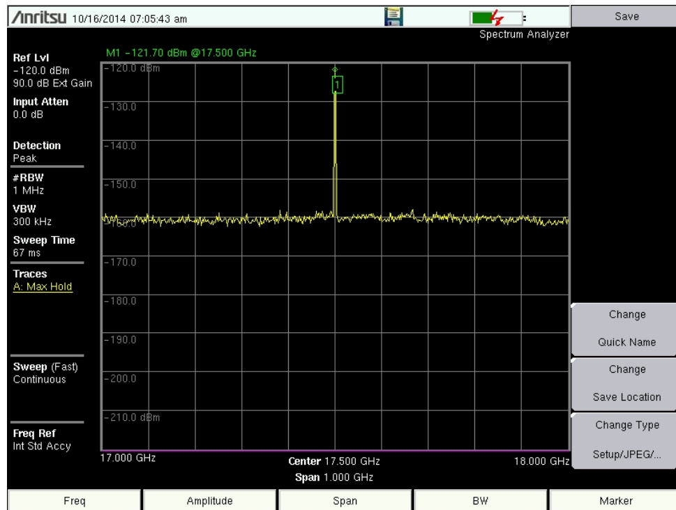
Figure 2.1-2 (A) Calibration Spectrum Photo 17.5 GHz
