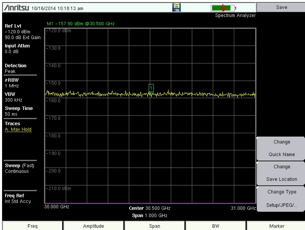
Figure 3.1-10 (C) Spectrum Photos 30-31 GHz 1 MHz Res BW Vertical Pol 360°
