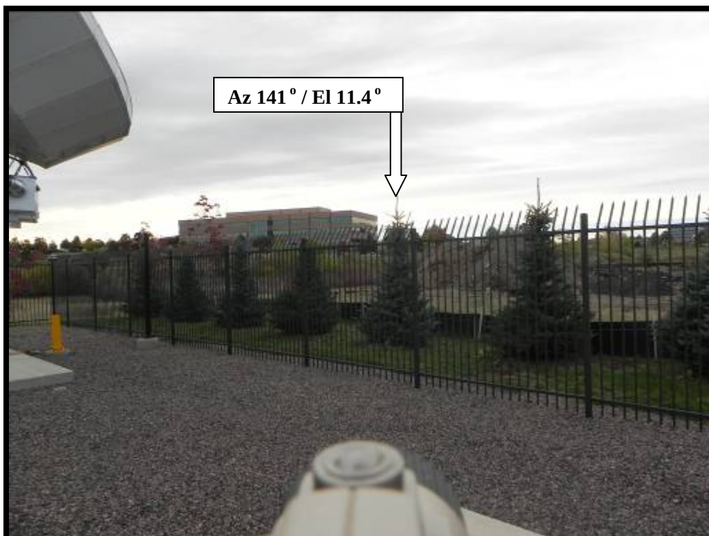
Figure 3.1-2 Horizon Photographs of Earth Station Site
