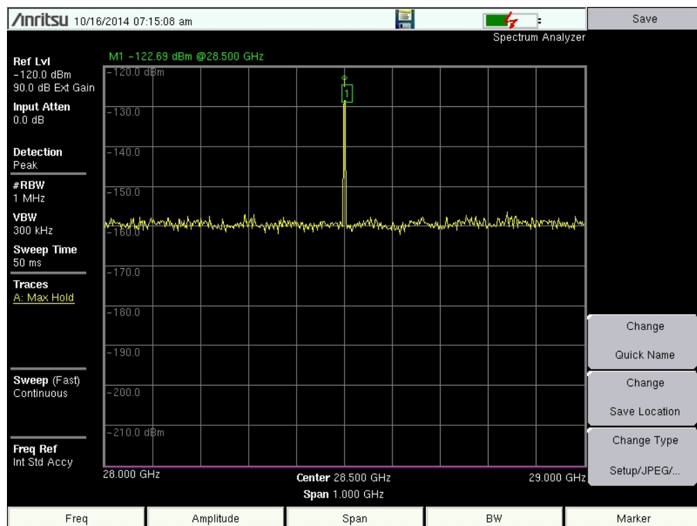
Figure 2.1-2 (F) Calibration Spectrum Photo 28.5 GHz
