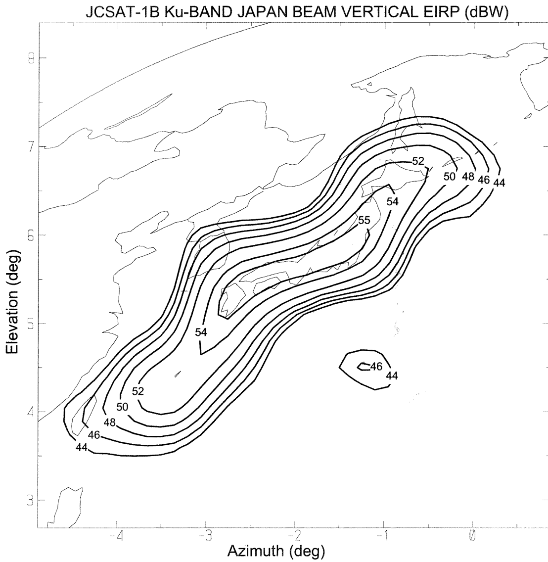
Figure 2.2(b) JCSAT-1B Ku-Band Japan Beam Vertical EIRP
