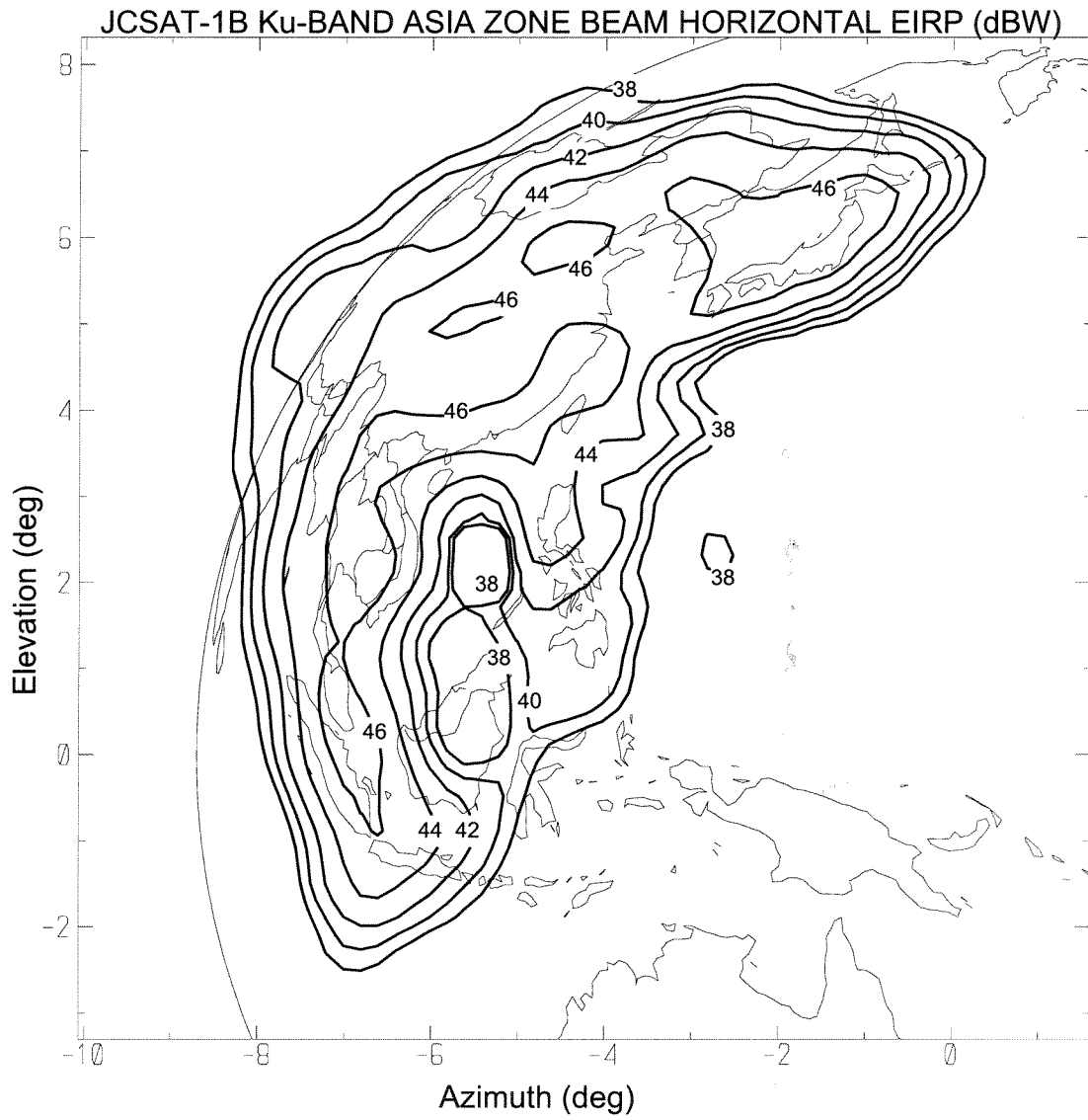
Figure 2.4(d) JCSAT-1B Ku-Band Asia Zone Beam Horizontal EIRP
