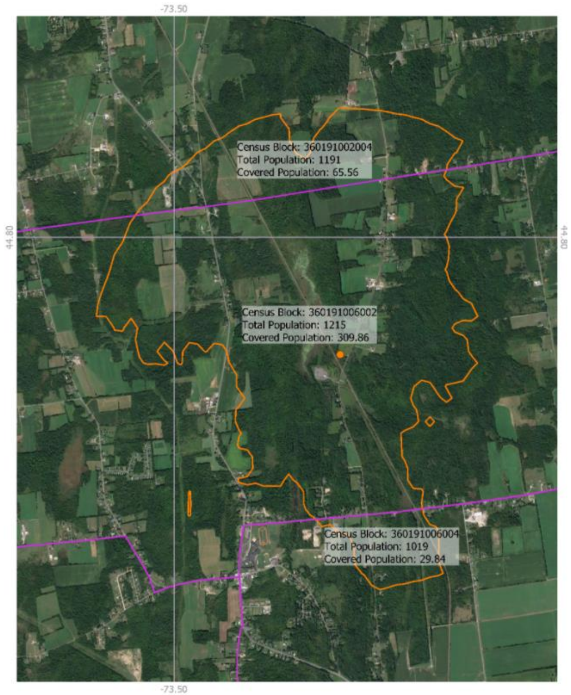
Figure 1. PFD Contours for Beekmantown Gateway
