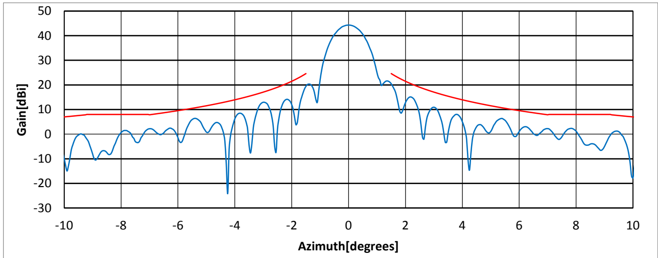
Figure 51 - Plot for 20.2 GHz
