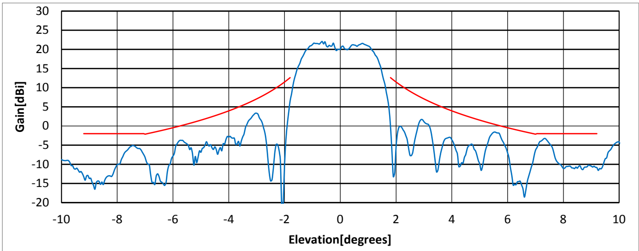
Figure 58 - Plot for 19.7 GHz
