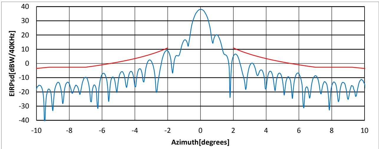
Figure 34 - Plot for 29.5 GHz
