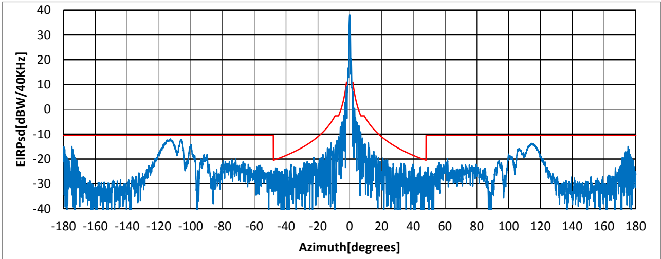
Figure 33 - Plot for 30.0 GHz
