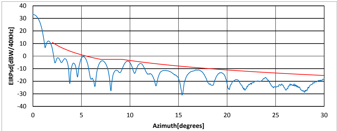
Figure 7 - Plot for 29.5 GHz
