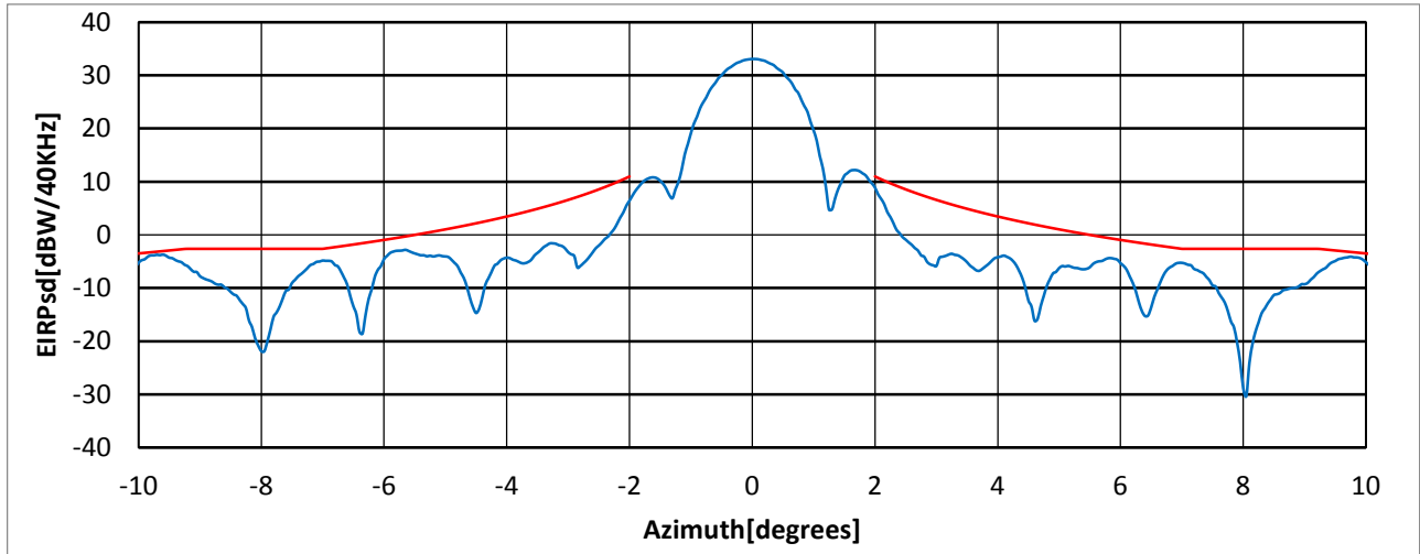
Figure 5 - Plot for 29.75 GHz
