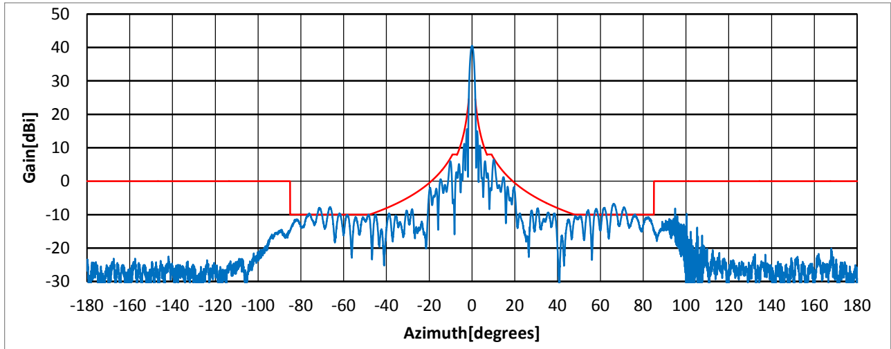
Figure 17 - Plot for 19.95 GHz
