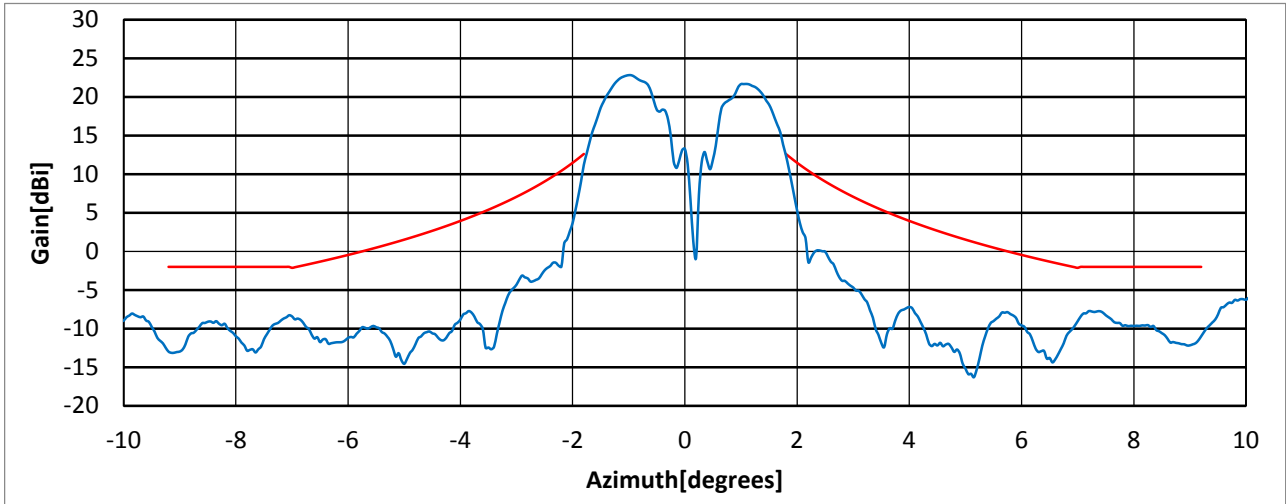
Figure 57 - Plot for 20.2 GHz
