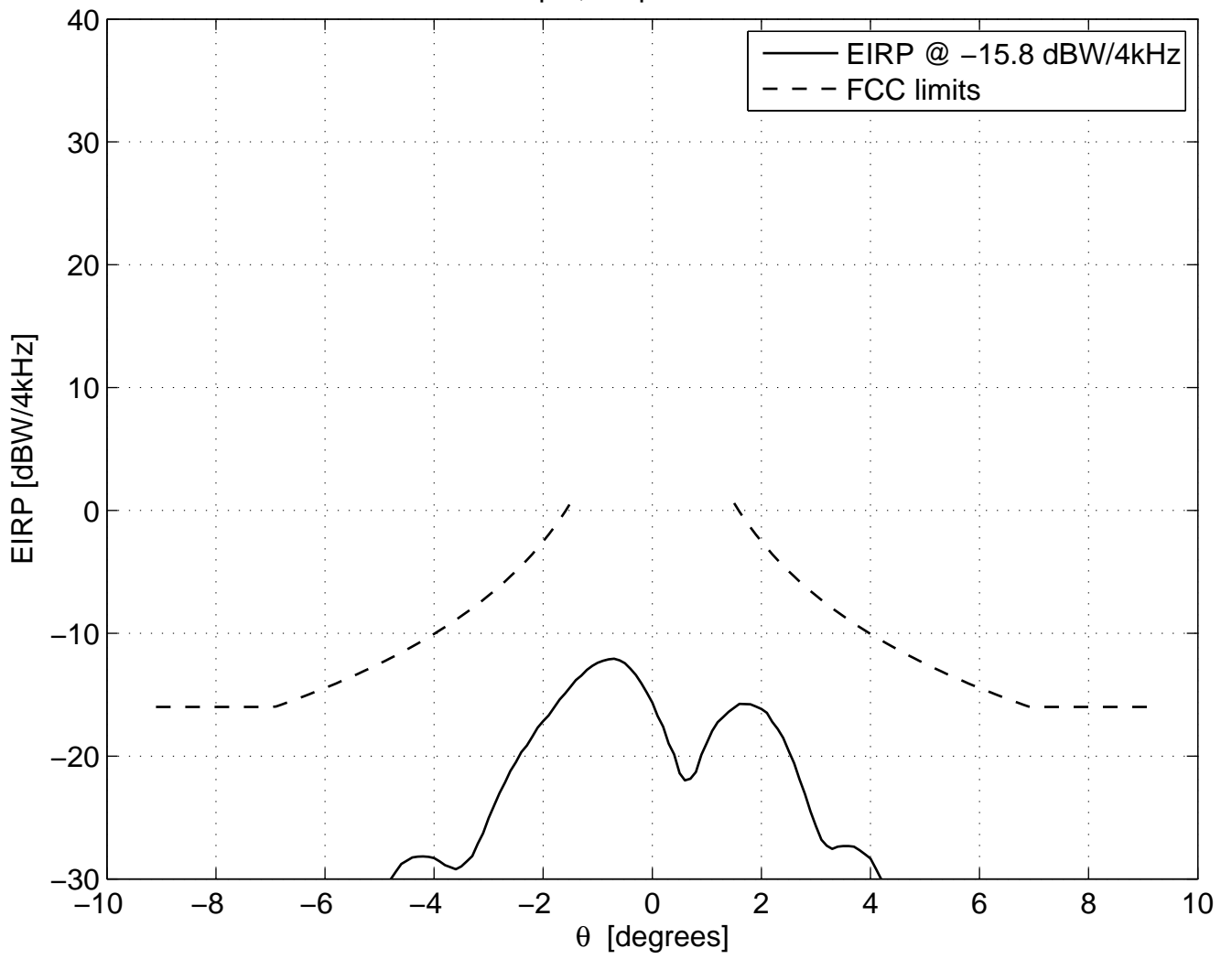
X-pol, freq=14.25 GHz
