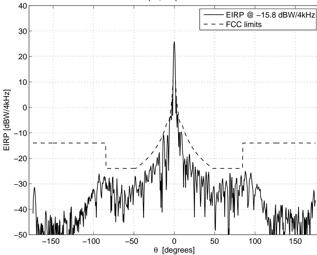
Co-pol, freq=14.5 GHz
