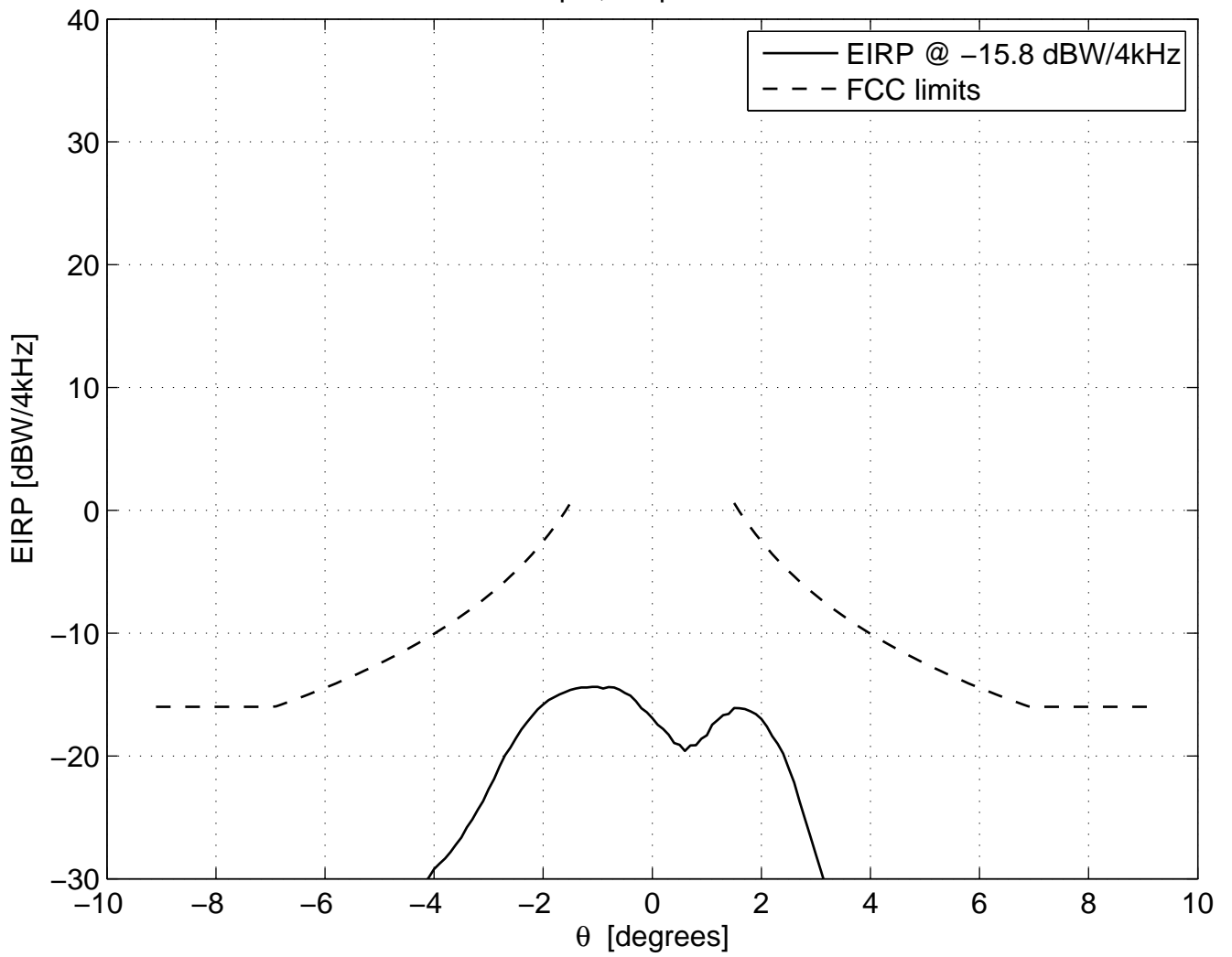
X-pol, freq=14 GHz
