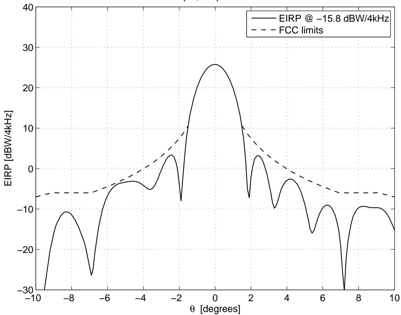
Co-pol, freq=14.5 GHz
