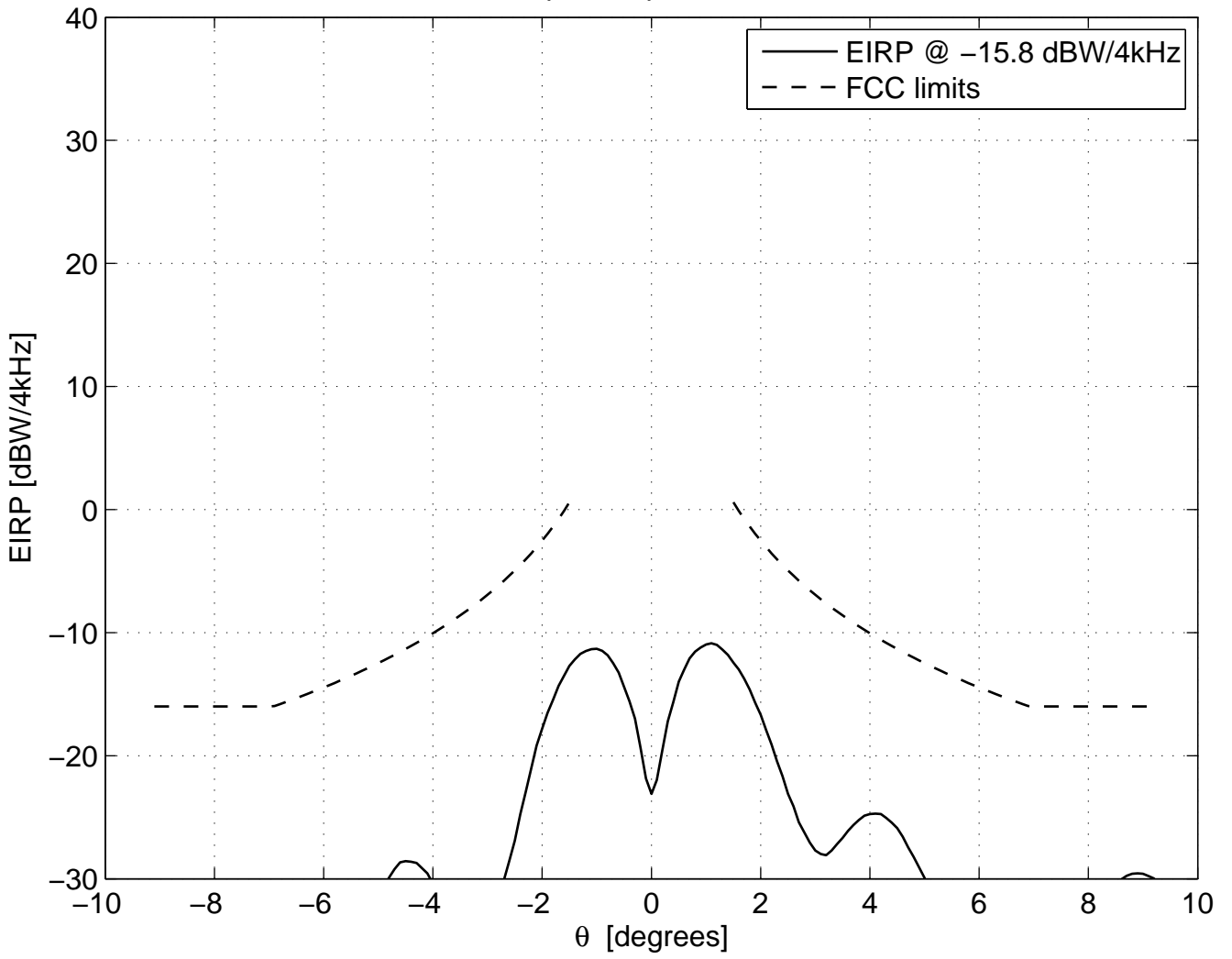
X-pol, freq=14.5 GHz
