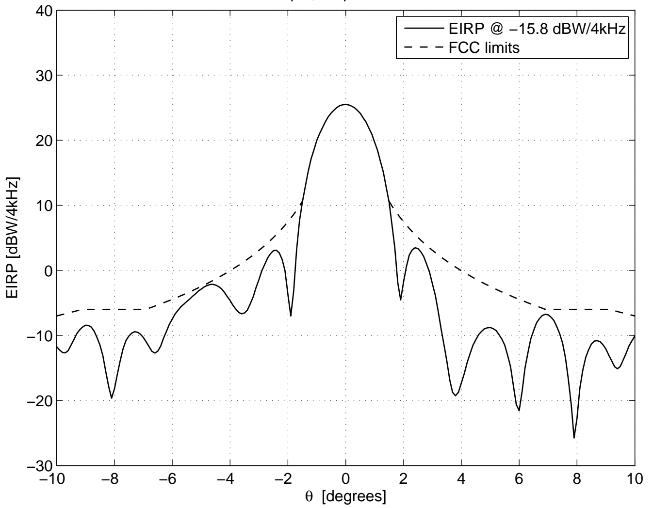
Co-pol, freq=13.75 GHz
