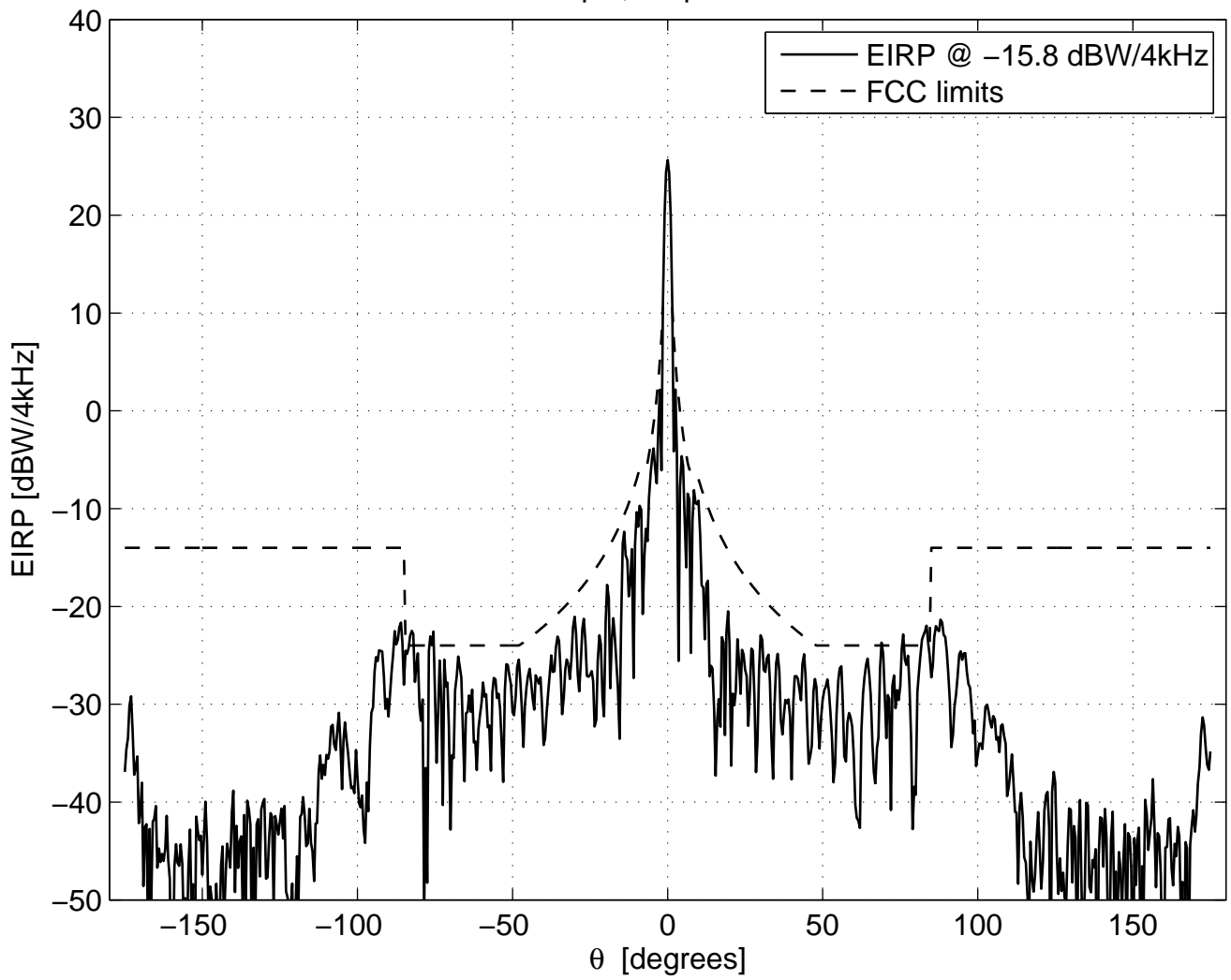
Co-pol, freq=14 GHz
