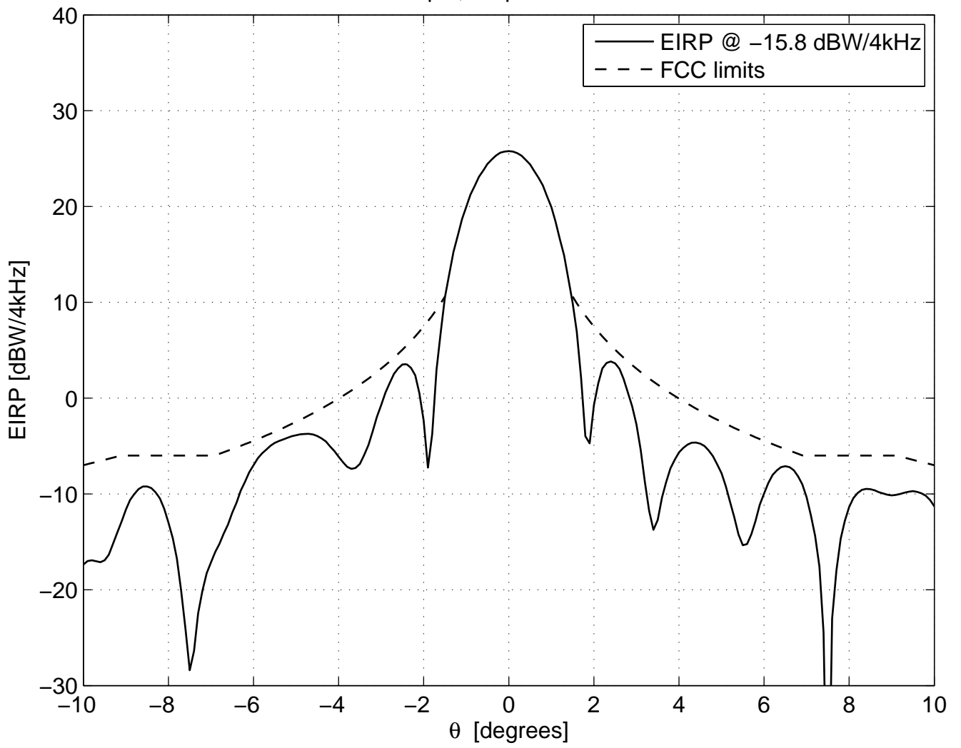
Co-pol, freq=14.25 GHz
