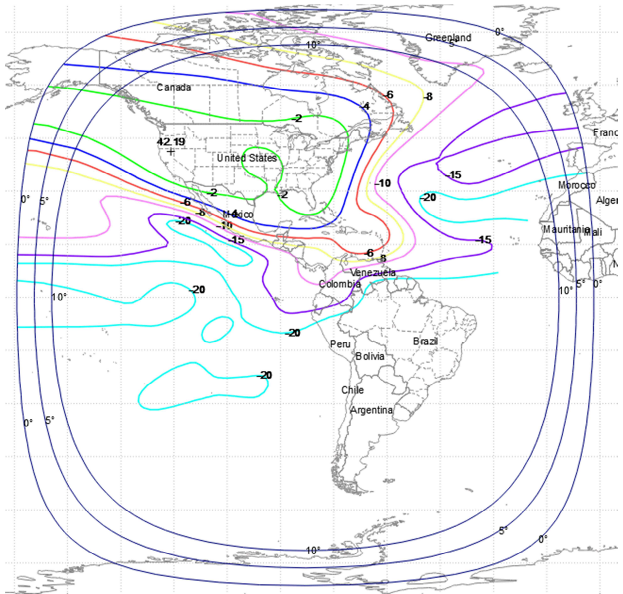
Figure 3: AMC-6 C-Band Beam Vertical Pol (Channel 13) EIRP Contour
