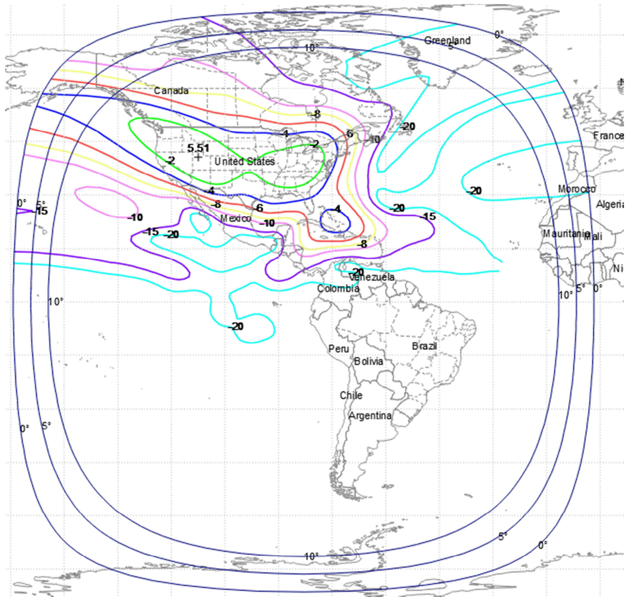
Figure 2: AMC-6 C-Band Beam Vertical Pol (Channel 12) G/T Contour
