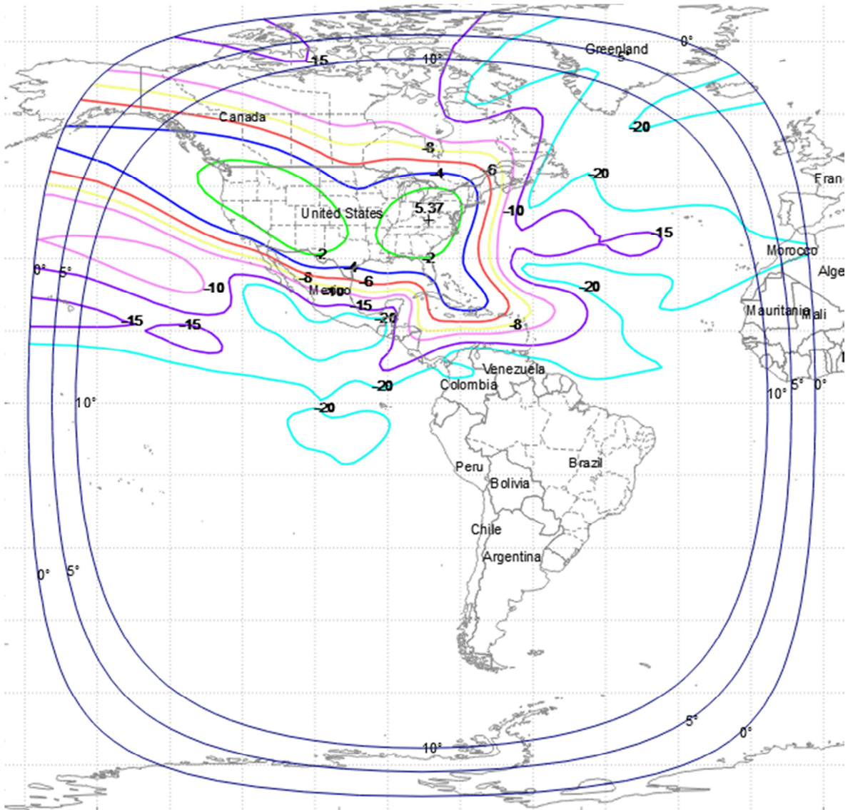
Figure 4: AMC-6 C-Band Beam Horizontal Pol (Channel 13) G/T Contour
