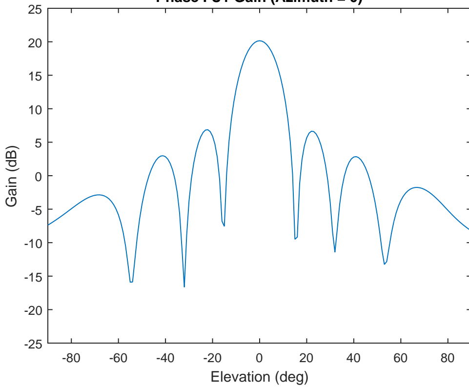
Phase I U1 Gain (Azimuth = 0)
