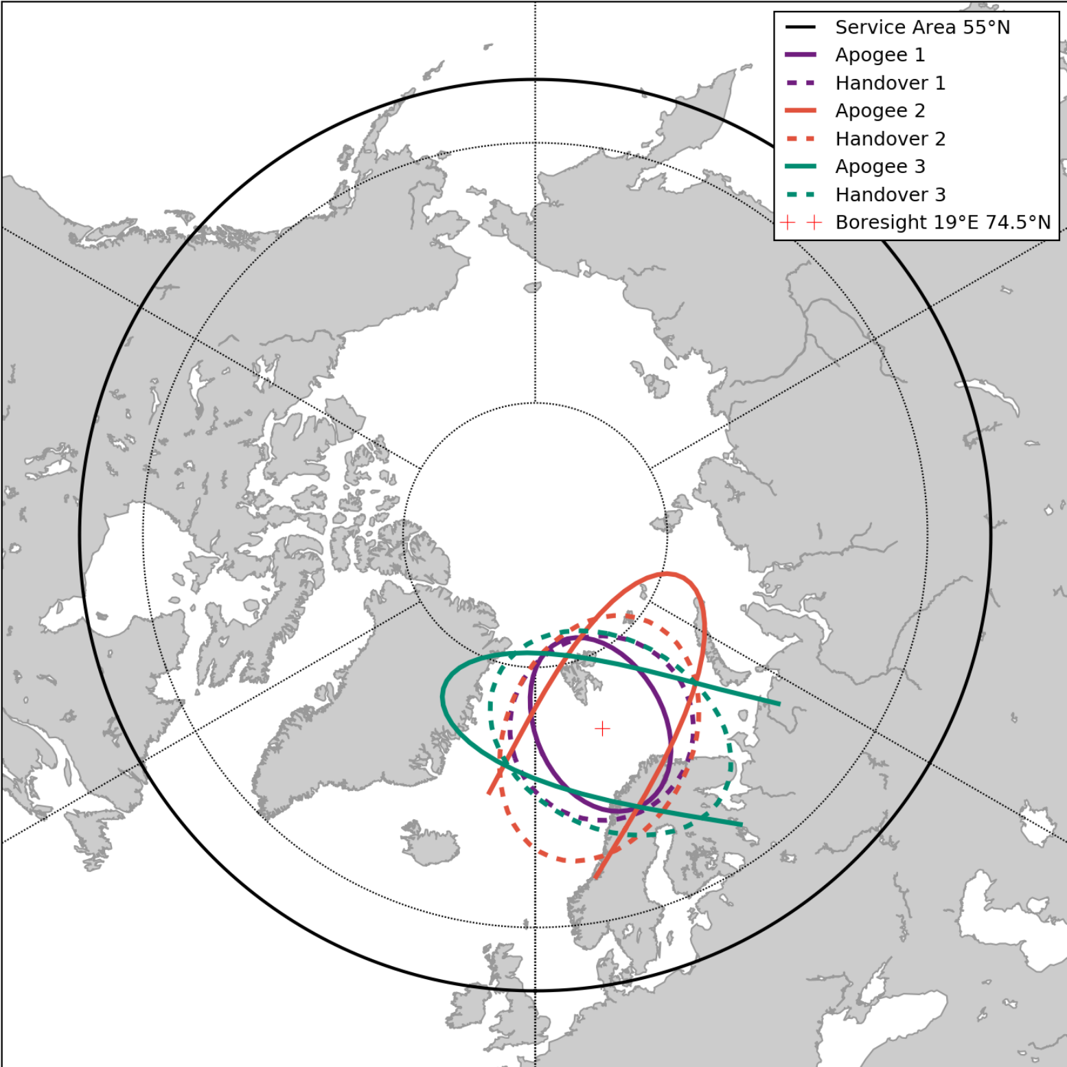
Gateway beam coverage ASBM (2 degree beam)
