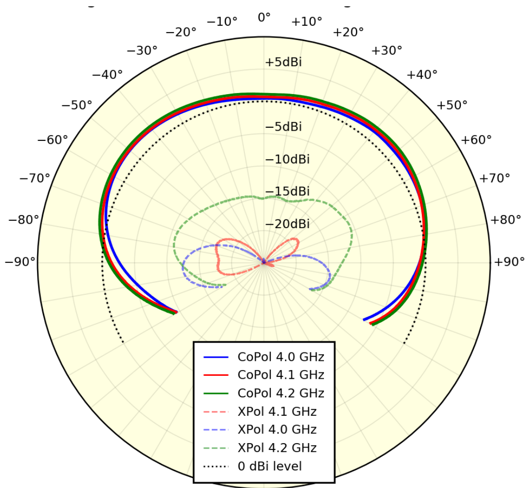
C-band receiver quad helix low-gain antenna pattern measurement (peak gain of 3 dBi)
