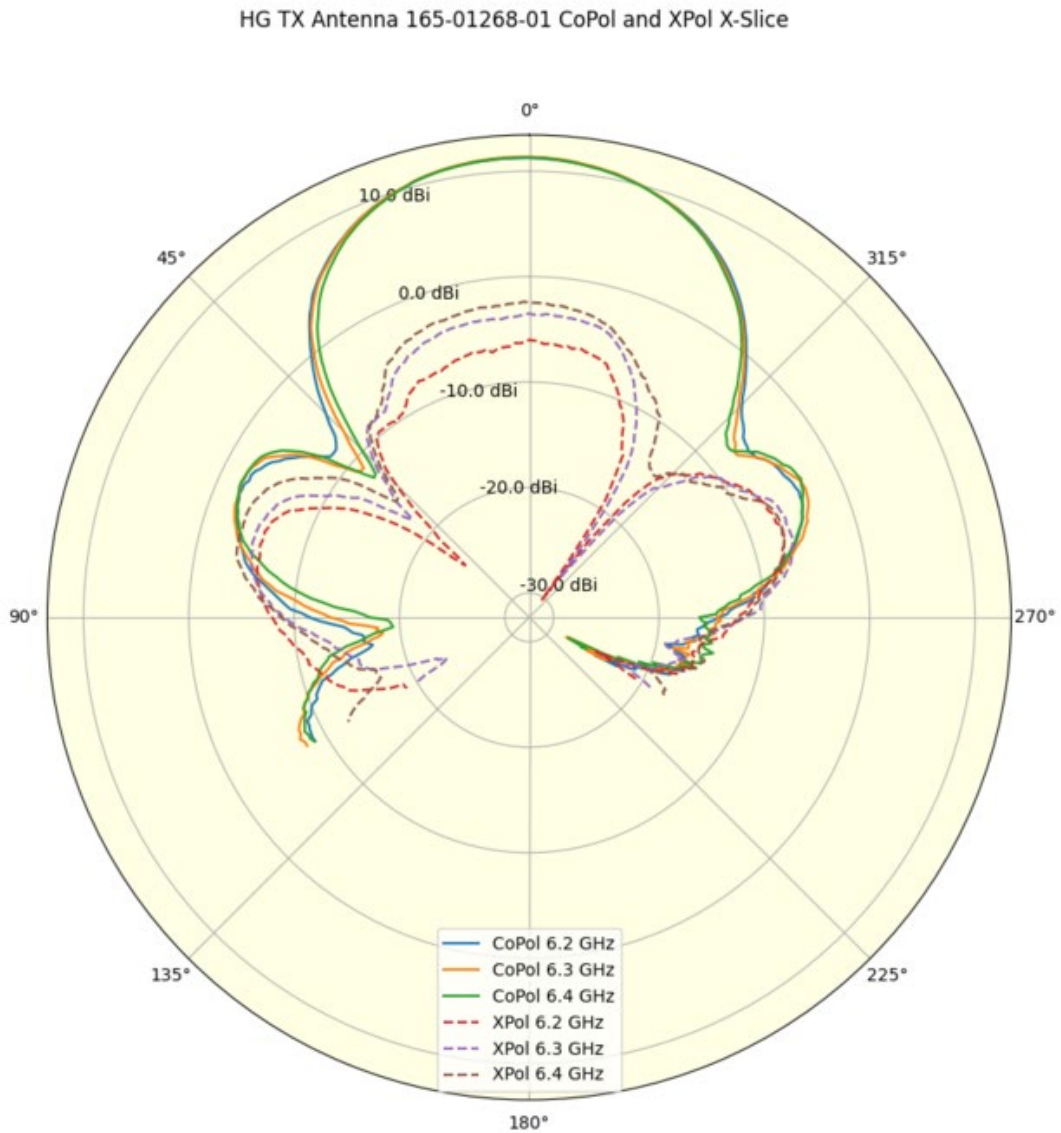
C-band transmitter single helix high-gain antenna pattern measurement (peak gain of 12 dBi)
