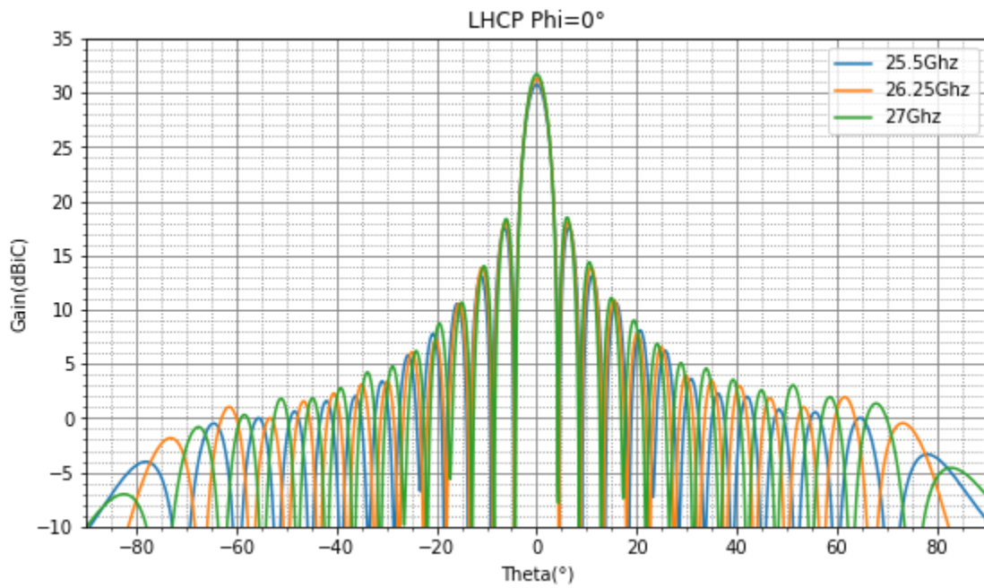
Downlink Ka-band transmitter LHCP antenna pattern simulation, \phi cut at 0^\circ
