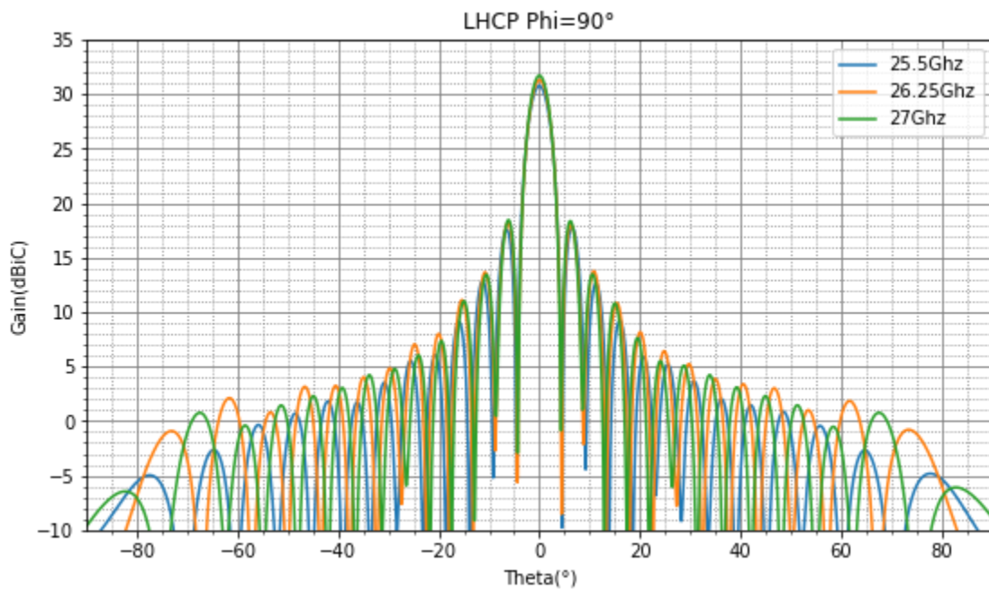
Downlink Ka-band transmitter LHCP antenna pattern simulation, \phi cut at 90^\circ
