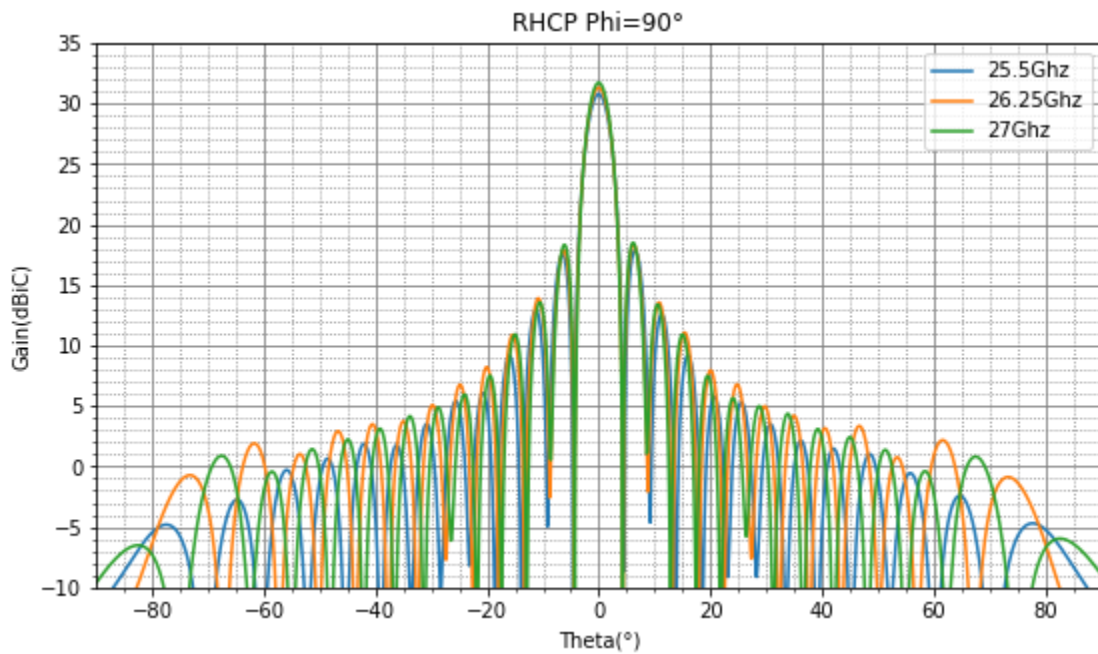
Downlink Ka-band transmitter RHCP antenna pattern simulation, \phi cut at 90^\circ
