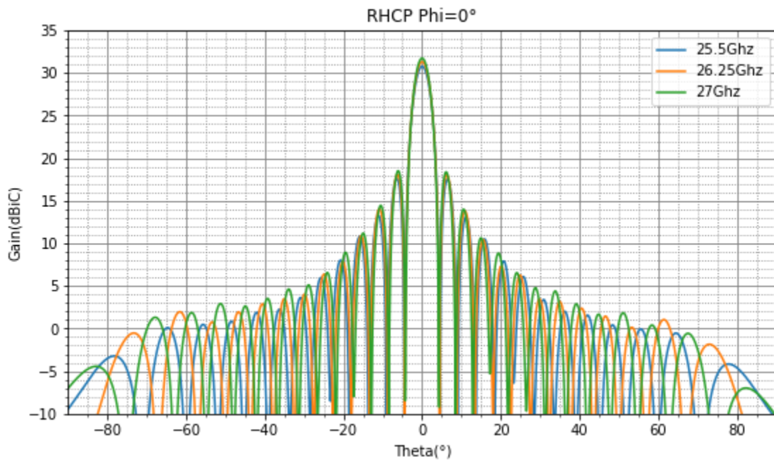
Downlink Ka-band transmitter RHCP antenna pattern simulation, \phi cut at 0^\circ
