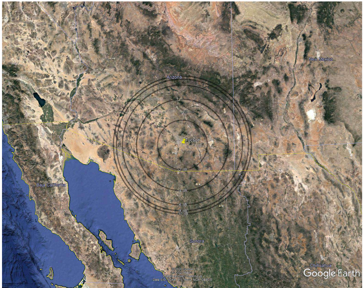
Figure 2 Apogee 450km – Orbital Planes 2, 3, 4
