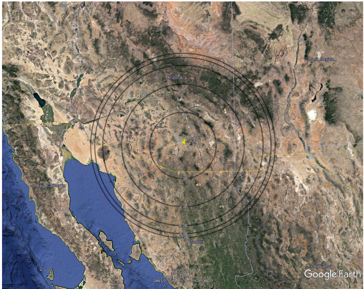
Figure 5 Apogee 600km – Orbital Planes 10, 11
