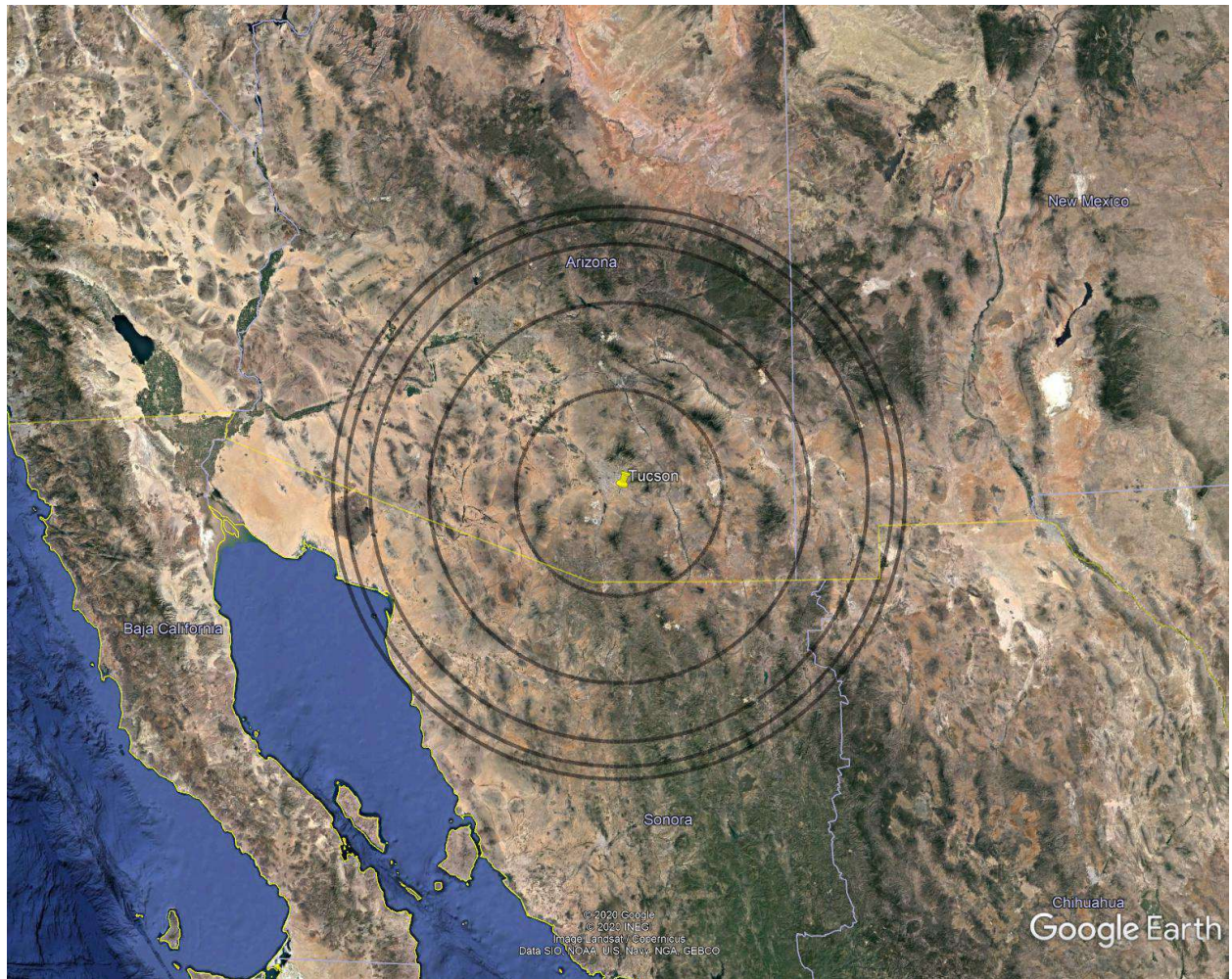
Figure 4 Apogee 550km – Orbital Planes 8, 9
