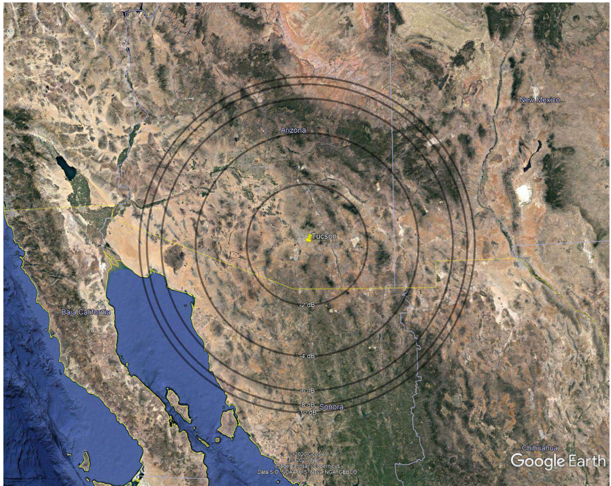
Figure 6 Apogee 650km – Orbital Planes 12, 13
