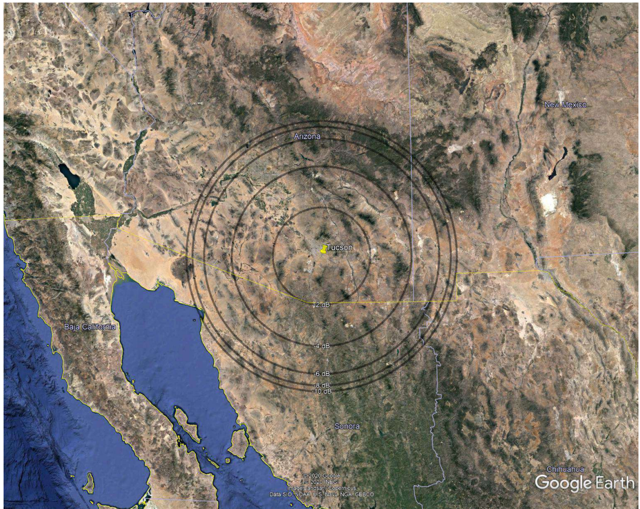
Figure 3 Apogee 500km – Orbital Planes 5, 6, 7
