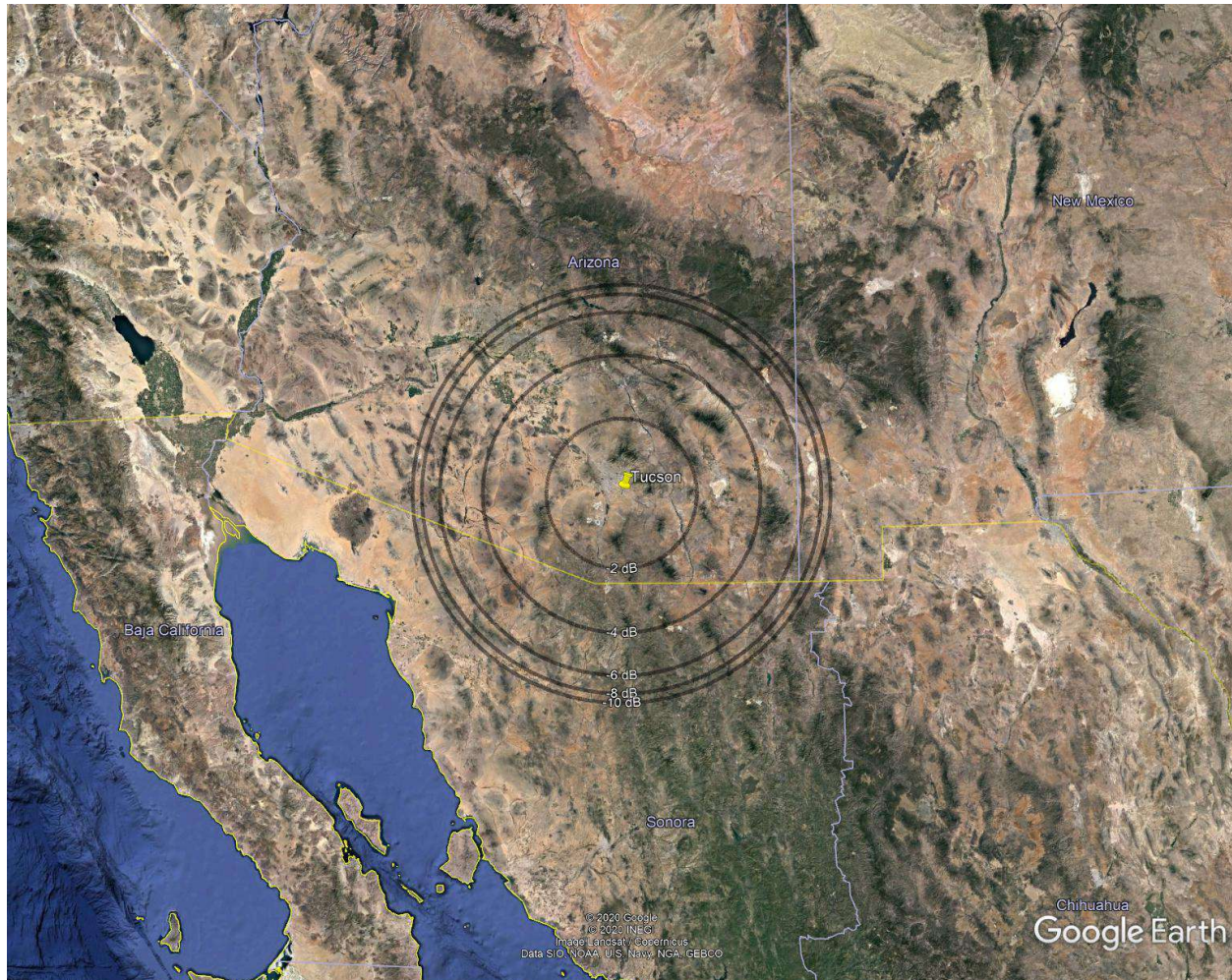
Figure 1 Apogee 400km – Orbital Plane 1
