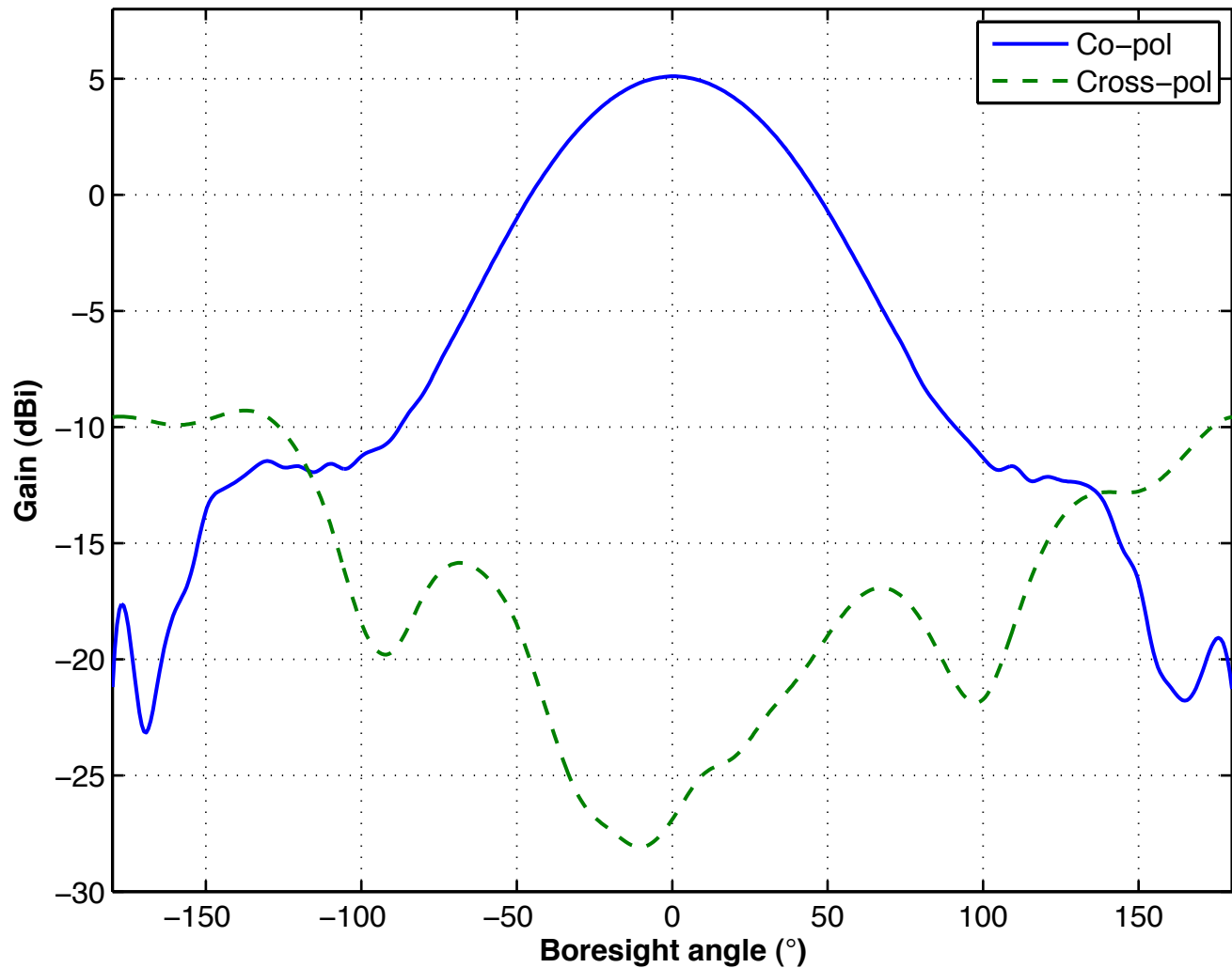
TT&C X-band antenna (RHCP)
