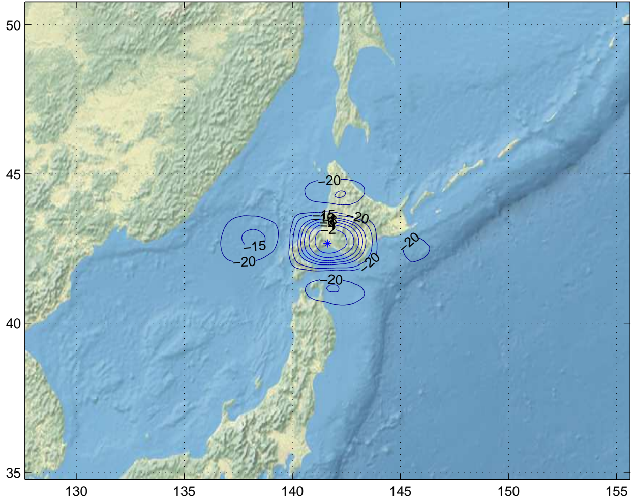
Gain Contours at 385km for CTS. Beam ID=XTC, Polarization=rhcp
