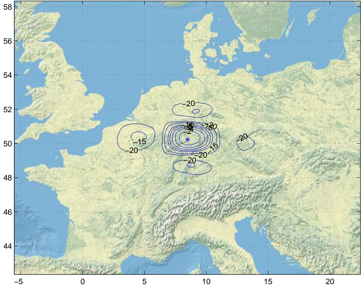
Gain Contours at 385km for FRA. Beam ID=XTC, Polarization=rhcp
