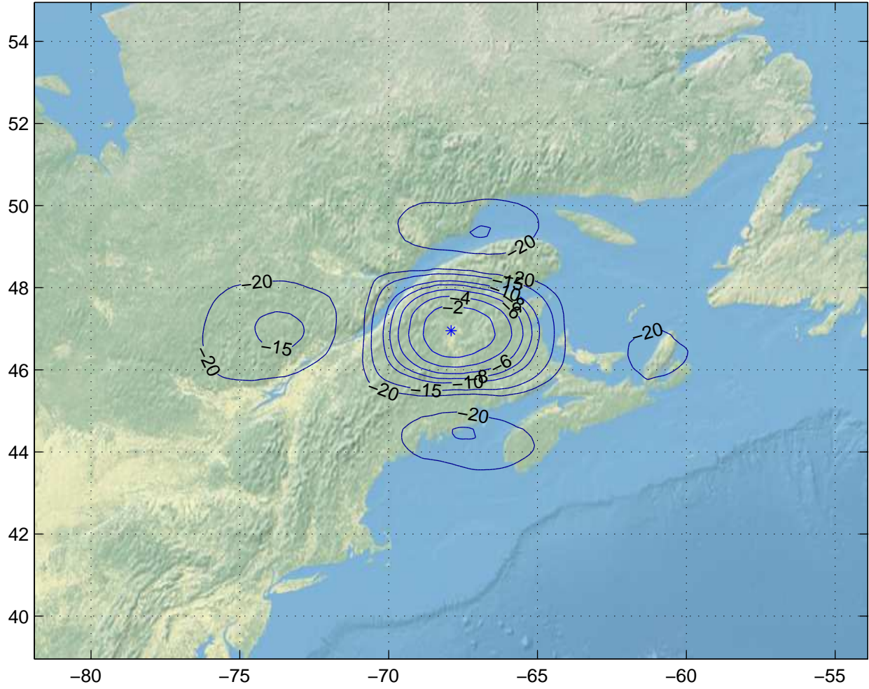
Gain Contours at 600km for PQI. Beam ID=XTC, Polarization=rhcp
