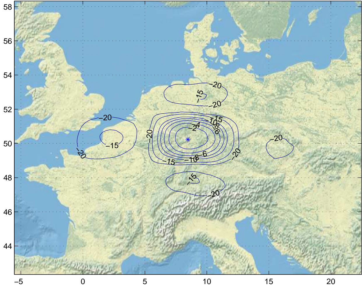
Gain Contours at 600km for FRA. Beam ID=XTC, Polarization=rhcp
