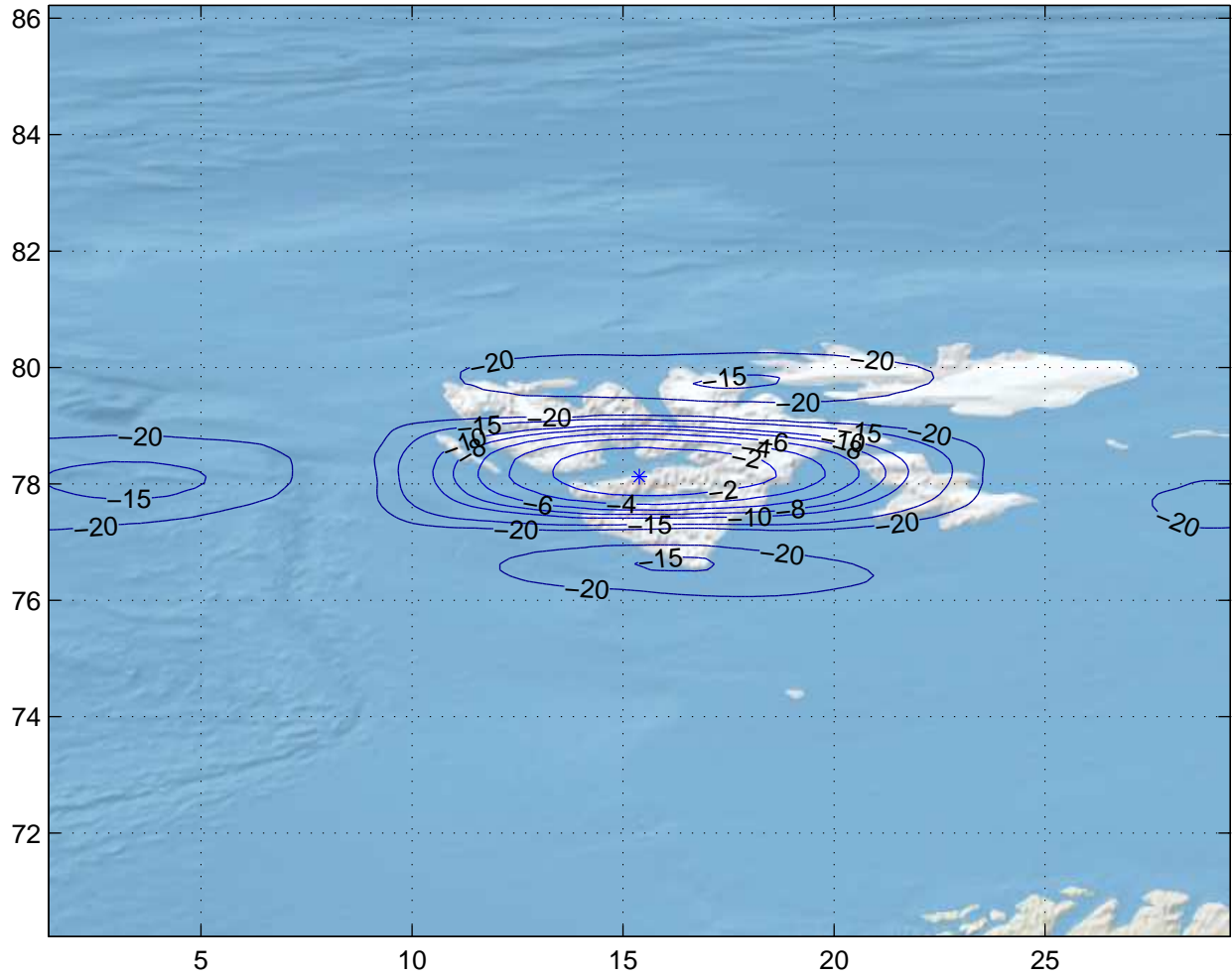
Gain Contours at 385km for LYR. Beam ID=XTC, Polarization=rhcp
