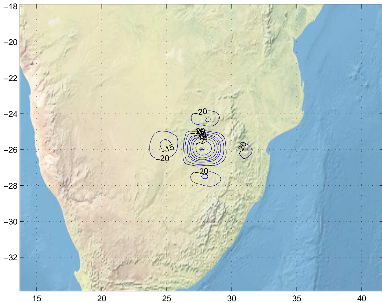
Gain Contours at 385km for JNB. Beam ID=XTC, Polarization=rhcp
