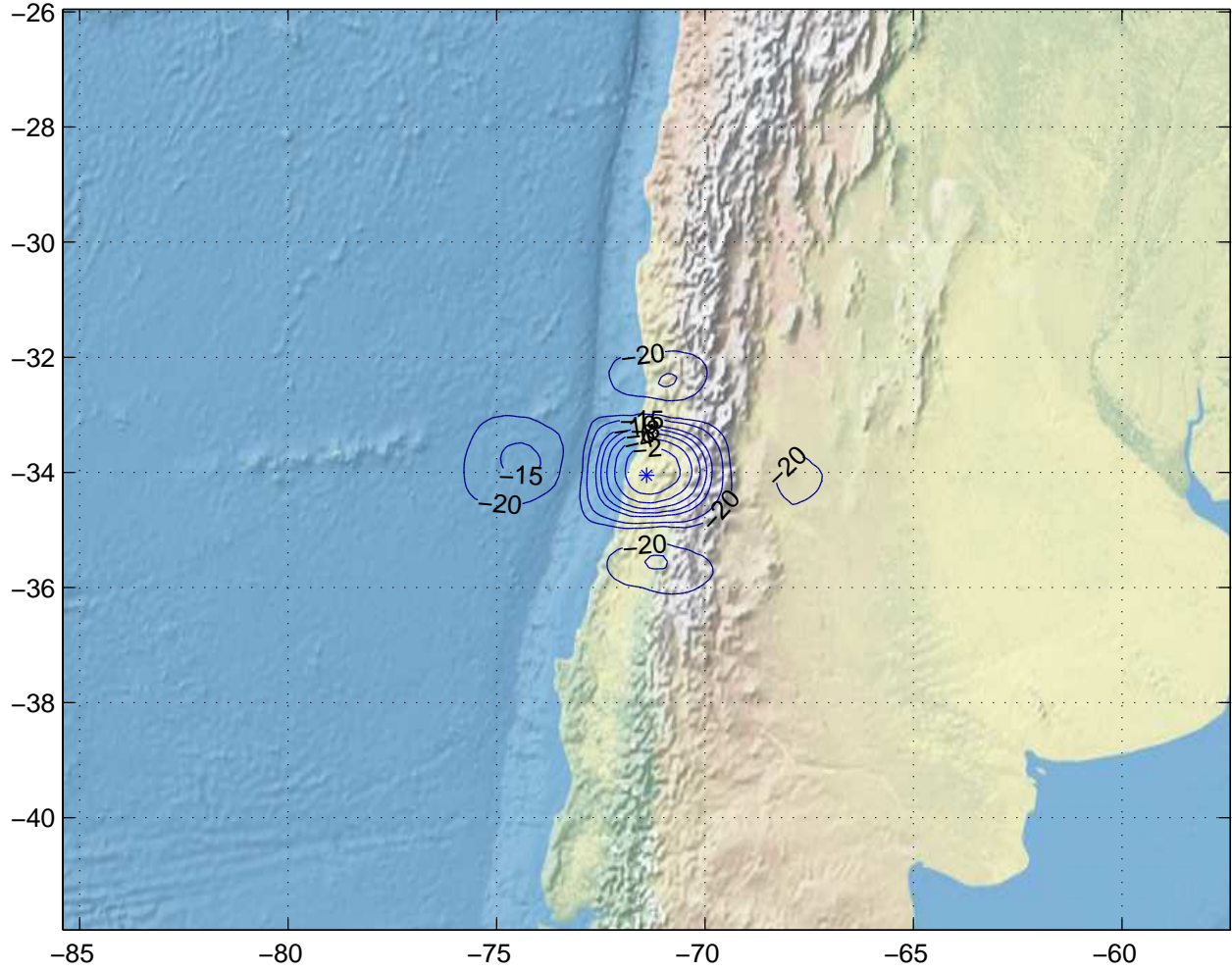
Gain Contours at 385km for SCL. Beam ID=XTC, Polarization=rhcp
