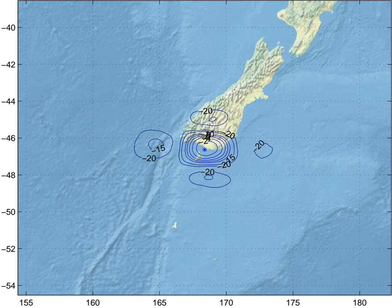
Gain Contours at 385km for IVC. Beam ID=XTC, Polarization=rhcp
