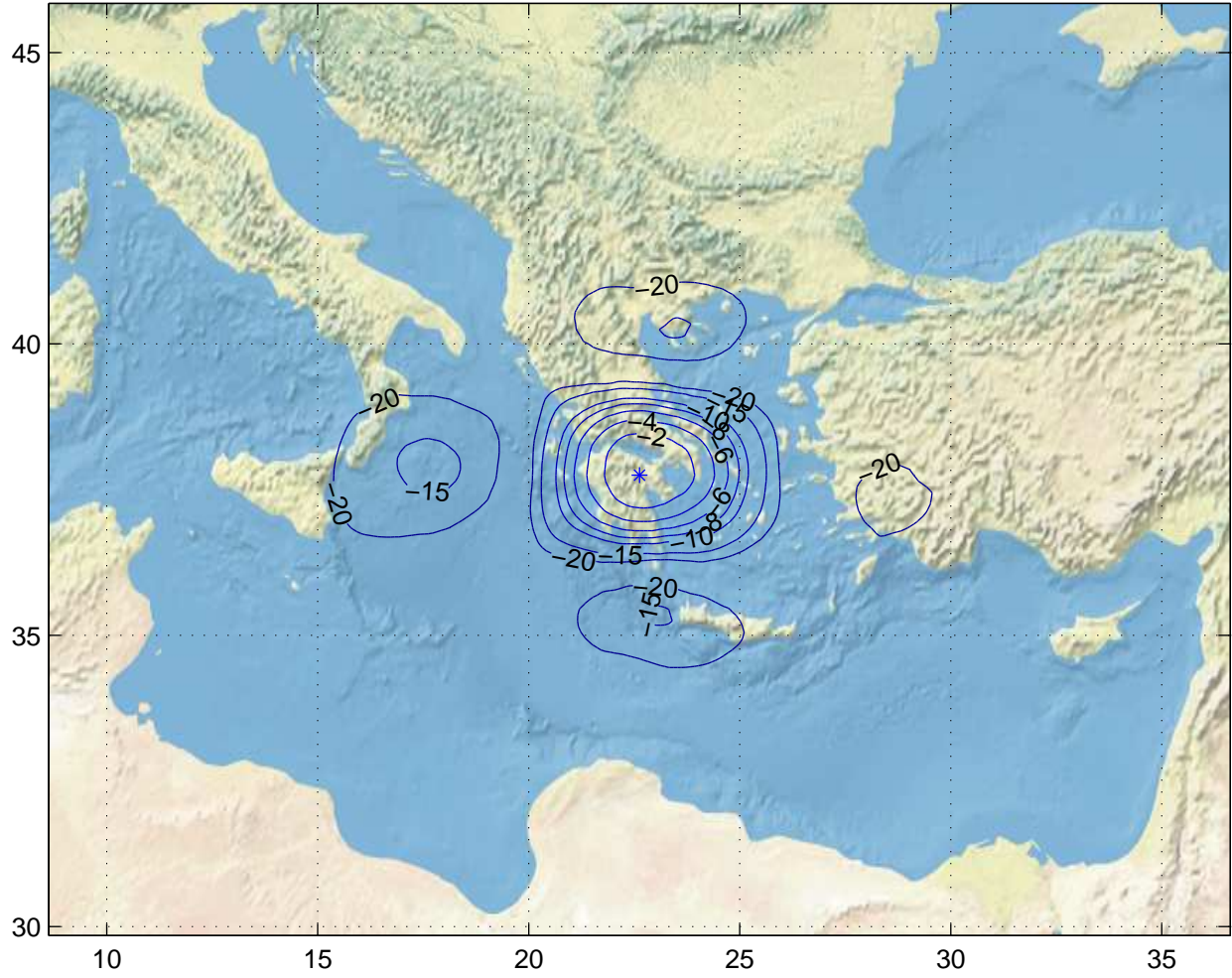
Gain Contours at 600km for ATH. Beam ID=XTC, Polarization=rhcp
