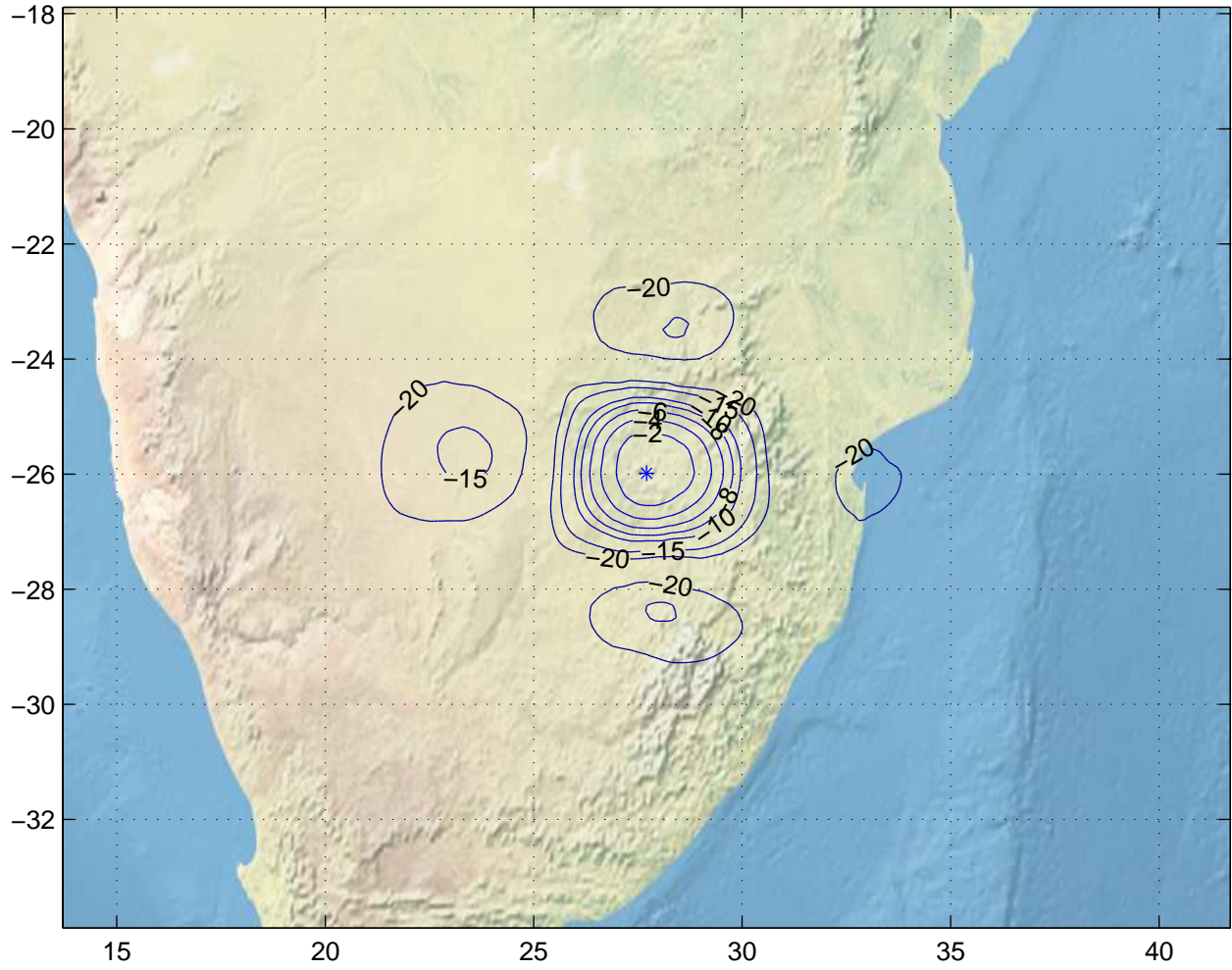
Gain Contours at 600km for JNB. Beam ID=XTC, Polarization=rhcp
