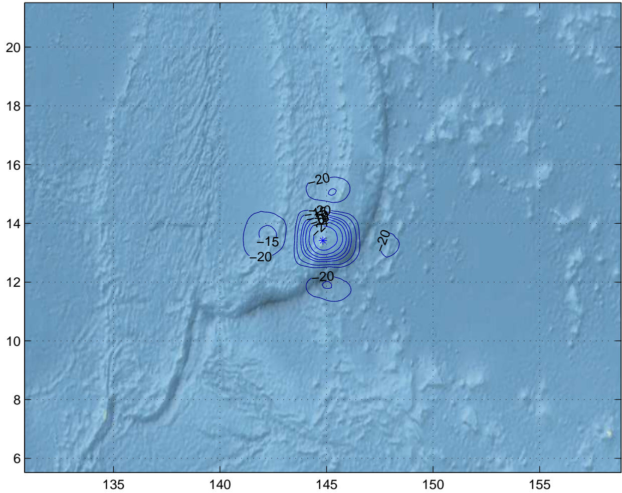
Gain Contours at 385km for GUM. Beam ID=XTC, Polarization=rhcp
