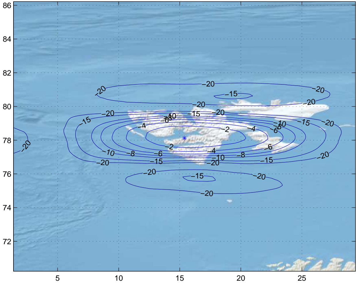
Gain Contours at 600km for LZR. Beam ID=XTC, Polarization=rhcp
