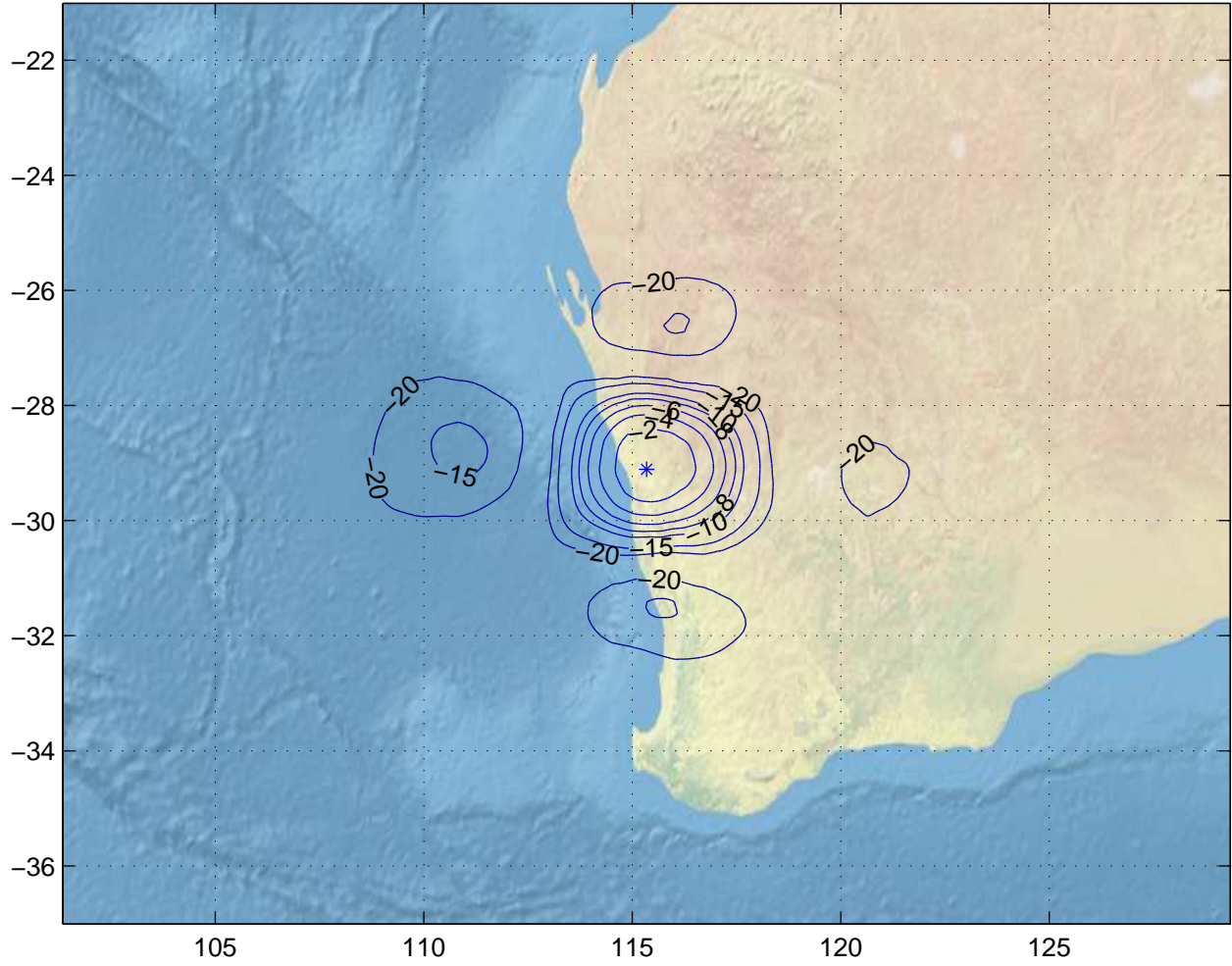
Gain Contours at 600km for GET. Beam ID=XTC, Polarization=rhcp
