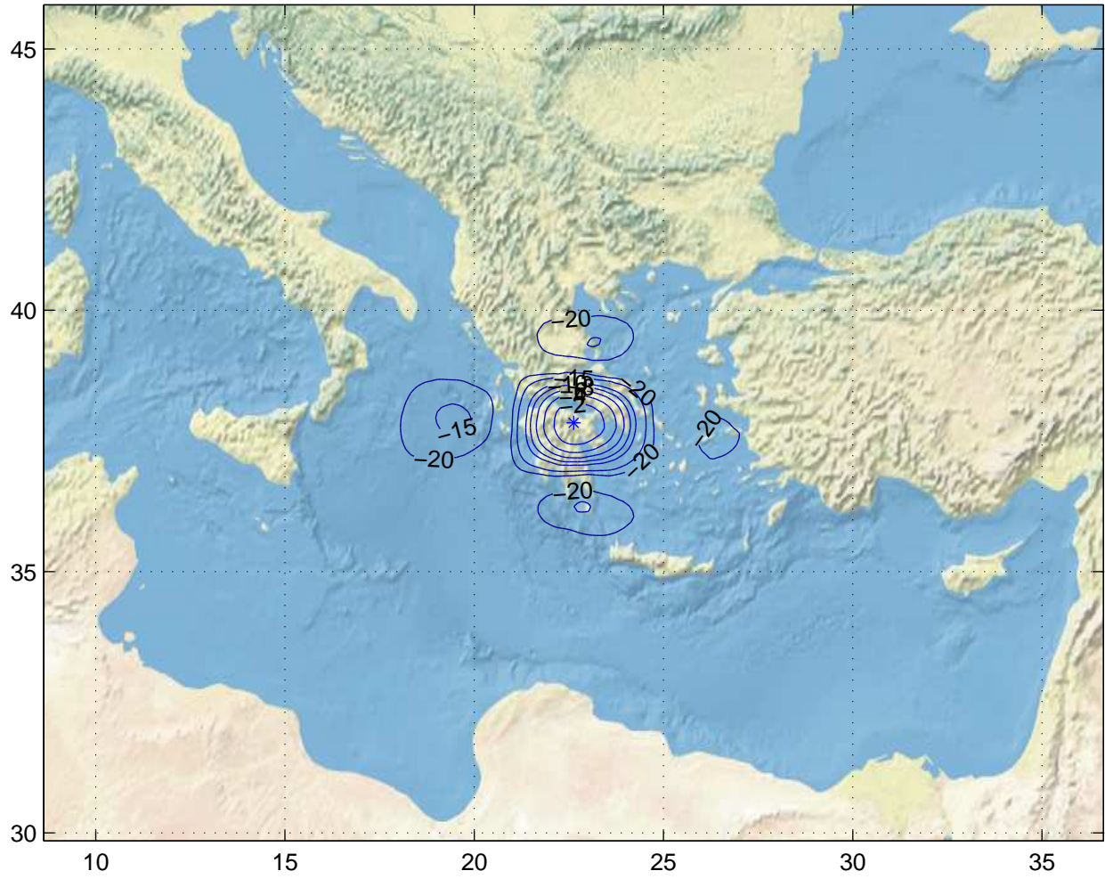
Gain Contours at 385km for ATH. Beam ID=XTC, Polarization=rhcp
