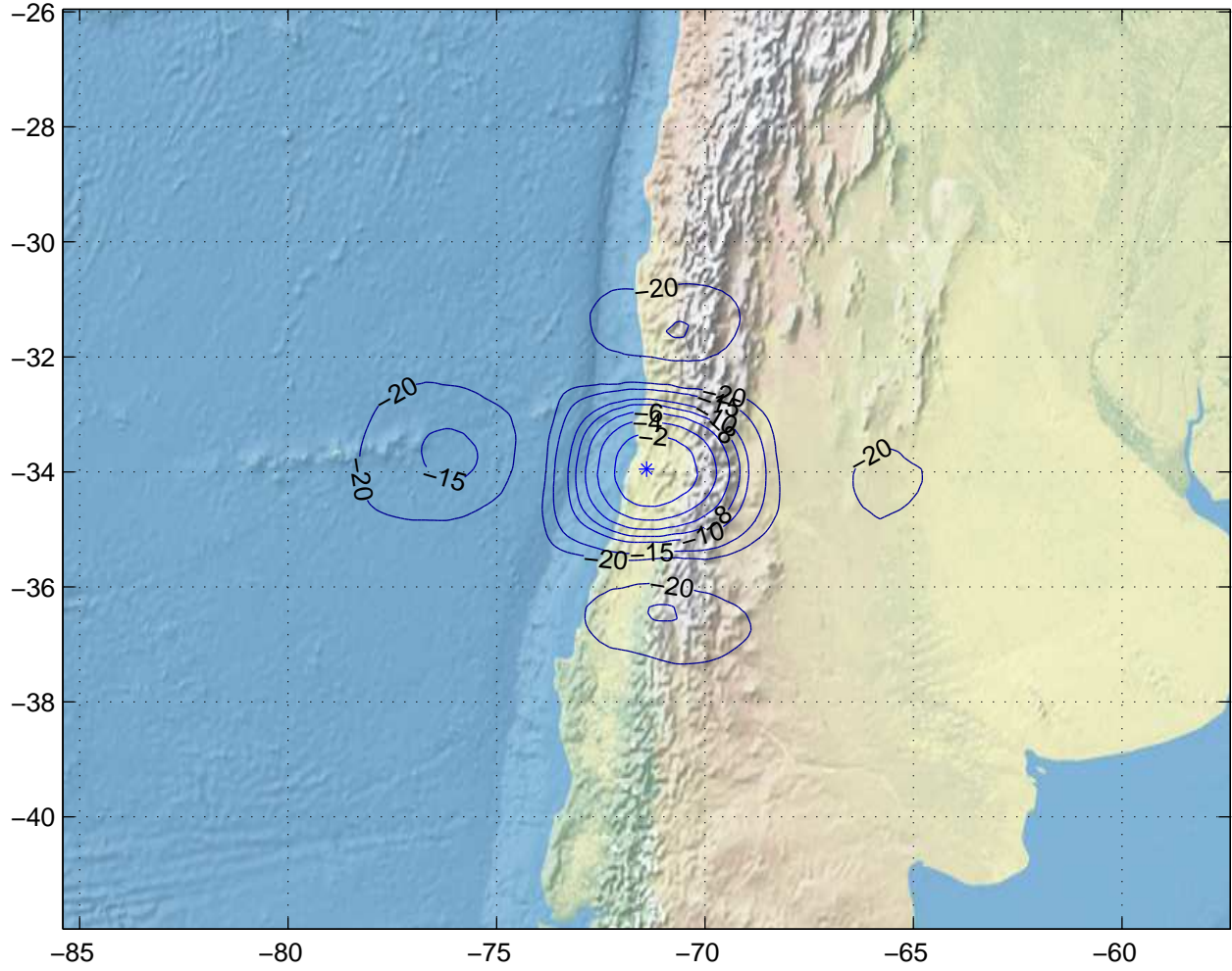
Gain Contours at 600km for SCL. Beam ID=XTC, Polarization=rhcp
