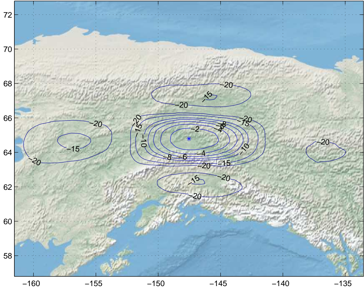
Gain Contours at 600km for FAI. Beam ID=XTC, Polarization=rhcp
