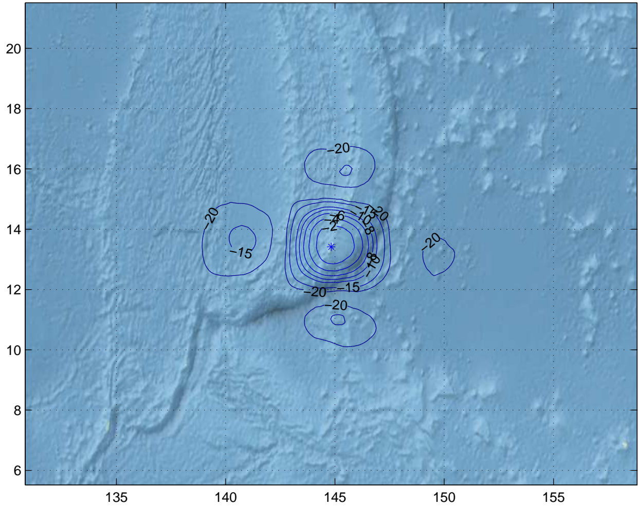
Gain Contours at 600km for GUM. Beam ID=XTC, Polarization=rhcp
