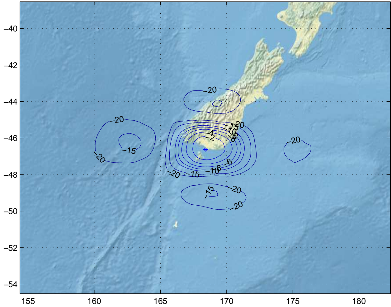
Gain Contours at 600km for IVC. Beam ID=XTC, Polarization=rhcp
