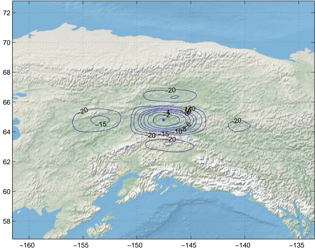
Gain Contours at 385km for FAI. Beam ID=XTC, Polarization=rhcp
