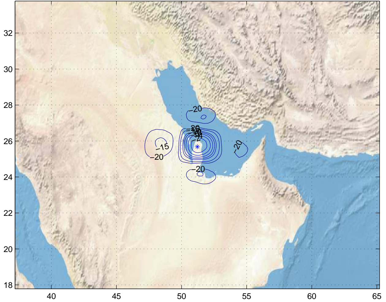
Gain Contours at 385km for DOH. Beam ID=XTC, Polarization=rhcp
