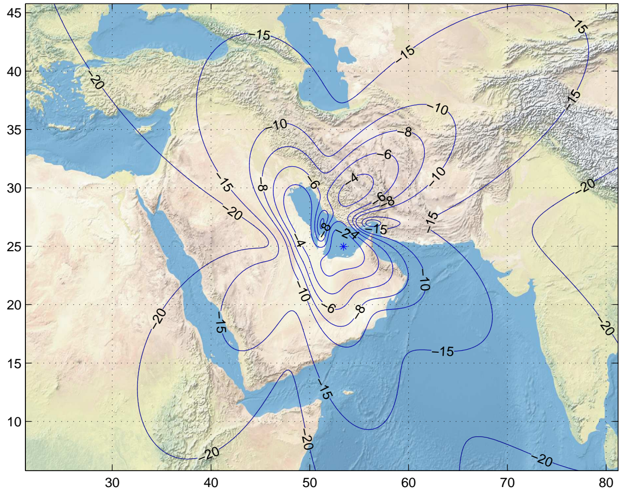
Gain Contours at 385km for DOH. Beam ID=UTX, Polarization=rhcp
