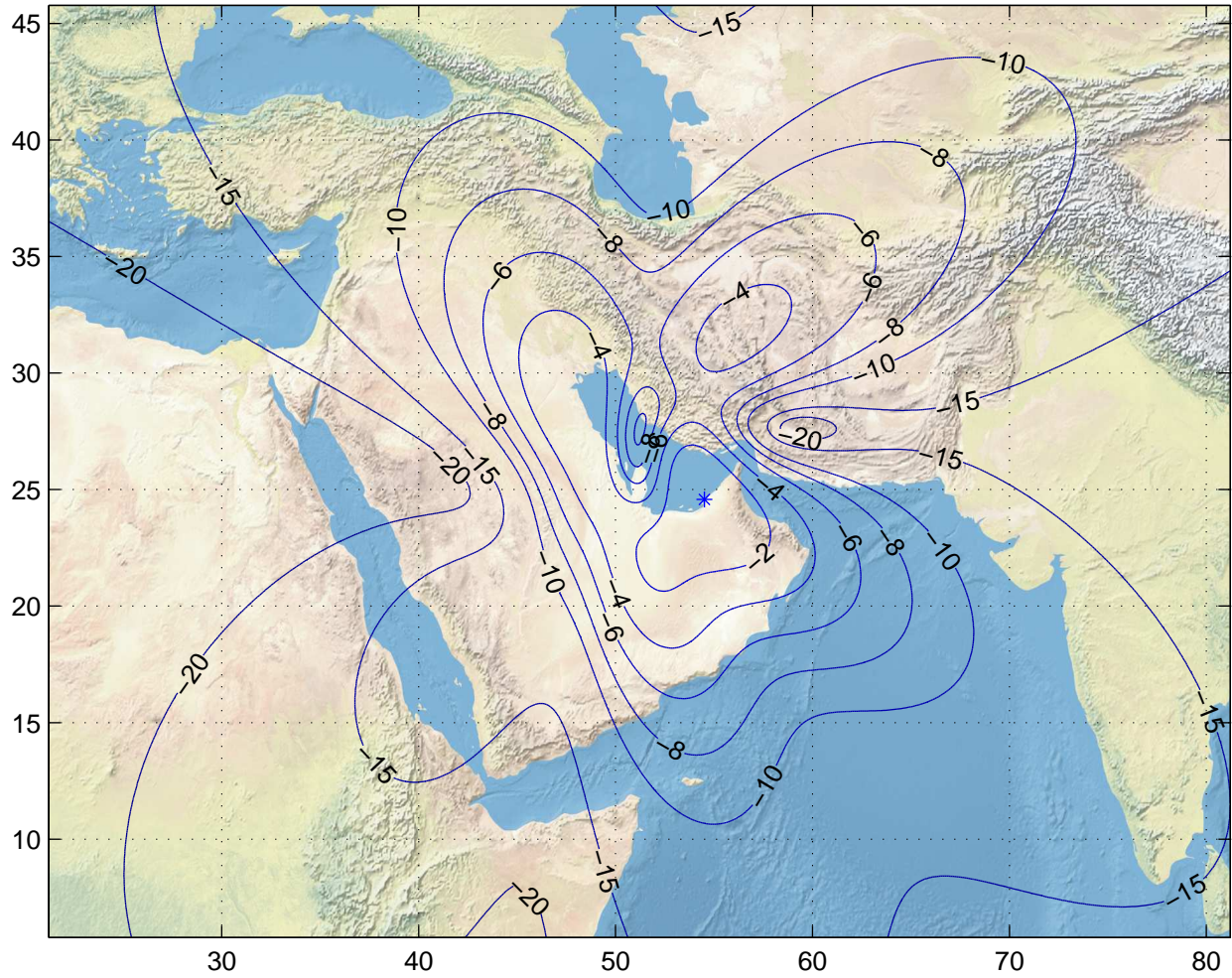
Gain Contours at 600km for DOH. Beam ID=UTX, Polarization=rhcp
