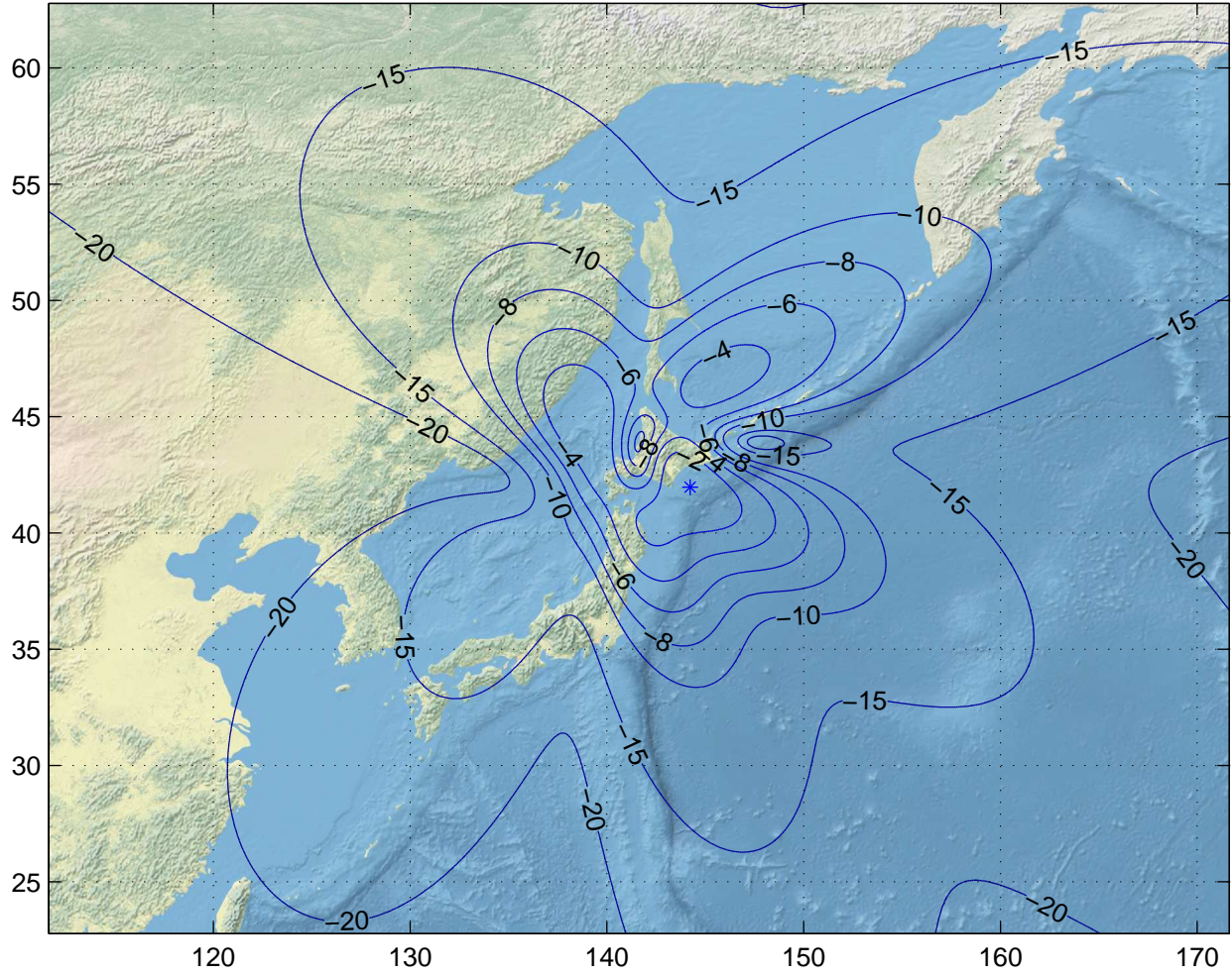
Gain Contours at 385km for CTS. Beam ID=UTX, Polarization=rhcp
