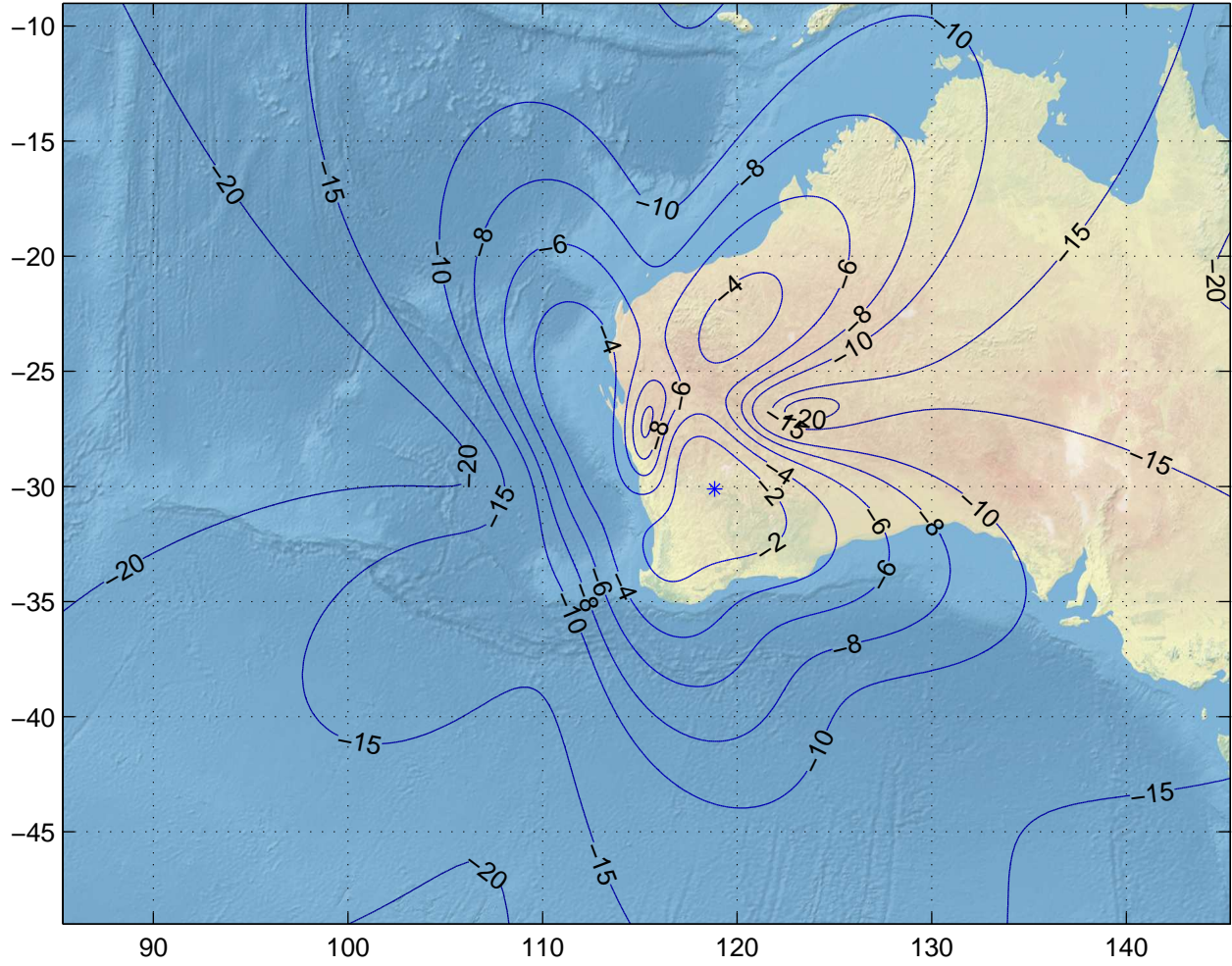
Gain Contours at 600km for GET. Beam ID=UTX, Polarization=rhpc
