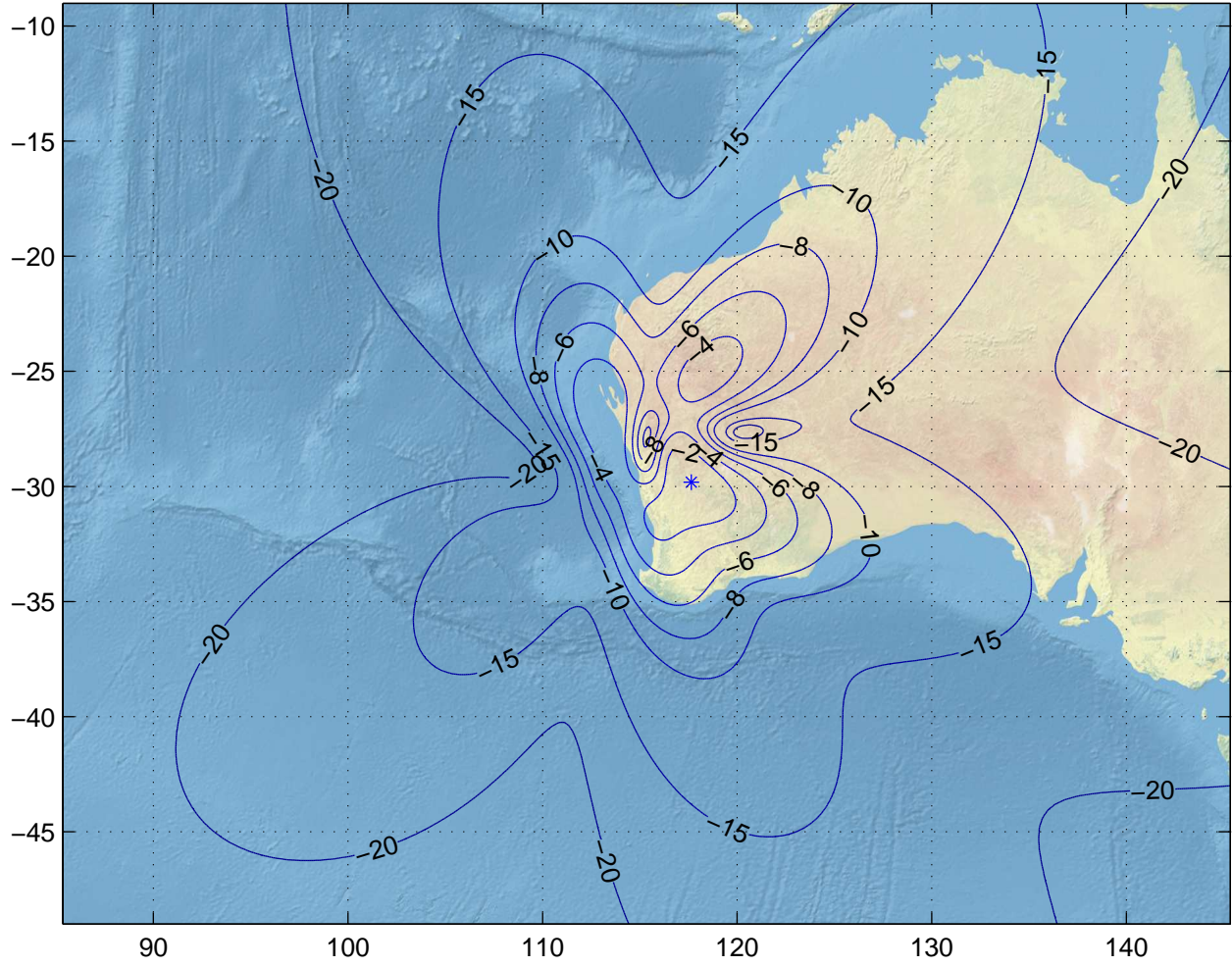
Gain Contours at 385km for GET. Beam ID=UTX, Polarization=rhcp
