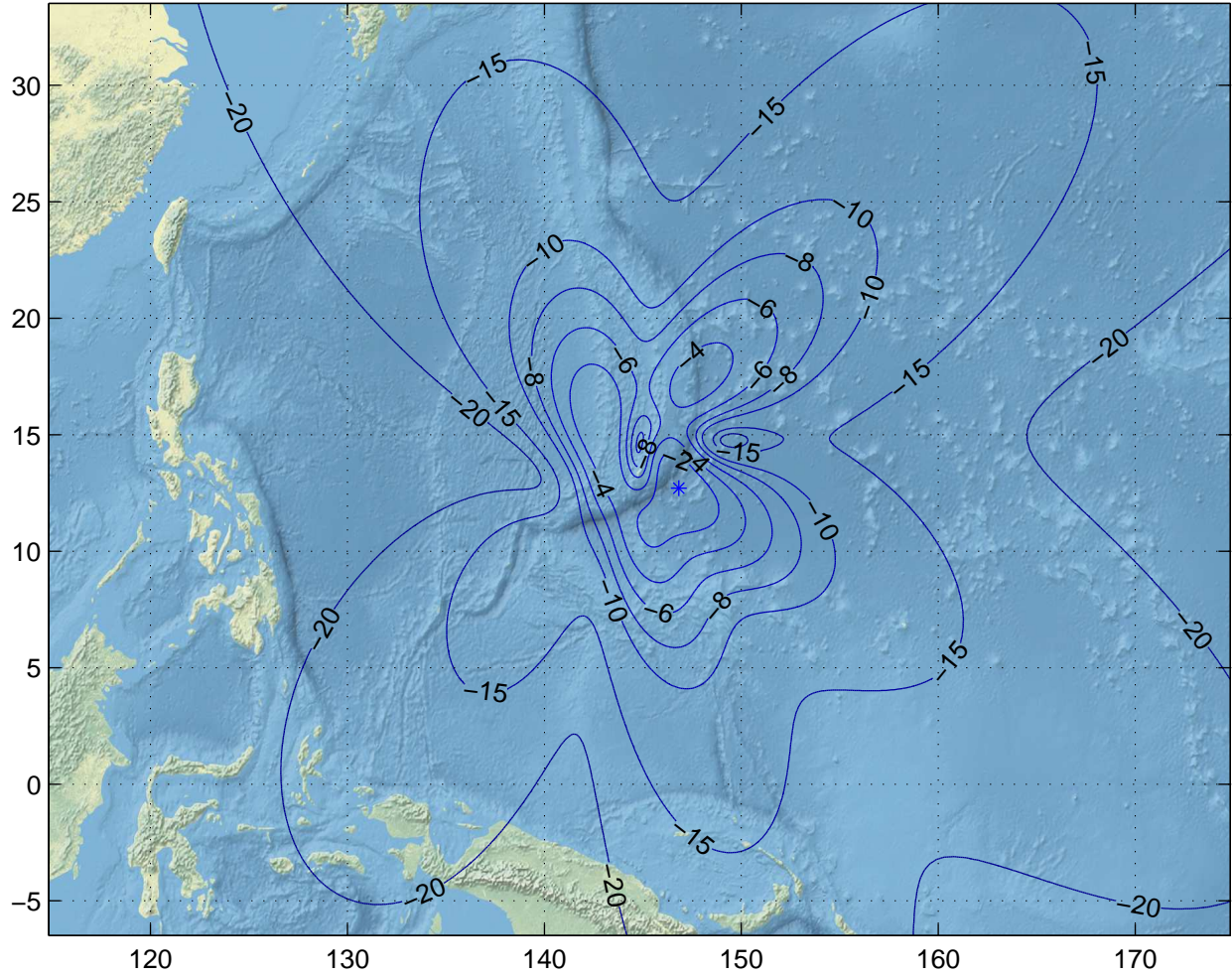
Gain Contours at 385km for GUM. Beam ID=UTX, Polarization=rhcp
