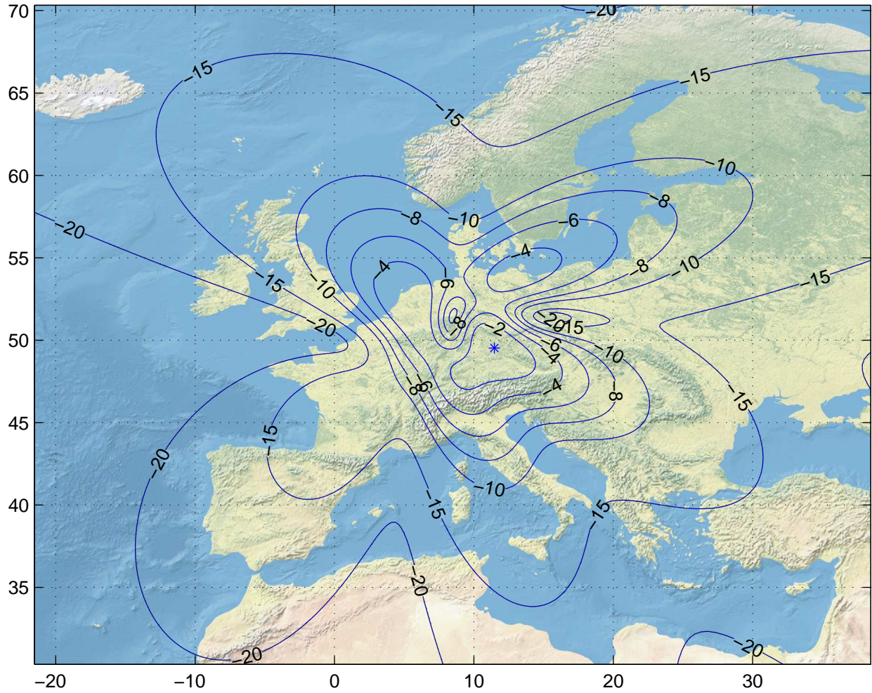
Gain Contours at 385km for FRA. Beam ID=UTX, Polarization=rhcp
