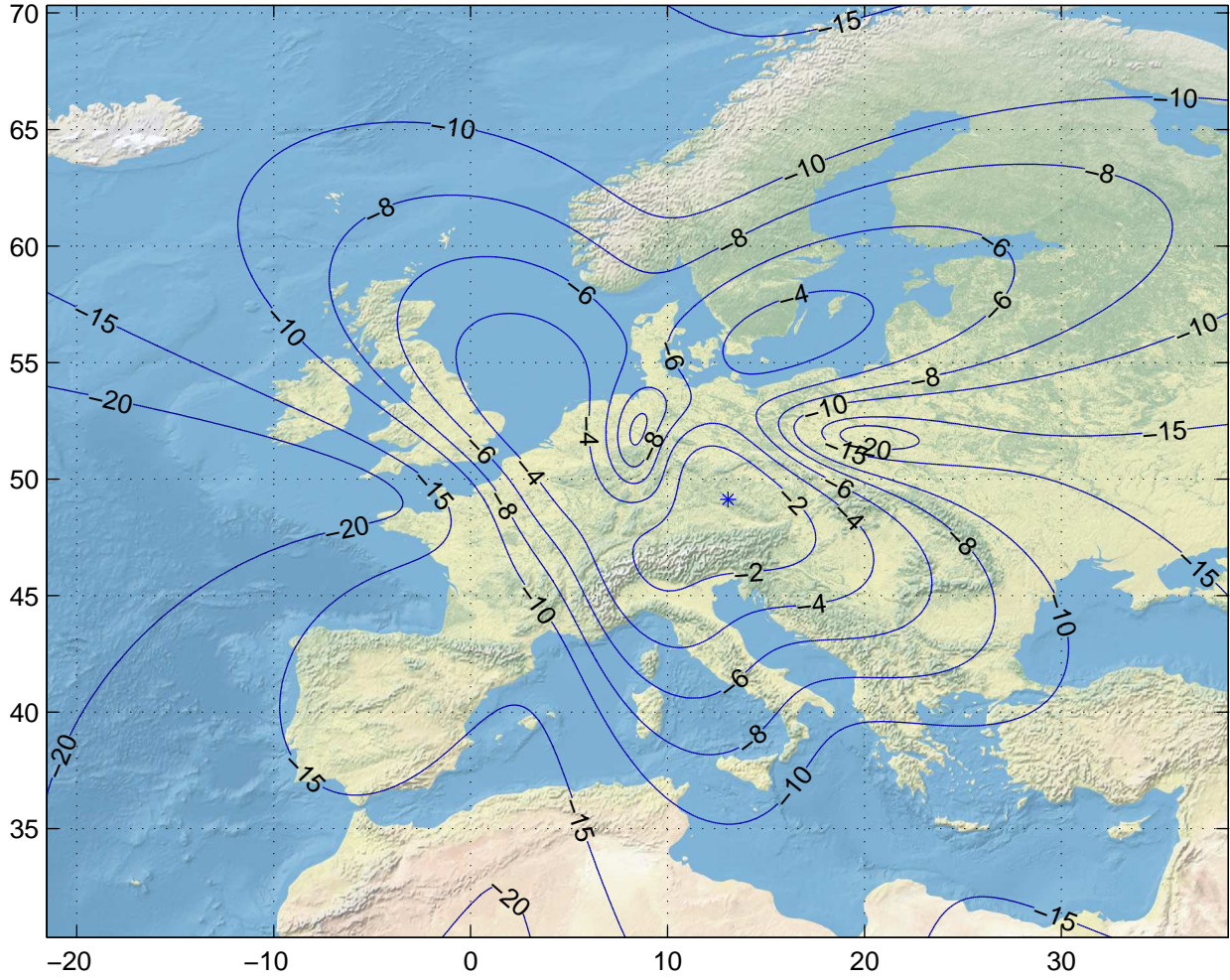
Gain Contours at 600km for FRA. Beam ID=UTX, Polarization=rhcp
