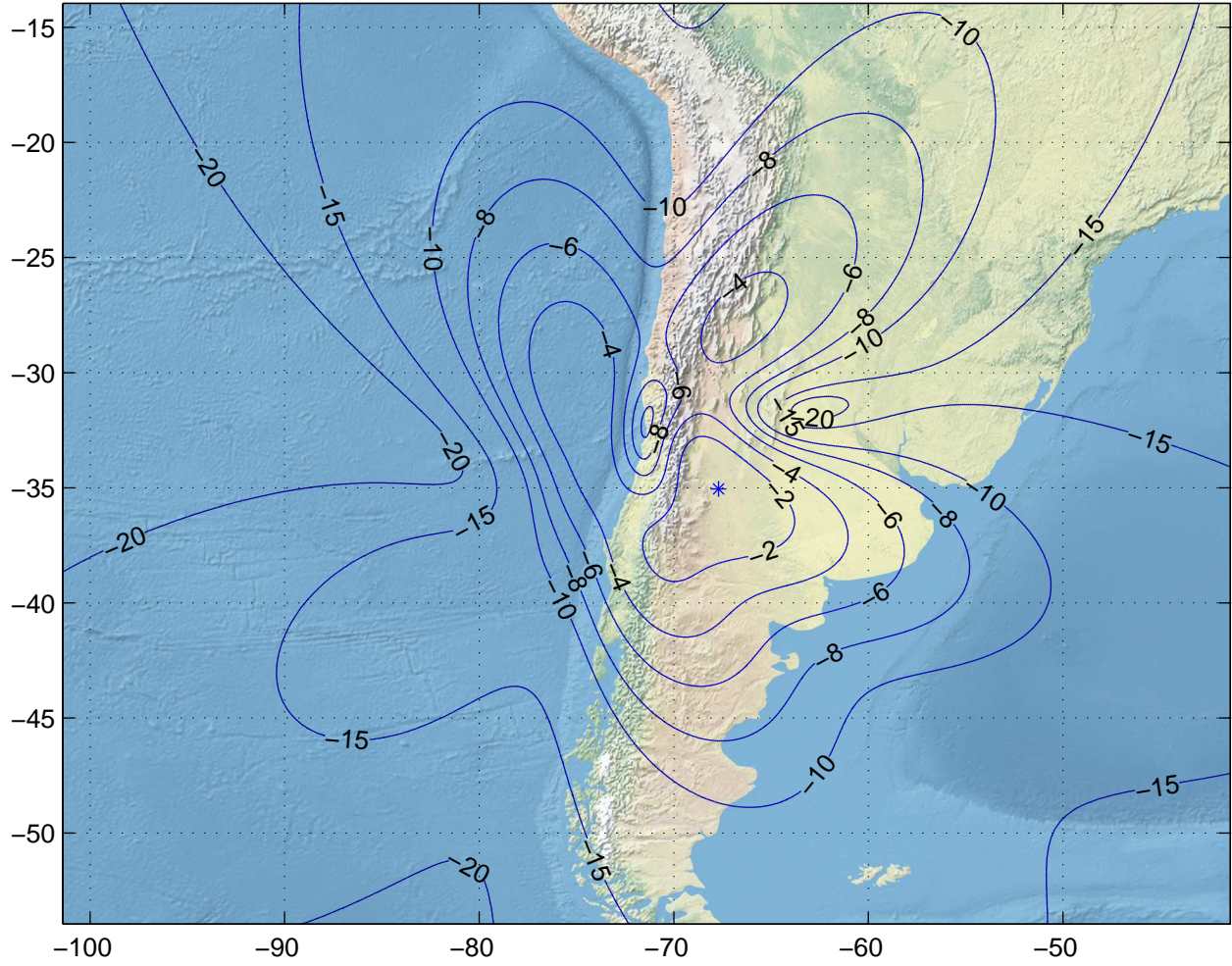
Gain Contours at 600km for SCL. Beam ID=UTX, Polarization=rhcp
