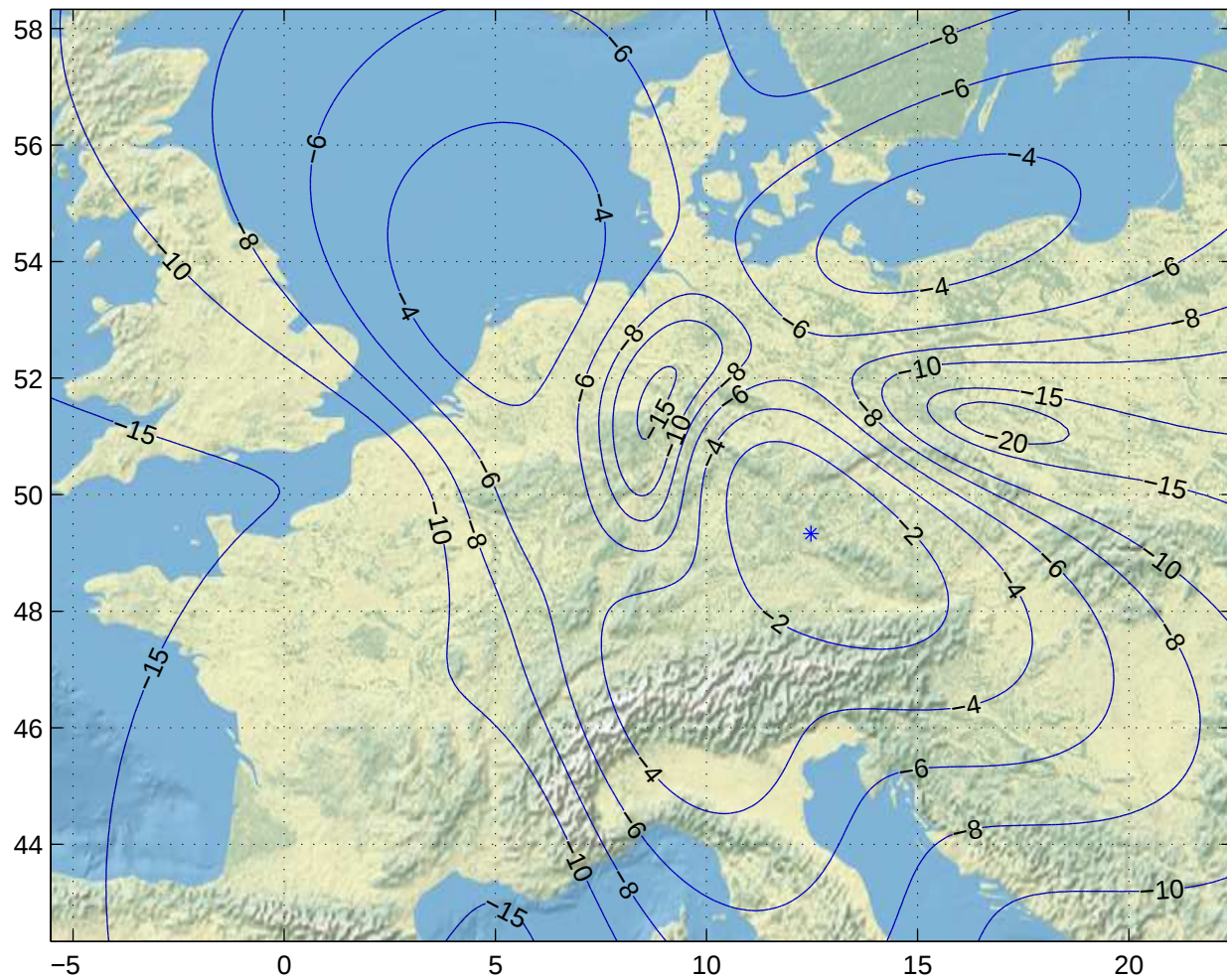
Gain Contours at 475km for FRA. Beam ID=URC, Polarization=h
