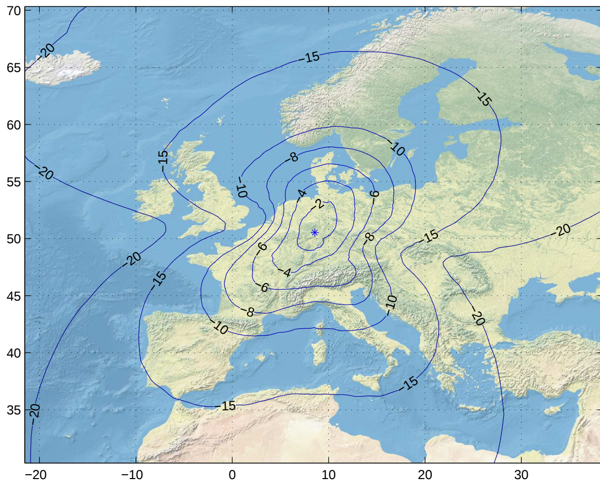
Gain Contours at 475km for FRA. Beam ID=SRX, Polarization=lhcp
