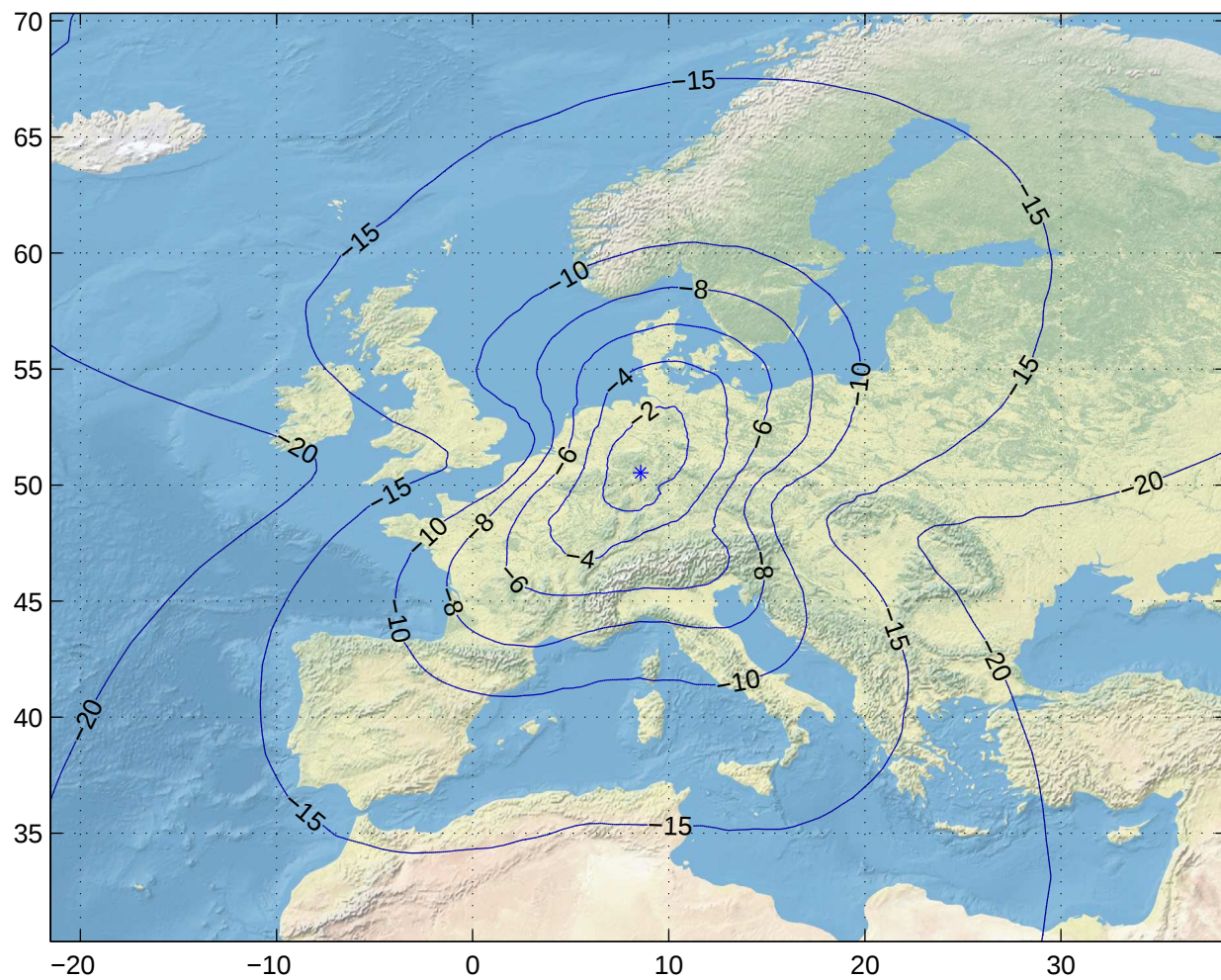
Gain Contours at 505km for FRA. Beam ID=SRX, Polarization=lhcp
