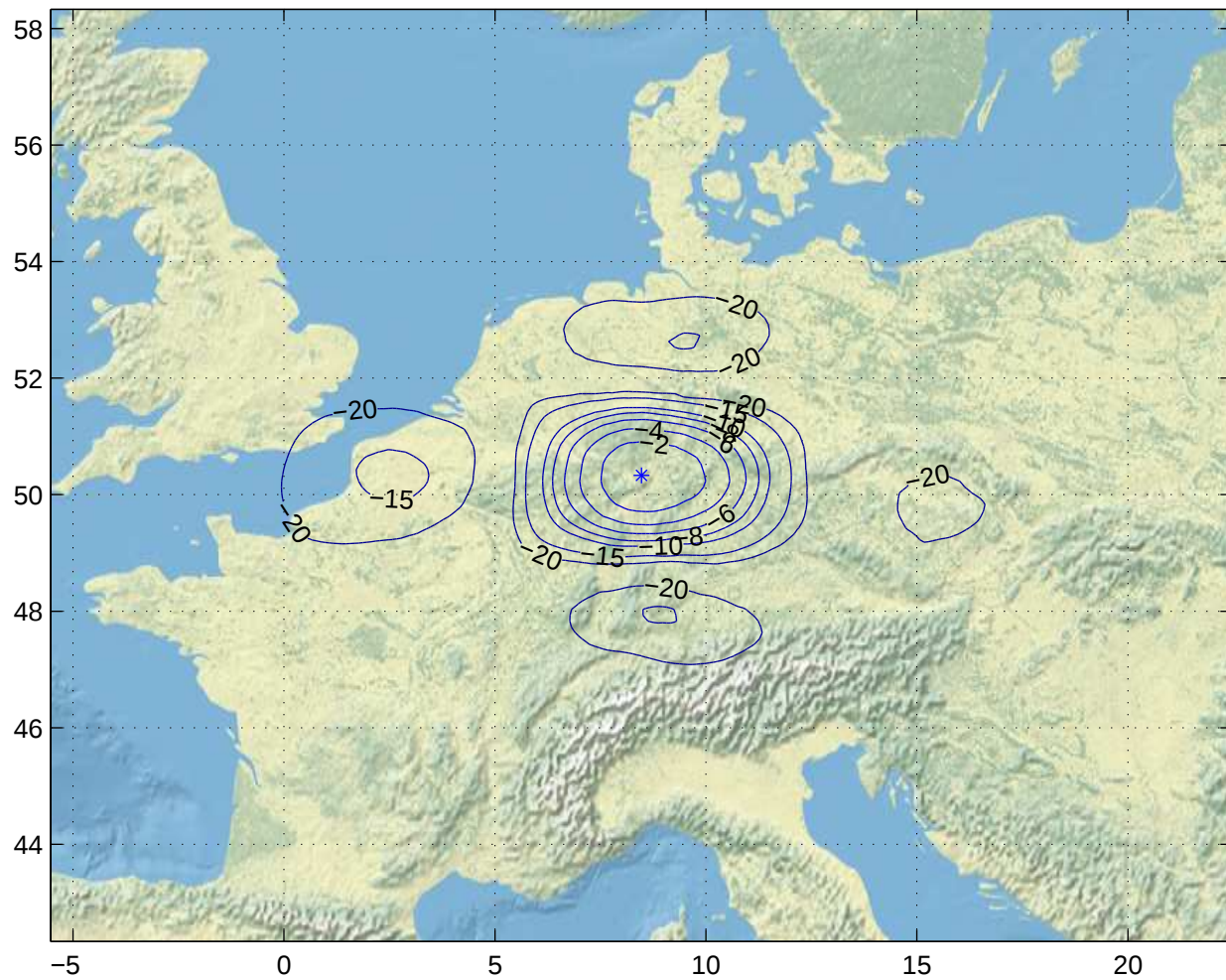
Gain Contours at 575km for FRA. Beam ID=XTC, Polarization=rhcp
