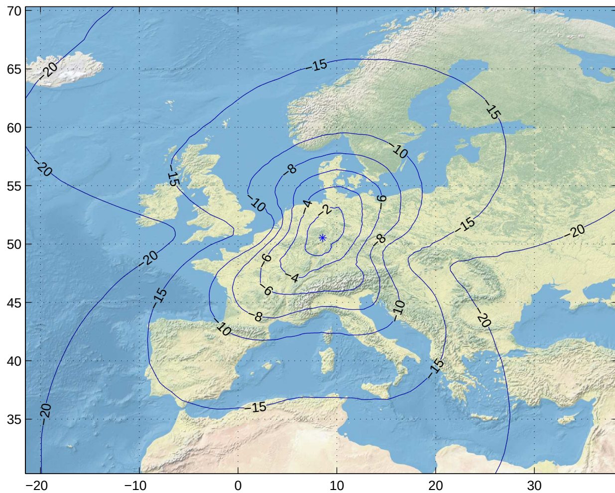
Gain Contours at 460km for FRA. Beam ID=SRX, Polarization=lhcp
