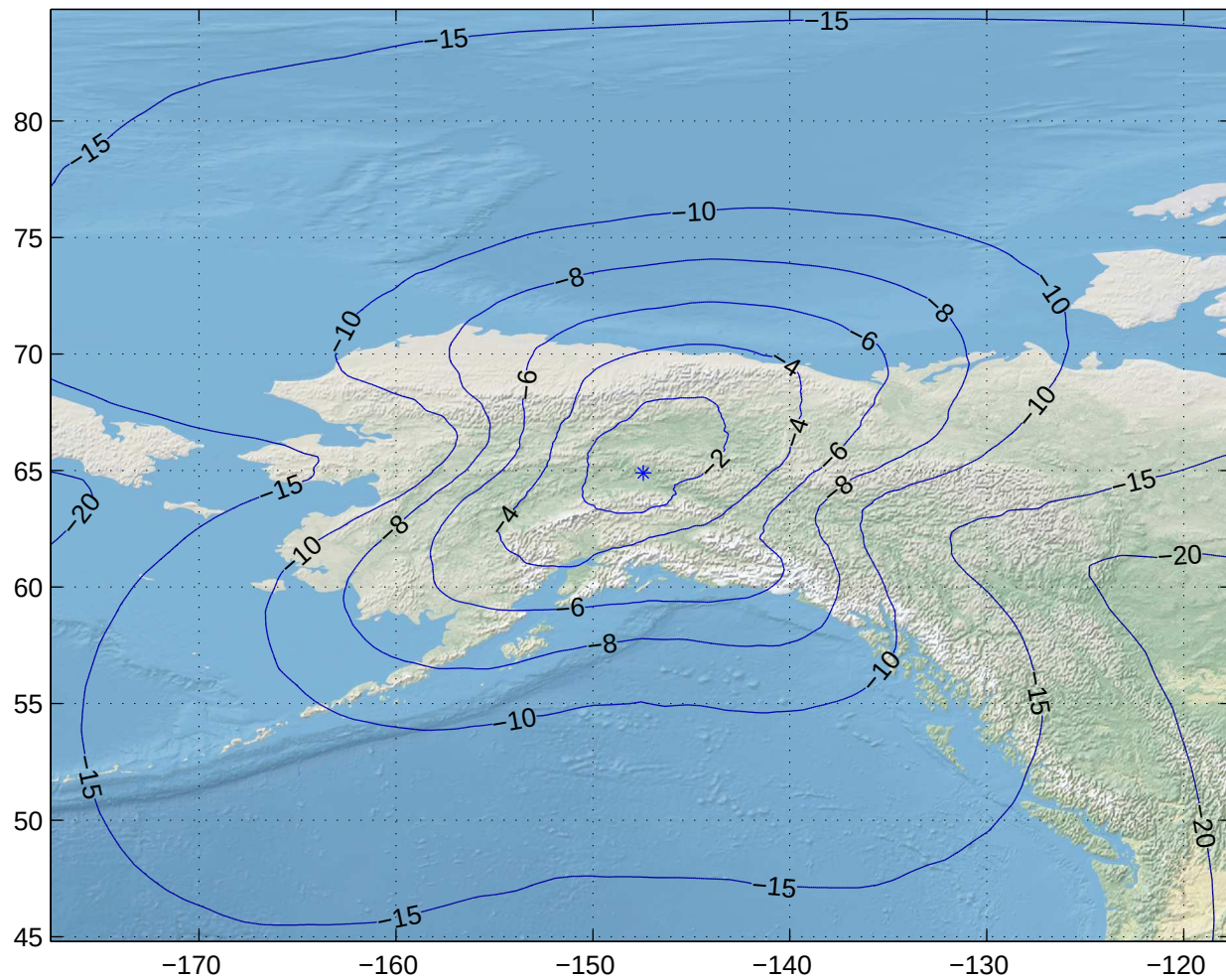
Gain Contours at 575km for FAI. Beam ID=SRX, Polarization=lhcp
