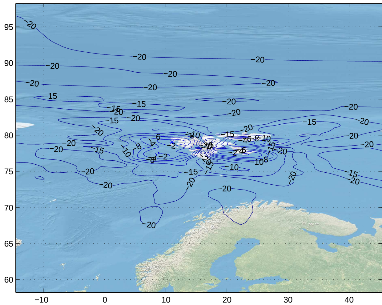
Gain Contours at 460km for LYR. Beam ID=XTX, Polarization=lhcp
