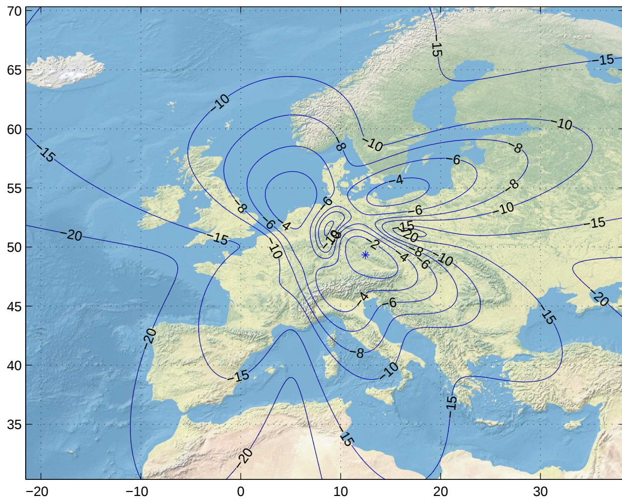
Gain Contours at 475km for FRA. Beam ID=URX, Polarization=rhcp
