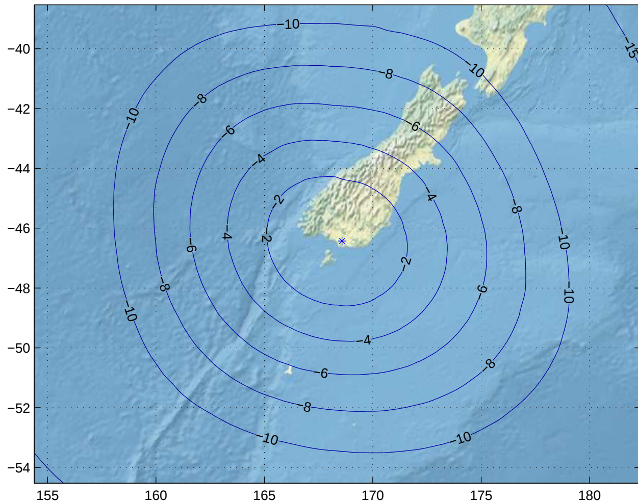
Gain Contours at 505km for IVC. Beam ID=SRC, Polarization=rhcp
