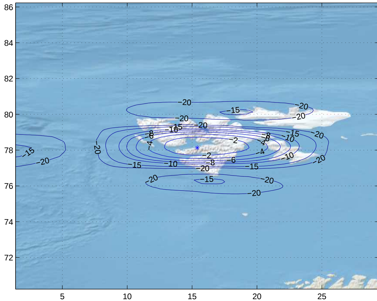
Gain Contours at 475km for LYR. Beam ID=XTC, Polarization=rhcp
