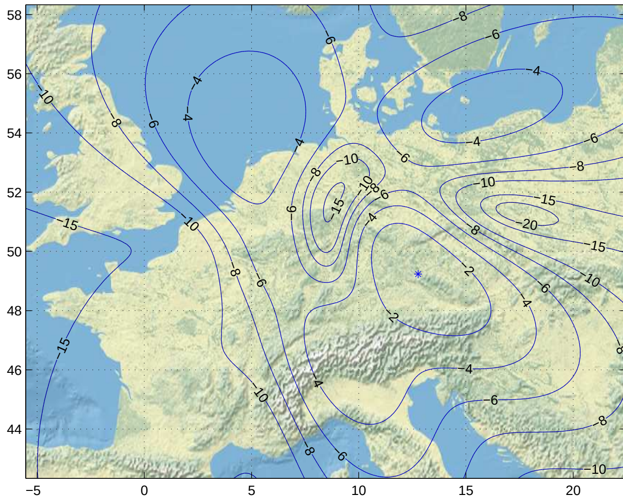
Gain Contours at 505km for FRA. Beam ID=URC, Polarization=h
