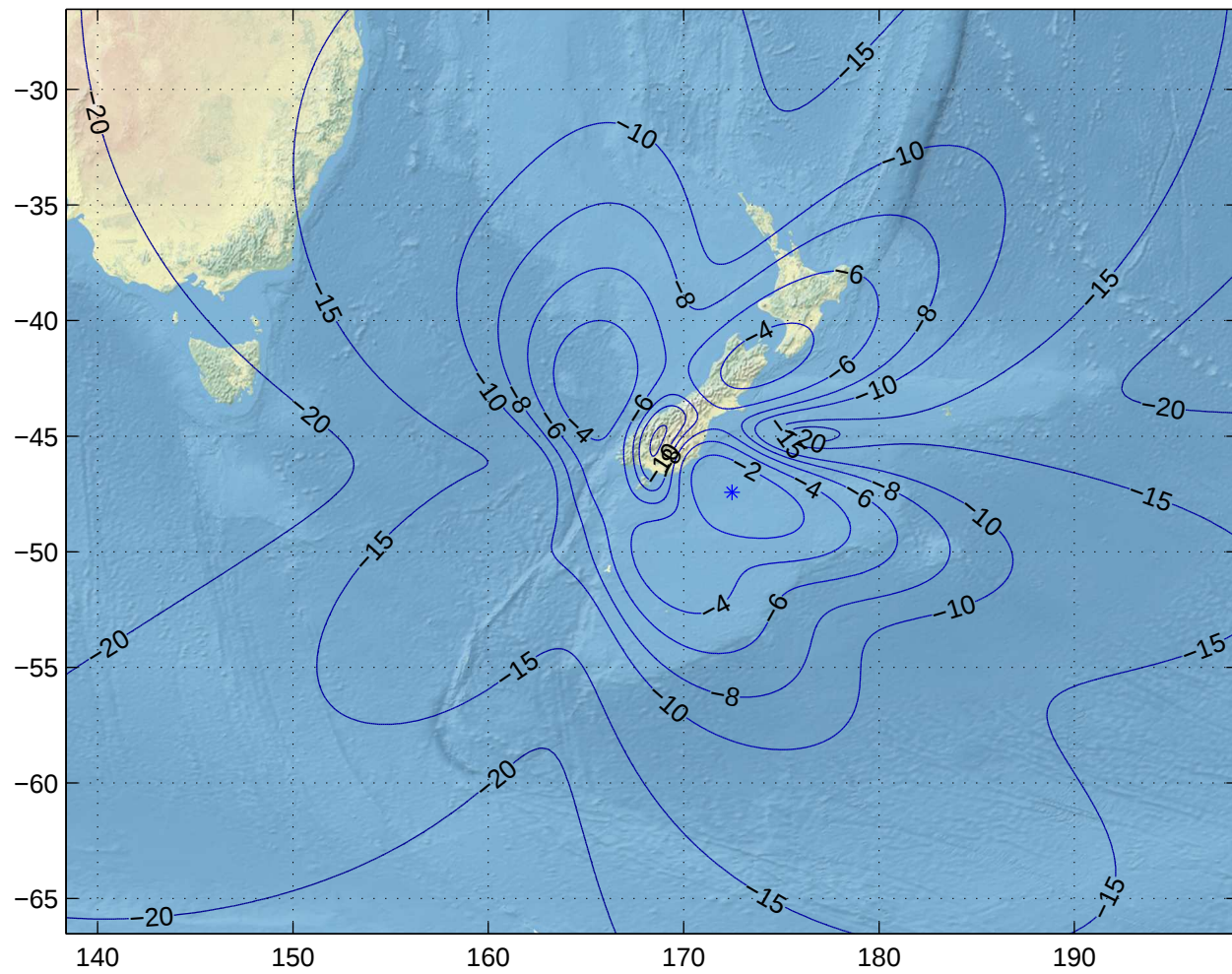
Gain Contours at 505km for IVC. Beam ID=URX, Polarization=rhcp
