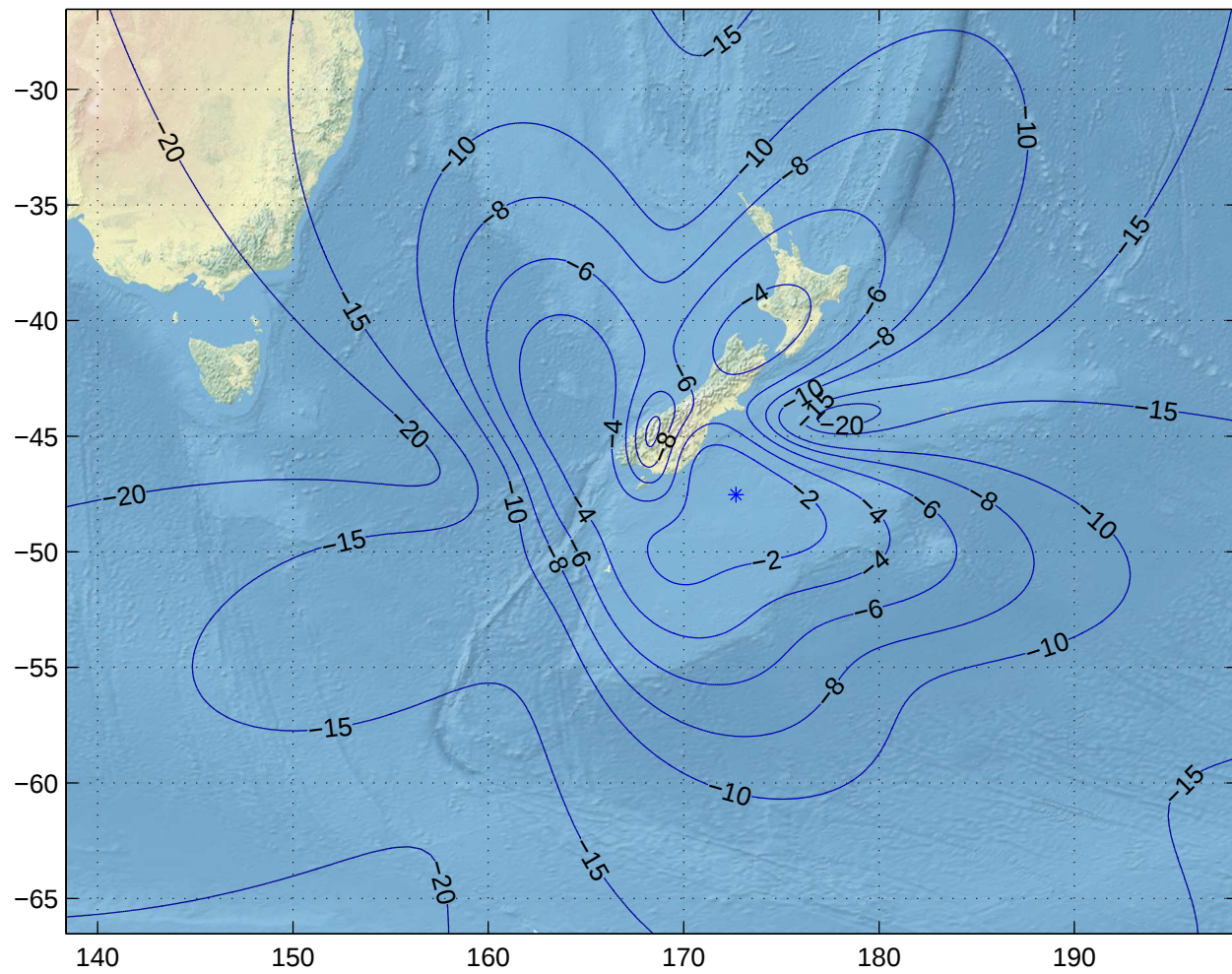
Gain Contours at 575km for IVC. Beam ID=UTX, Polarization=rhcp
