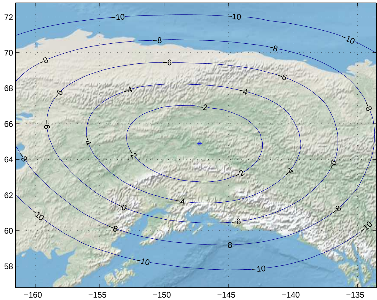
Gain Contours at 505km for FAI. Beam ID=SRC, Polarization=rhcp
