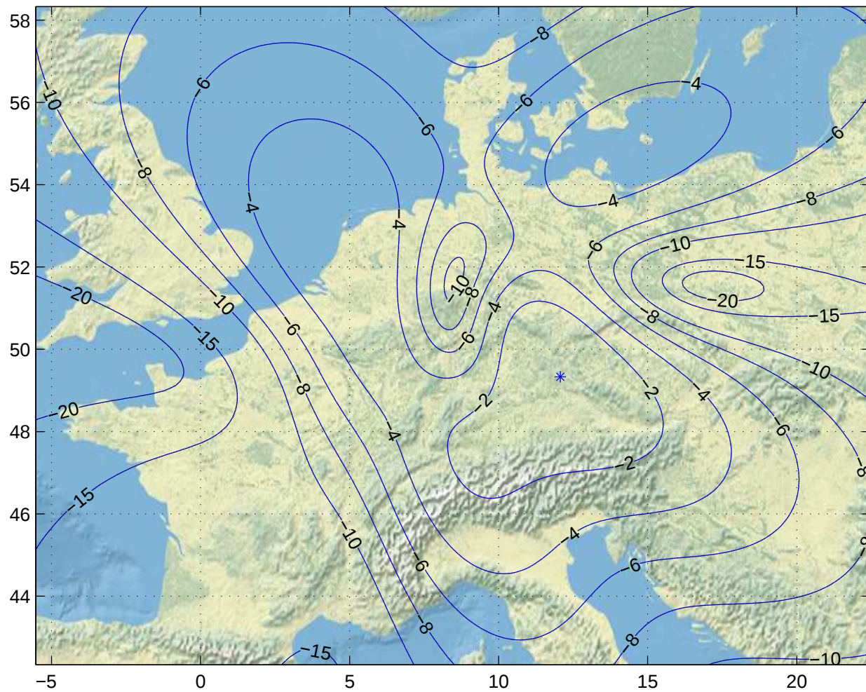
Gain Contours at 460km for FRA. Beam ID=UTC, Polarization=h
