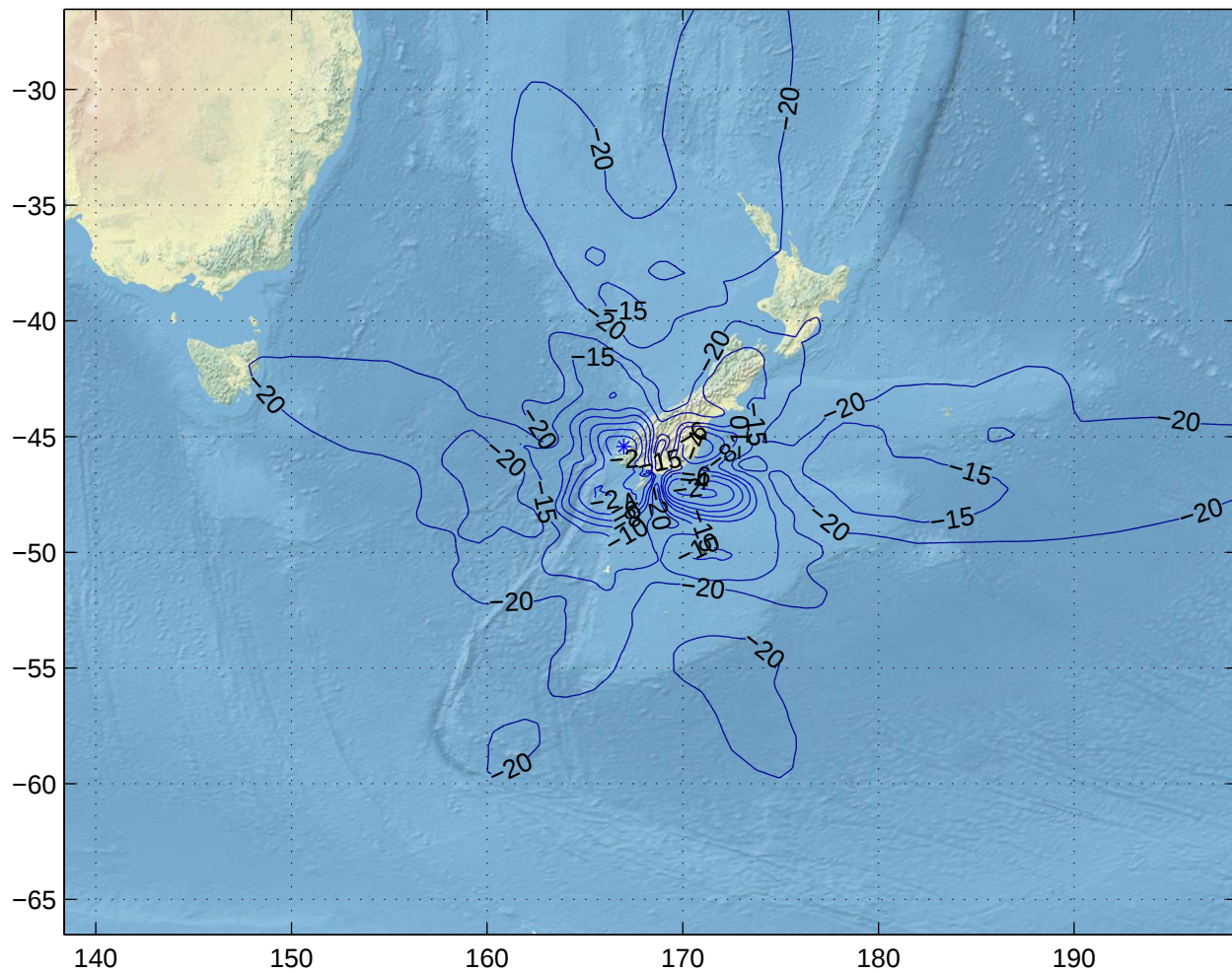
Gain Contours at 575km for IVC. Beam ID=XTX, Polarization=lhcp
