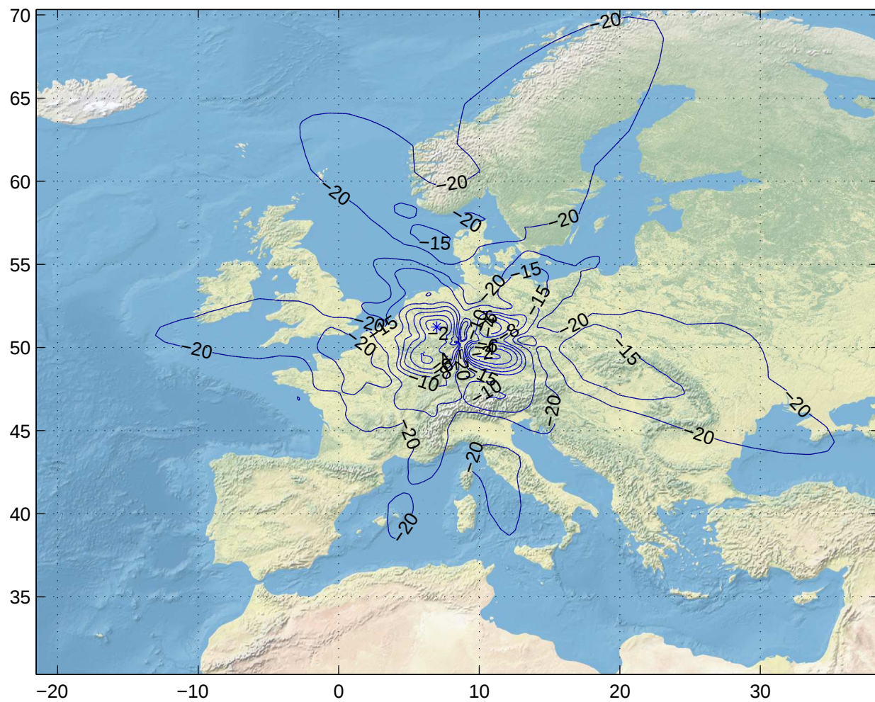
Gain Contours at 505km for FRA. Beam ID=XTX, Polarization=lhcp
