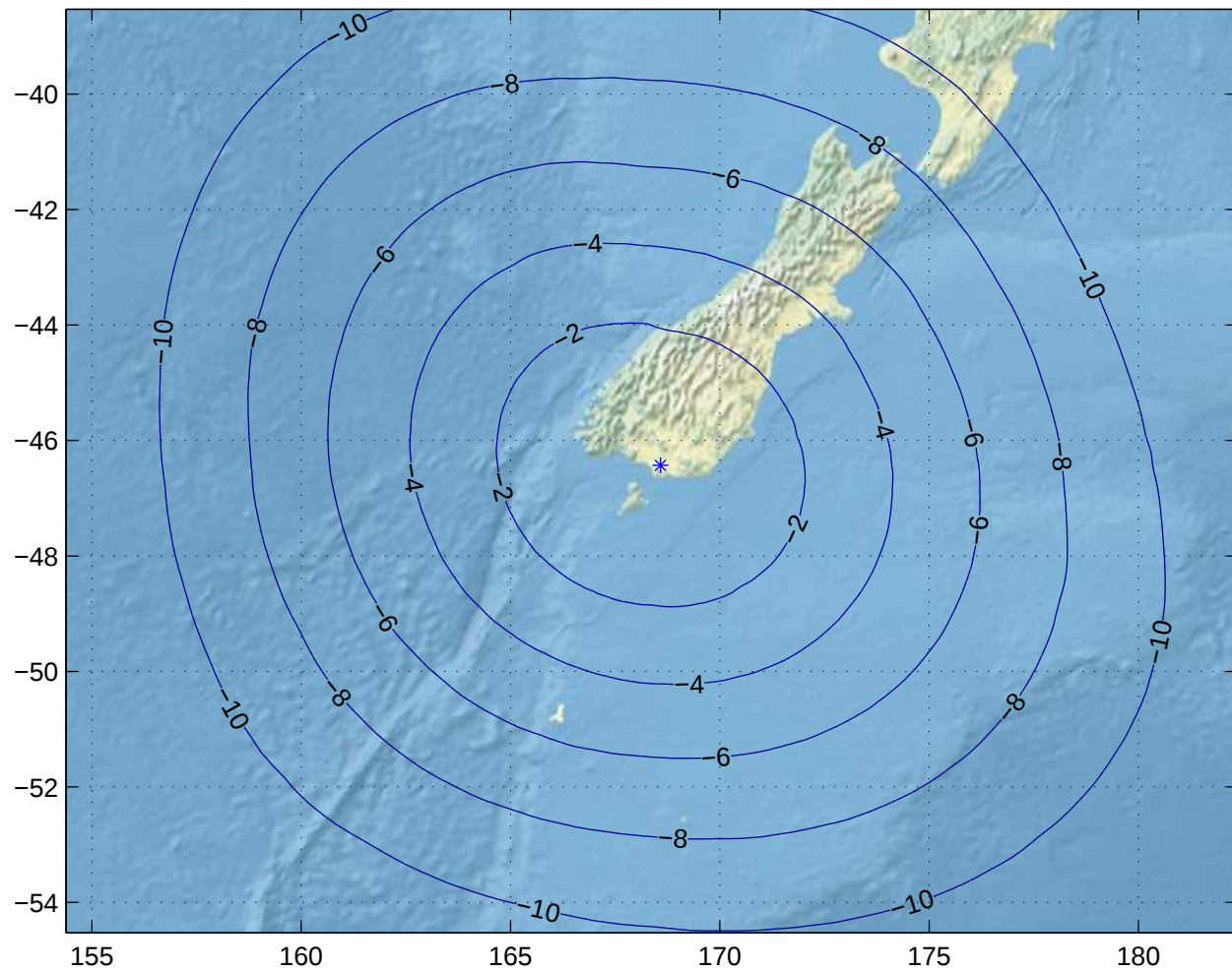
Gain Contours at 575km for IVC. Beam ID=SRC, Polarization=rhcp
