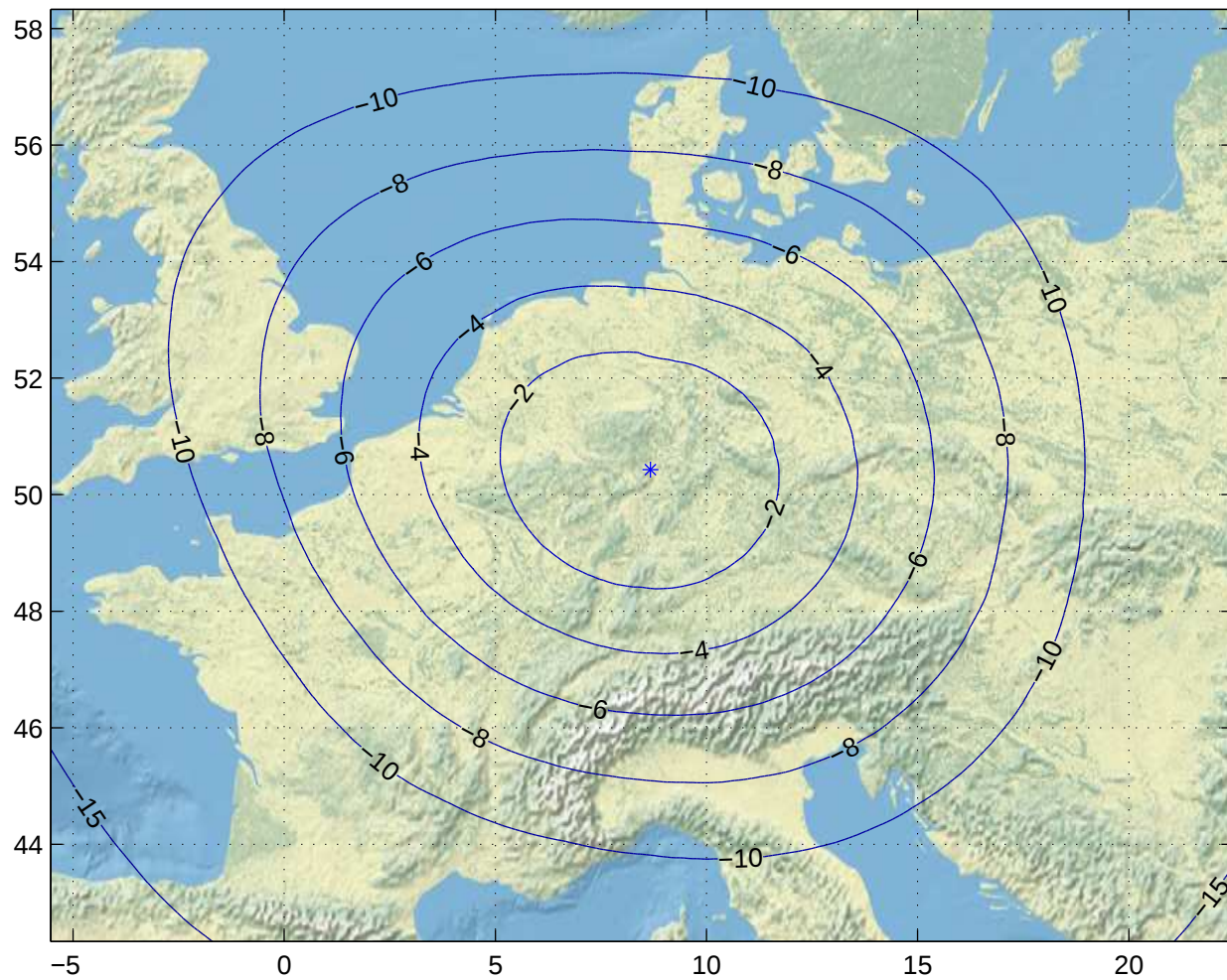
Gain Contours at 475km for FRA. Beam ID=SRC, Polarization=rhcp
