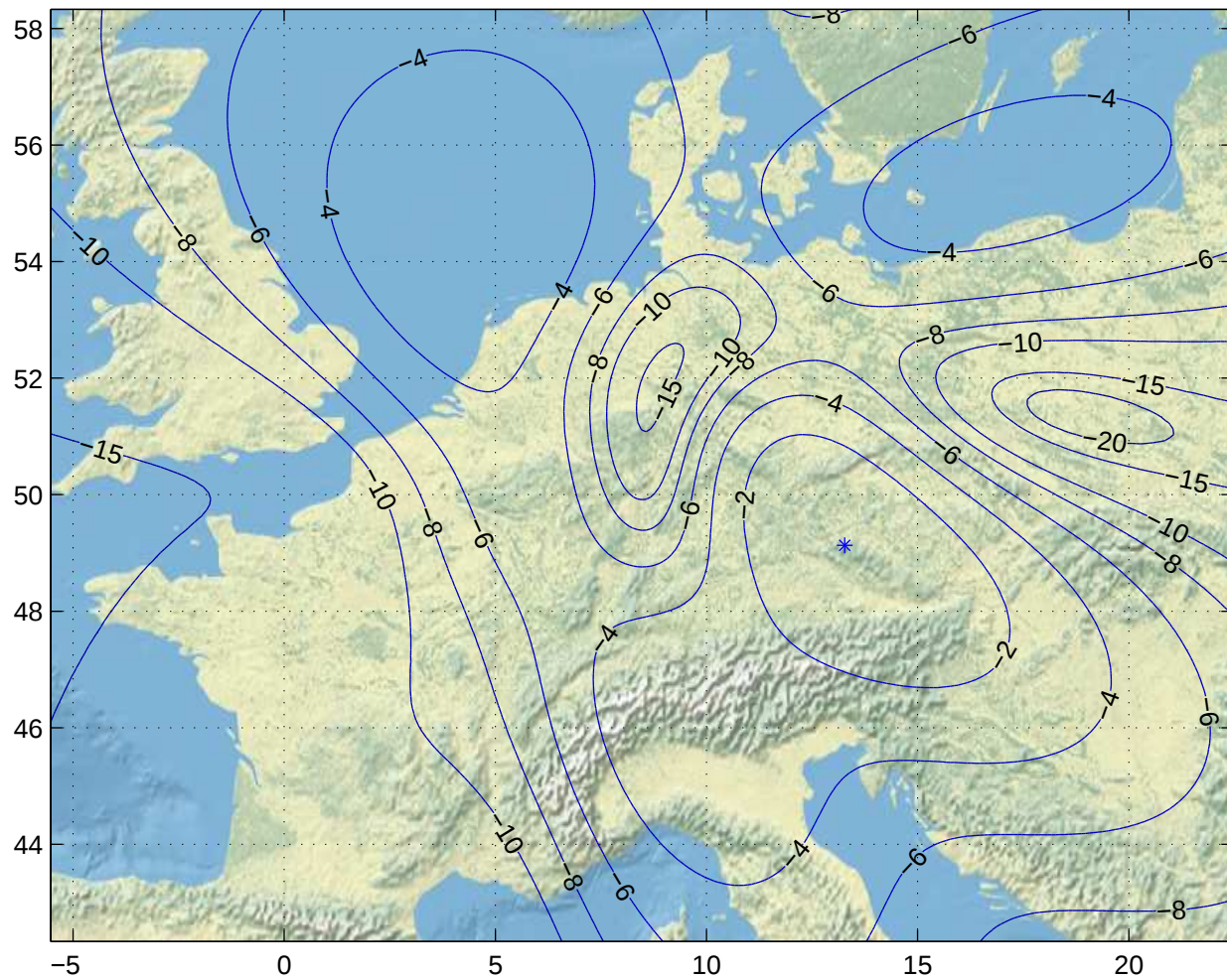
Gain Contours at 575km for FRA. Beam ID=URC, Polarization=h
