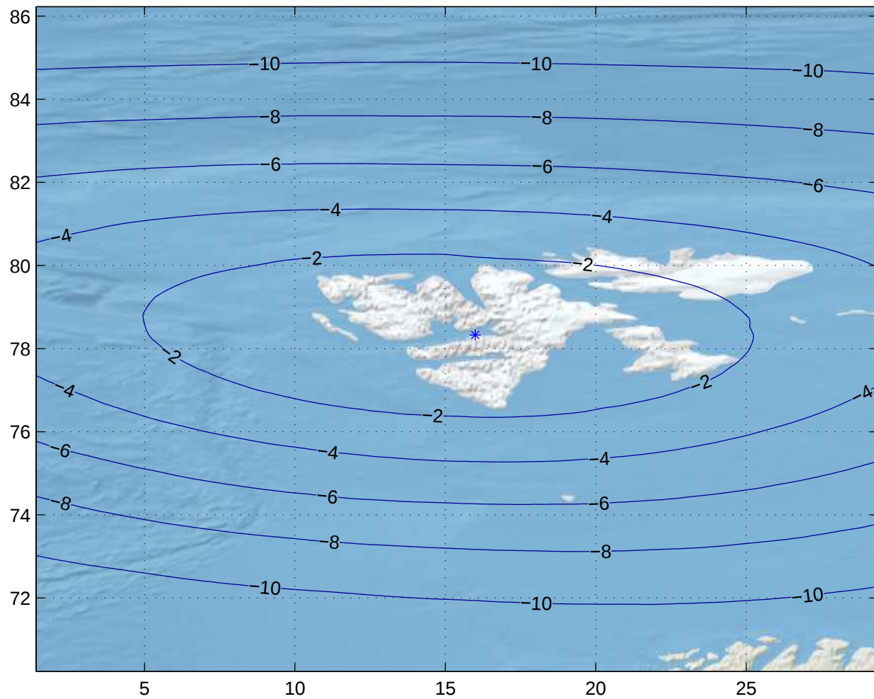
Gain Contours at 460km for LYR. Beam ID=SRC, Polarization=rhcp
