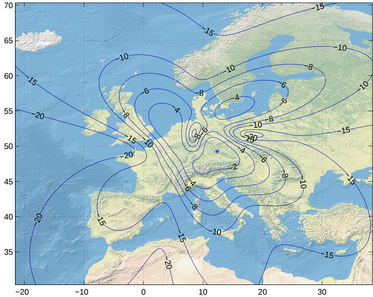
Gain Contours at 505km for FRA. Beam ID=UTX, Polarization=rhcp
