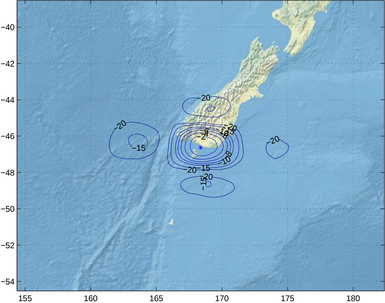
Gain Contours at 505km for IVC. Beam ID=XTC, Polarization=rhcp
